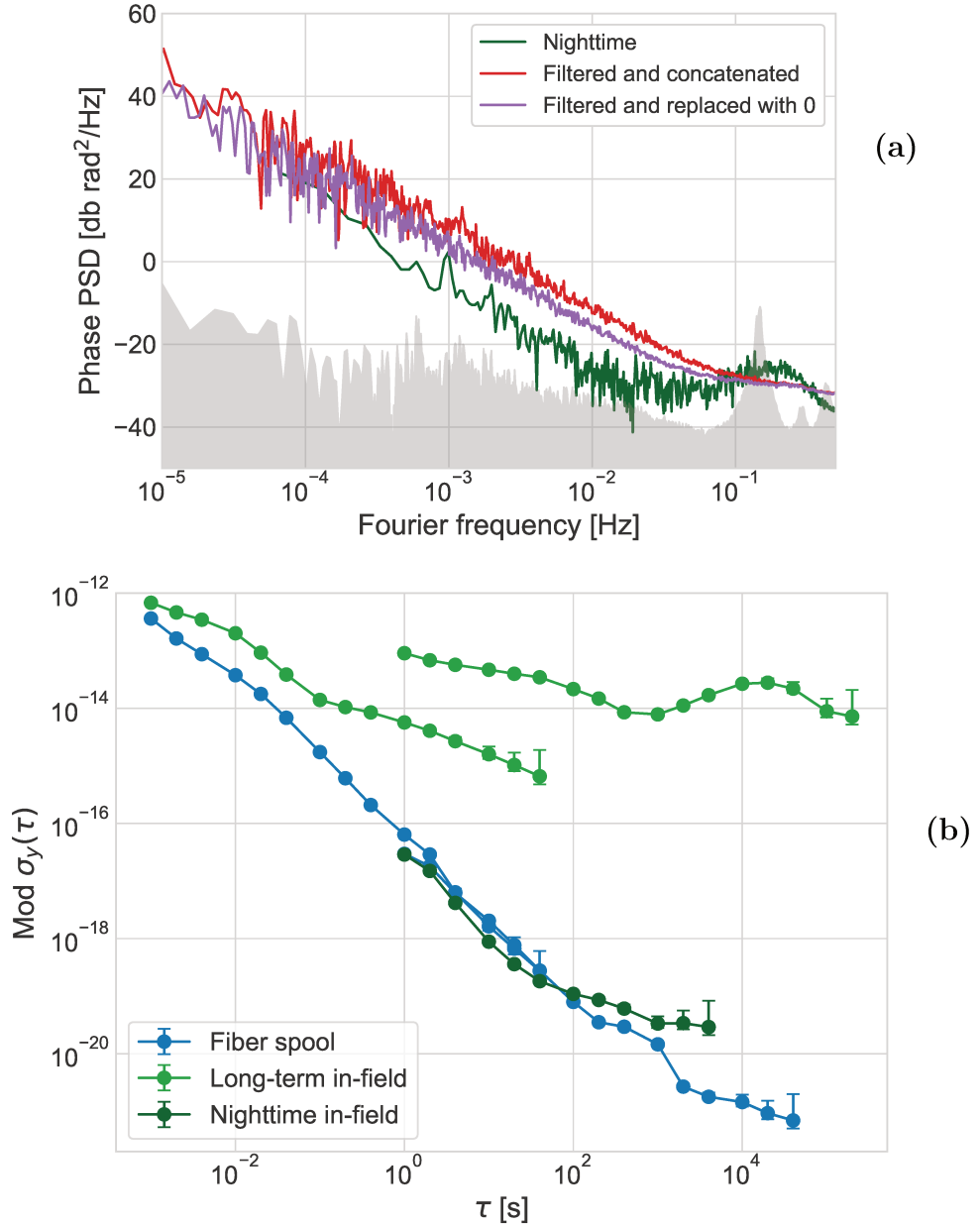
FIGURE B.1: (a): Phase power spectral density (PSD) of the of the in-filed configuration during nighttime (green), filtered long-term where data is concatenated (red), and filtered long-term where the phase is kept constant across the gap left by the missing data (purple). (b): modified Allan deviation (MDEV) of the long-term in-field configuration (light green), nighttime in-field (dark green), and fiber spool configuration (blue).
