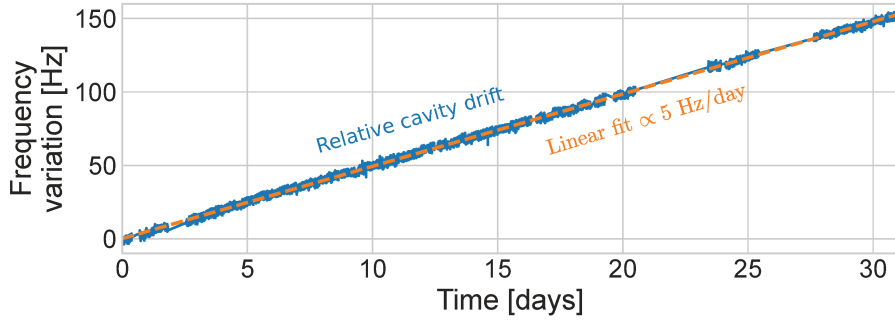
FIGURE 5.5: Variation of the two-way comparison between the ultra-stable cavities as SYRTE and PTB, for the duration of 1 month. Orange dotted line shows a linear fit, with a relative drift of 5 Hz/day.
