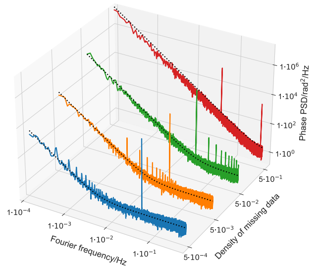
Figure 8. Phase noise PSD of a carrier signal with white phase noise for 4 different densities of periodically missing data. Both the aliasing due to the Dick effect and due to the sampling of the modulation are clearly seen. The black dotted lines represent equation (6).
