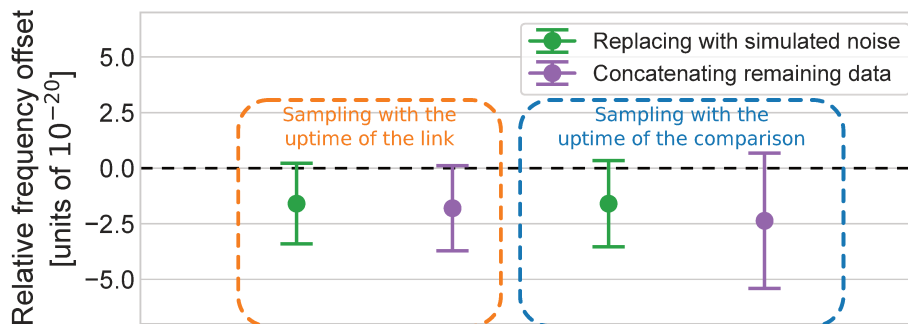
FIGURE 5.19: Uncertainty contribution of the optical fiber link to the cavity comparison, over the one month of comparison campaign when: sampled by the uptime of the link itself (orange box), and when sampled by the full cavity comparison (blue box). Evaluations are made in the two following cases: using a concatenation of the remaining data (purple) and replacing the missing data with simulated noise (green).
