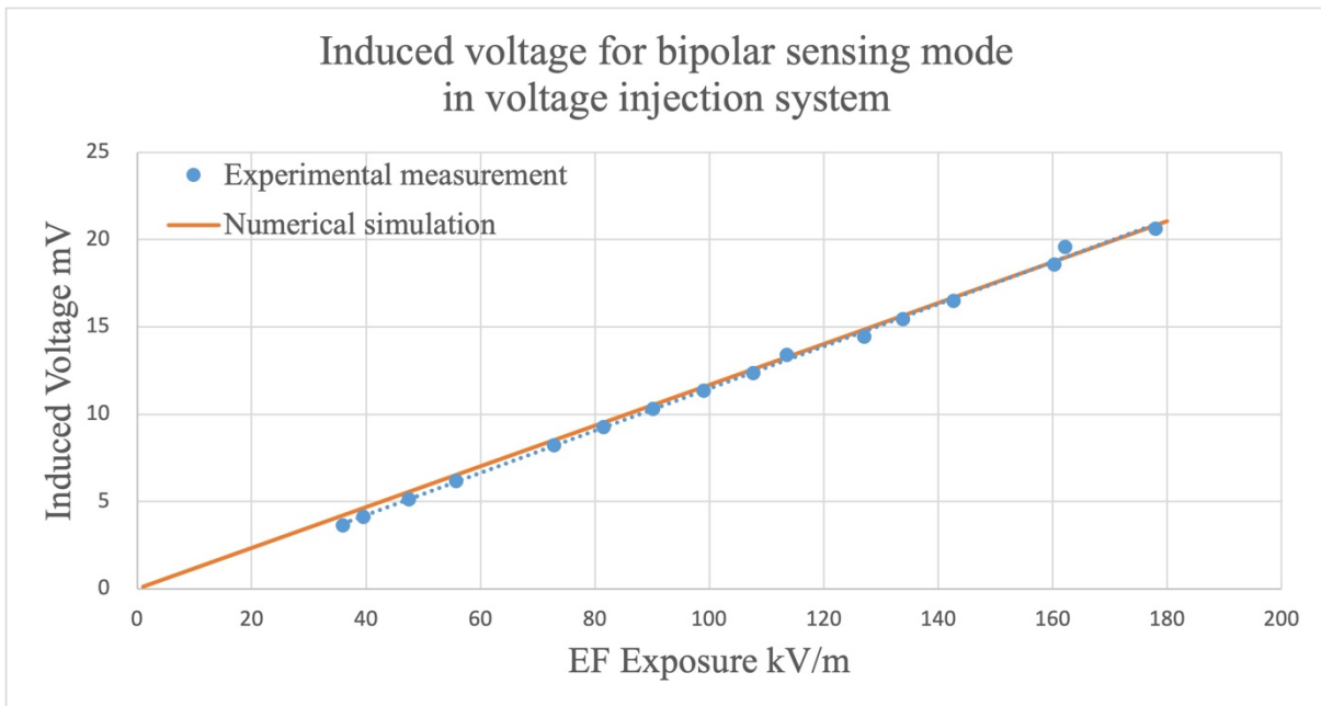
Figure 3-27 Measurement results for bipolar sensing mode in voltage injection system
