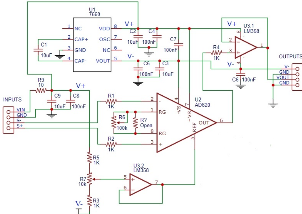
Figure 3-12 Circuit B: AD620 instrumentation amplifier module
