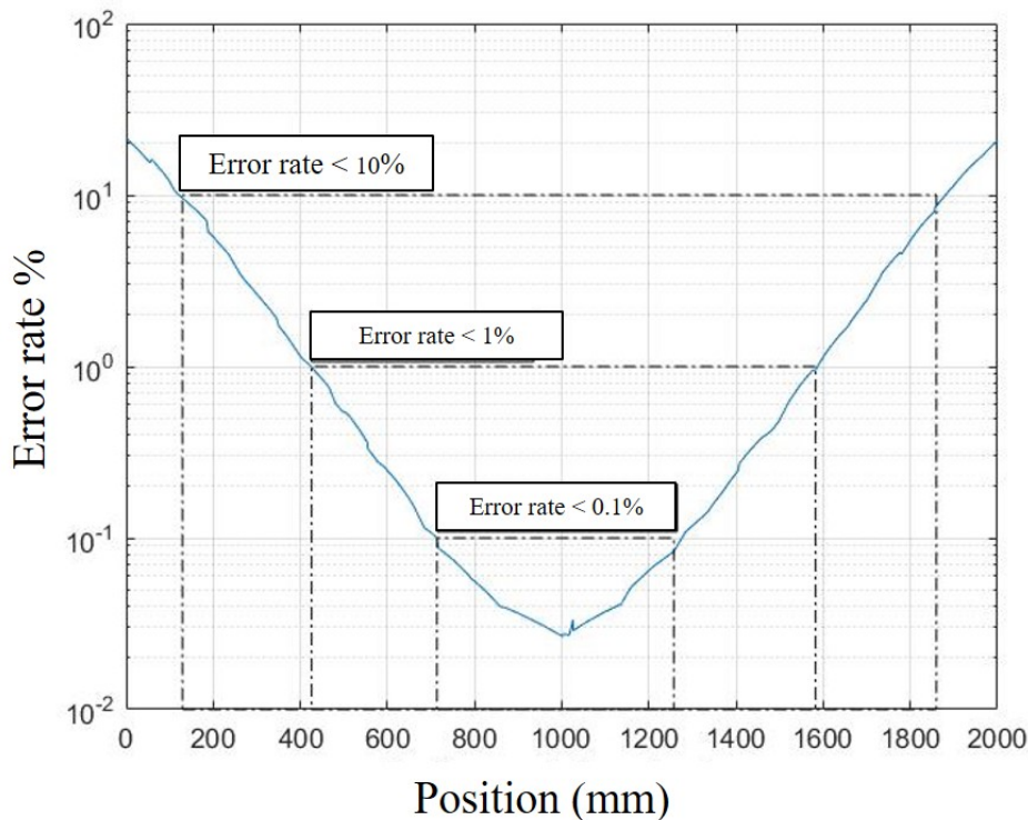
Figure 2-15 Error rate of the generated EF on the horizontal central line
