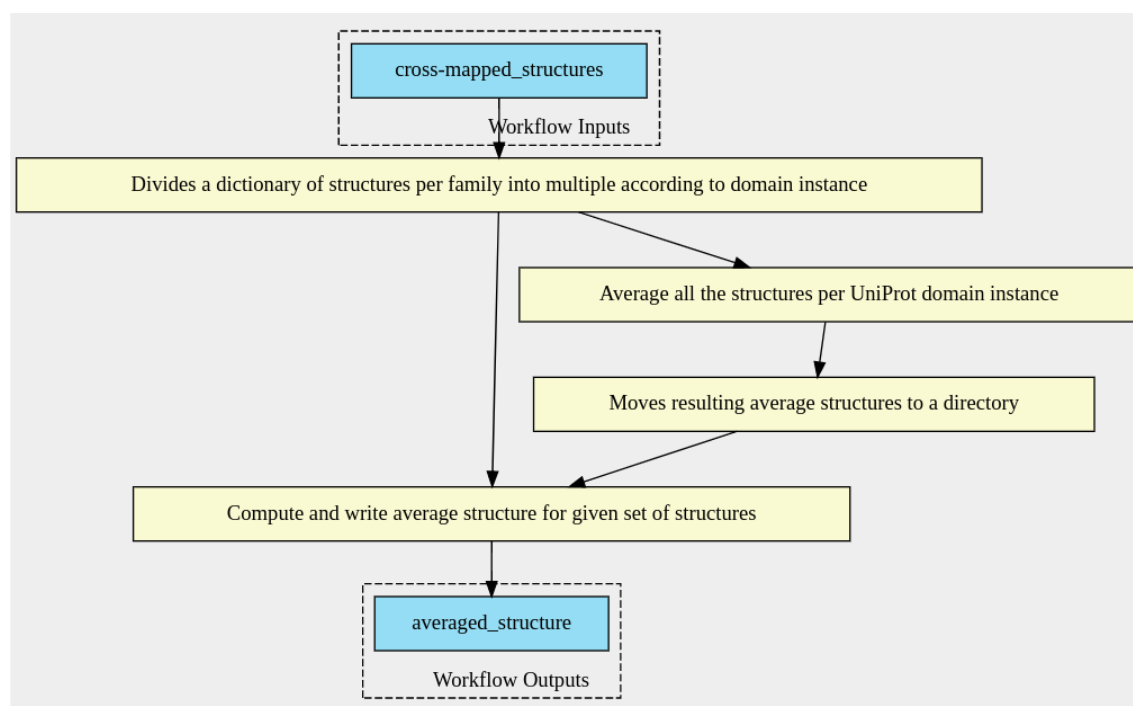
Figure 4.4: Steps to compute family-level average structure as the average of instance-level average structures (Figure was generated locally using cwltool).
