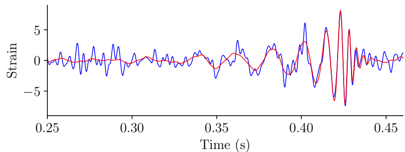
Figure 2.10: Whitened observations (blue) and matched filter template (red) of GW150914 for LIGO Hanford detector.
