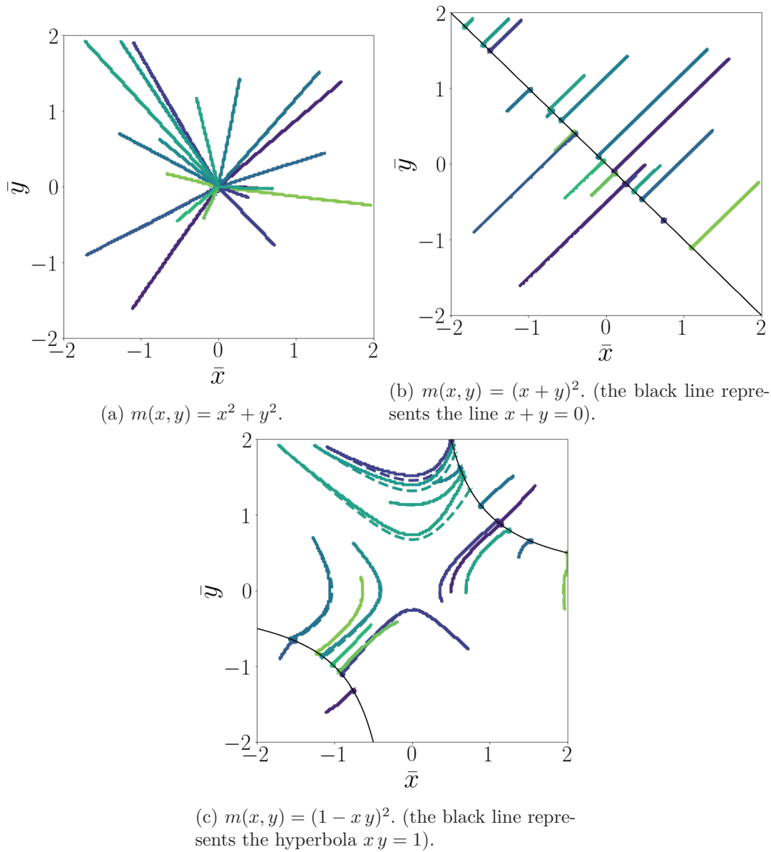
Figure 6.3: Simulated trajectories of the dominant alleles \bar{x} and \bar{y} . The plain lines correspond to the trajectories of (x^{\max}(t), y^{\max}(t)) that realizes the maximum of n_\varepsilon(t, \cdot, \cdot) in the numerical resolution of (P(n_\varepsilon)) , with \varepsilon = 0.01 . The dashed lines correspond to the numerical resolution of the canonical equations given in 6.2.2. Each color corresponds to one trajectory starting at an initial monomorphic state chosen randomly and uniformly in [-2, 2]^2 . The final states of the trajectories obtained from the discretization of (P(n_\varepsilon)) are indicated by full circles. This figure shows that the qualitative derivation of the section are numerically consistent with the model.
