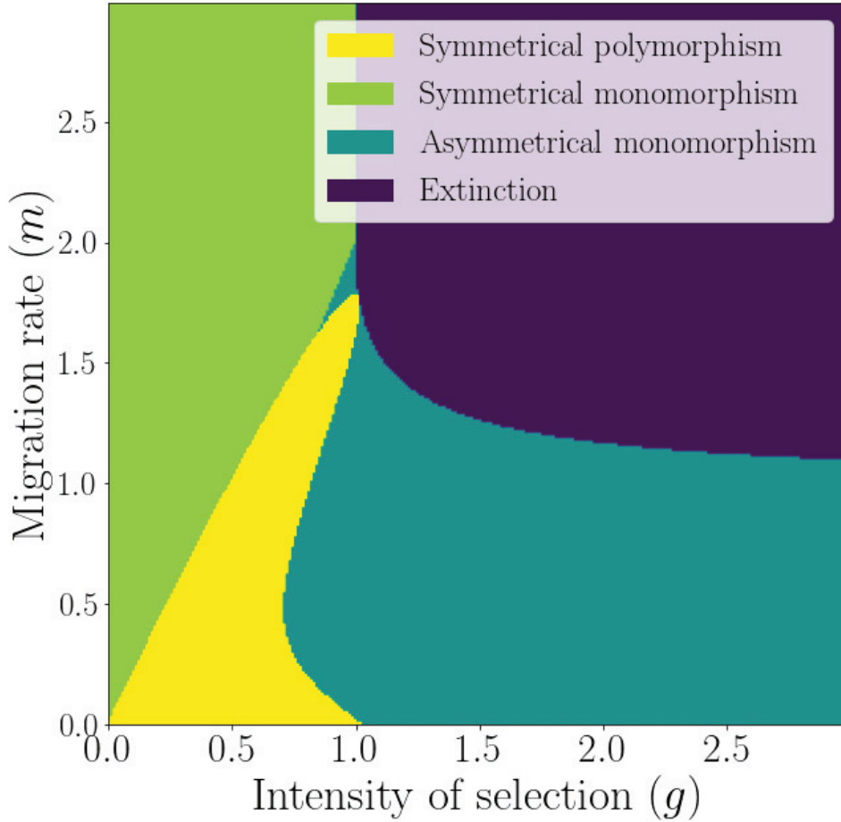
Figure 4.6: Summary of the complete analytical outcomes of the model , for \eta = 0.5 and varying migration ( y -axis) and selection ( x -axis). The figure combines the results obtained in Section 4.3.1 on the stability of the symmetrical polymorphic equilibrium with the results of the model of Dekens [2022] (equivalent to this model upon loss of polymorphism). For bounded selection, when migration increases, there is a threshold over which the polymorphism at the major-effect locus is lost due to the blending effect of migration (consistent with Yeaman and Whitlock 2011). The population then becomes equally maladapted to both habitats (generalist - symmetrical monomorphism, in the green region). For this specific major-effect allelic effect \eta = 0.5 , there exists additionally an interval of selection strength ( \approx [0.7, 1] ) for which the major polymorphism might not be stable at all migration rates below the critical threshold. This phenomenon does not seem to hold when the major effect is larger (see Fig. 4.3b). For bounded migration (below the threshold rate over which the strong migration blending hampers the major polymorphism), when selection strength increases, the polymorphism at the major-effect locus (yellow region) is lost, and the population becomes adapted to one of the two habitats (specialist - asymmetrical monomorphism, in the blue region). As this figure is obtained in the small segregational variance regime (which should remain smaller than the other parameters of the system for the analysis to be valid), we warn that the outcomes displayed in the vicinity of the x -axis (very small migration rates) might not correspond to the limit when the migration rate is 0 (no migration).
