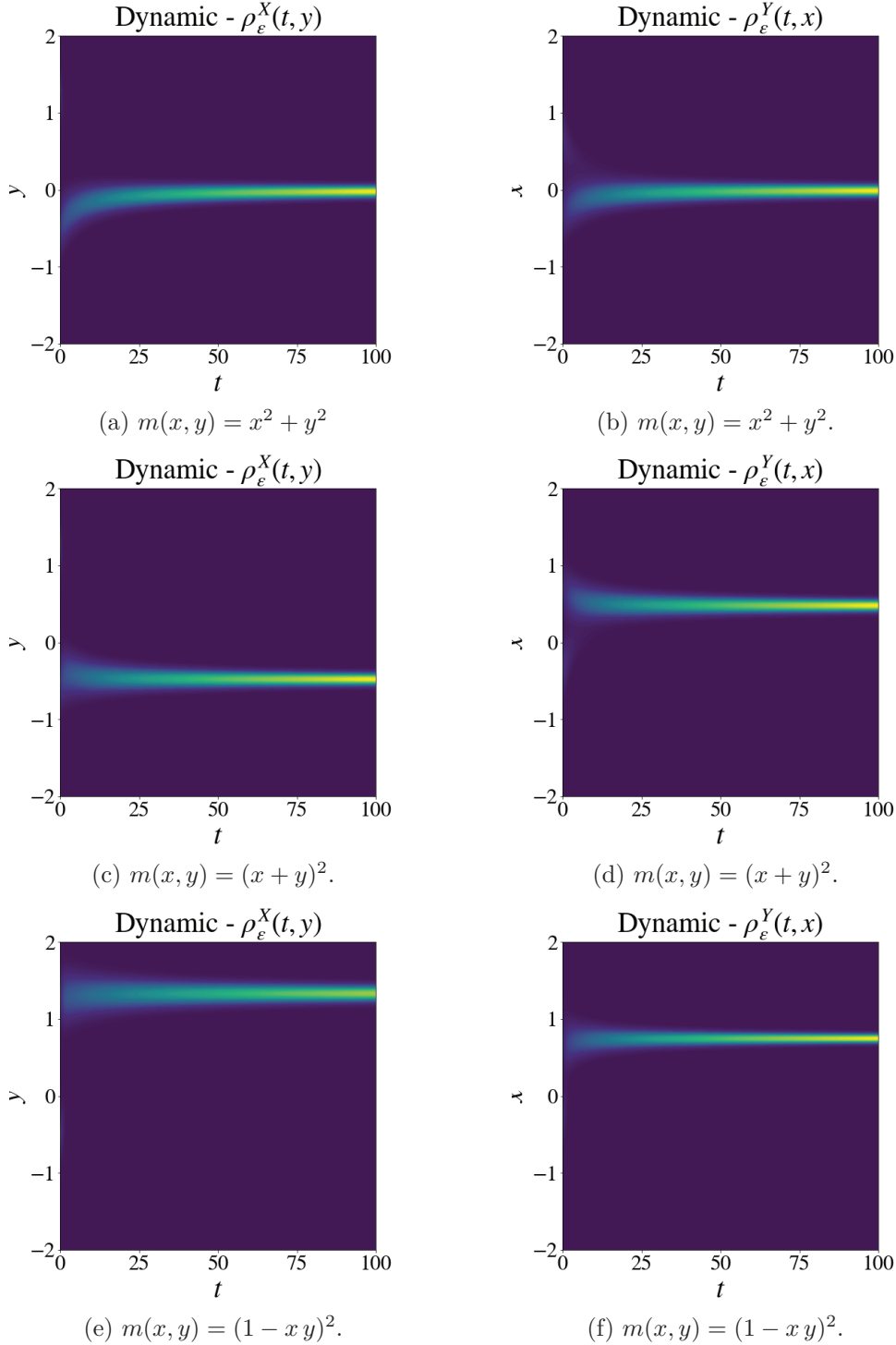
Figure 6.2: Robustness of monomorphism with regard to assumption H_{\text{increasing}} of 6.2.2 with dimorphic initial densities. For each selection function (by row), we display the numerically solved dynamics of \rho^X(t, y) (left panel) and \rho^Y(t, x) (right panel) ( (x, y) \in [-2, 2] ). The colors correspond to isolines of \rho^X and \rho^Y . The initial state is sum of two Gaussians centered in (x_1, y_1) = (-0.3, 1.3) and (x_2, y_2) = (0.7, -0.5) and of variance \epsilon = 0.05 . Lighter colors indicate stronger densities. The figures seem to indicate that the trajectories become monomorphic almost instantaneously and that this phenomenon actually occur under weaker conditions than H_{\text{increasing}} of 6.2.2. One can also notice that the stationary dominant alleles that arise vary greatly from one selection function to another.
