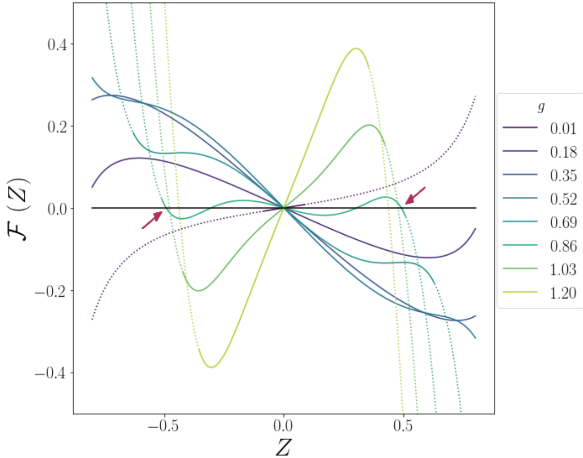
Figure 4.4: Phase lines of the limit equation (4.19), when the migration rate and the strong allelic effect are held constant ( m = 0.1, \eta = \frac{1}{2} ) and the selection strength varies (the lighter the color, the stronger the selection). Solid curves indicate that the system is polymorphic, whereas dashed curves indicate that one major-effect allele has fixed. Every intersection of the horizontal black line and a solid colored curve with a negative (resp. positive) slope indicates a locally stable (resp. unstable) polymorphic equilibrium. The darker curve with weak selection g = 0.01 has a positive slope at Z = 0 (unstable), the following curves have a negative slope at Z = 0 (stable for selection between g = 0.18 and g = 0.86 ), and finally the lightest curves have a positive slope at Z = 0 (unstable for g \geq 1.03 ), which is consistent with Fig. 4.3a. Note that there exists additionally two mirrored asymmetrical polymorphic equilibria for g = 0.86 , for Z \approx \pm 0.5 (indicated by the red arrows), which were unsuspected prior to this numerical analysis.
