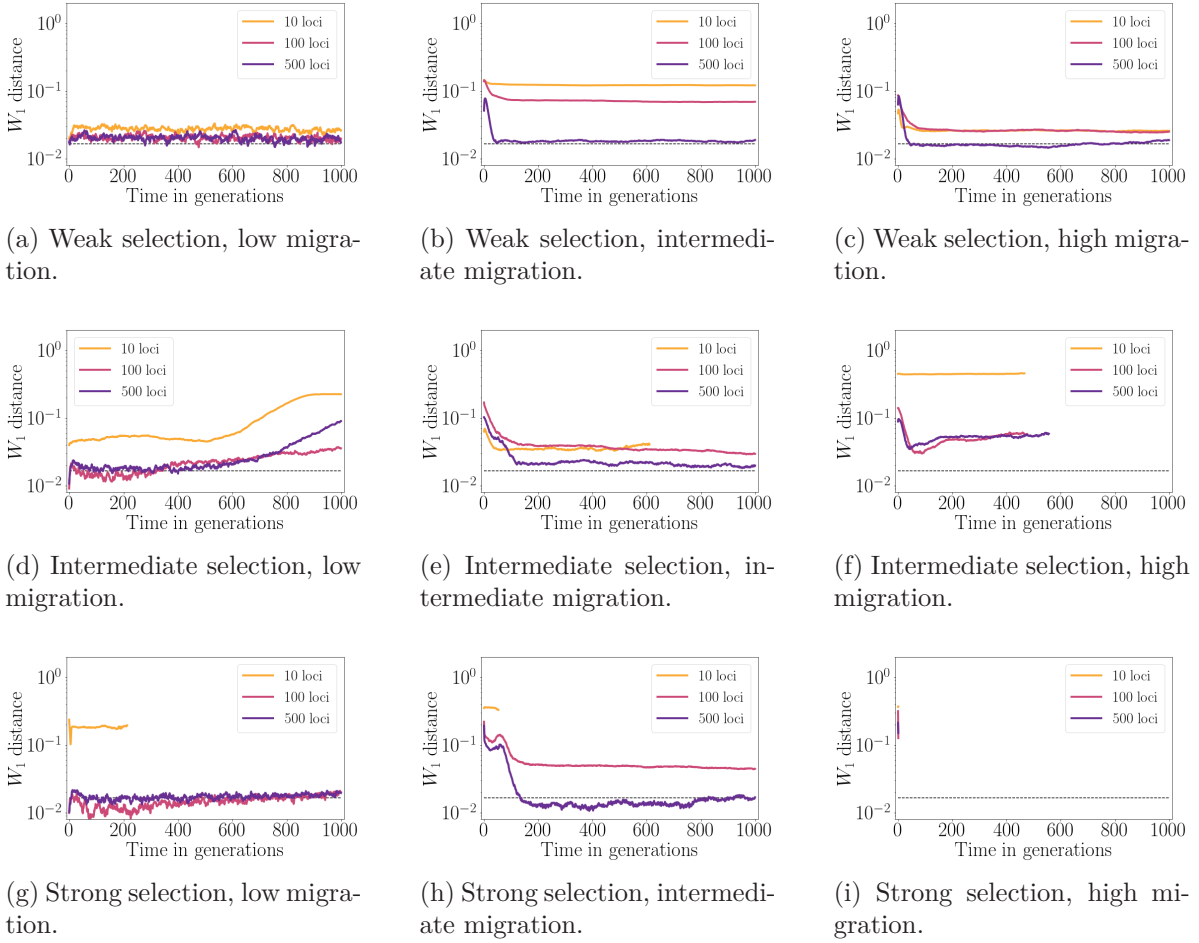
Figure 3.2: Dynamics of the W_1 distance between the distributions of the IBS replicates according to (3.8) and the solutions of the deterministic discrete-time model (3.2), for 3 increasing levels of selection (rows, top to bottom 0.1, 1, 2) and 3 increasing levels of migration (columns, left to right 0.05, 0.8, 1.4), with a small standard deviation at linkage equilibrium \sigma_{LE} = 0.1 (small variance case). For each figure, the three colors correspond to three different number of loci L = \{10, 100, 500\} (darker colors for larger number of alleles). The coloured lines represent the median distance across replicates (interrupted lines means that extinction occurred). The black dashed line represents the distance between two Dirac masses on consecutive points of the trait space's grid Z . Other parameter values for the deterministic models are: r = 1, \kappa = 1, \Delta t = 0.1 and those for the IBS as indicated in Section 3.3. Here, the number of loci matters substantially. With 500 loci, the distances between the IBS and deterministic trajectories (purple lines) are almost always equivalent to the minimum distance between two Dirac masses on the discretization grid (dashed horizontal line), with indicates excellent agreement, at the exception of extinction events (Fig. 3.2f, Fig. 3.2i). With 100 loci, which is the limit case where the phenotypic range matches the difference between local optima, the agreement with the deterministic model is similar than with 500 loci when migration is low (left column), but degrades when migration becomes higher (middle and right column). With 10 loci, additional extinctions occur when selection is strong and migration is low (Fig. 3.2g) or intermediate (Fig. 3.2h), and at intermediate selection-migration (Fig. 3.2e), which is consistent with Fig. 3.1d. Notice that in Fig. 3.2d, the distance increases slightly after 600 generation for all number of loci. This comes from the fact that the outcomes at this particular migration-selection parameters are near the border of two qualitatively different phenomena (asymmetrical monomorphic or dimorphic - see Fig. 3.1a.)
