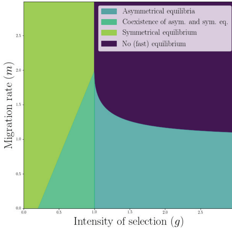
Figure 2.4: Regions of existence of the equilibria, according to 2.5.1 and 2.5.2. The symmetrical equilibrium is only determined by the intensity of selection, regardless of the migration rate. The asymmetrical equilibria cannot exist for large migration rate ( m > 2 ) or small intensity of selection. The limit of the blue region is given by m = 1 when g goes to \infty . Interestingly enough, at intermediate migration: m \in [1, 2] , asymmetrical equilibria only exist for a bounded range of positive g : selection cannot be too strong nor too weak. Moreover, see Section 2.5.2 for stability results about these equilibria to determine which equilibria prevail when both symmetrical and asymmetrical coexist (turquoise triangular region).
