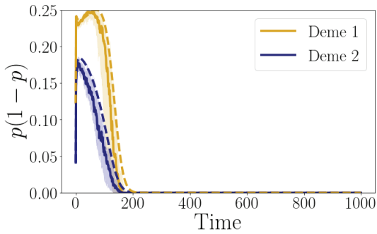
(e) Major-effect locus with polygenic background: strong selection ( g = 1 ).
