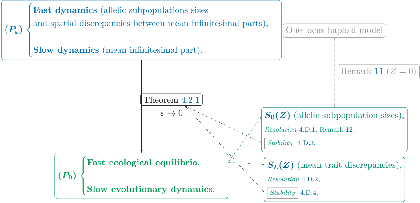
Figure 4.7: Layout of the slow-fast analysis in Section 4.D. This figure presents the key elements of the separation of time scales leading from P_\varepsilon to P_0 . The stability of the fast equilibria (studied in the two subsystems S_0(Z) and S_L(Z) ) is the crucial argument underlying the convergence result stated in Theorem 4.2.1. The resolution of S_0(Z) leads to a uniqueness result that is unexpected with regard to the analogous resolution in Dekens [2022] (see Remark 12).
