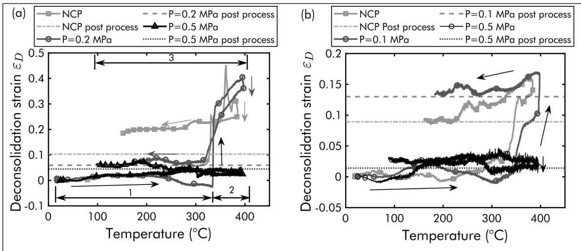
Figure 7.15: Through thickness deconsolidation strain \epsilon_D at the center of a wet AS (a) and dried DS-72H@180C (b) UD-HP samples subjected to different counter pressure vs temperature (sample lower face temperature estimated with the thermal model).
