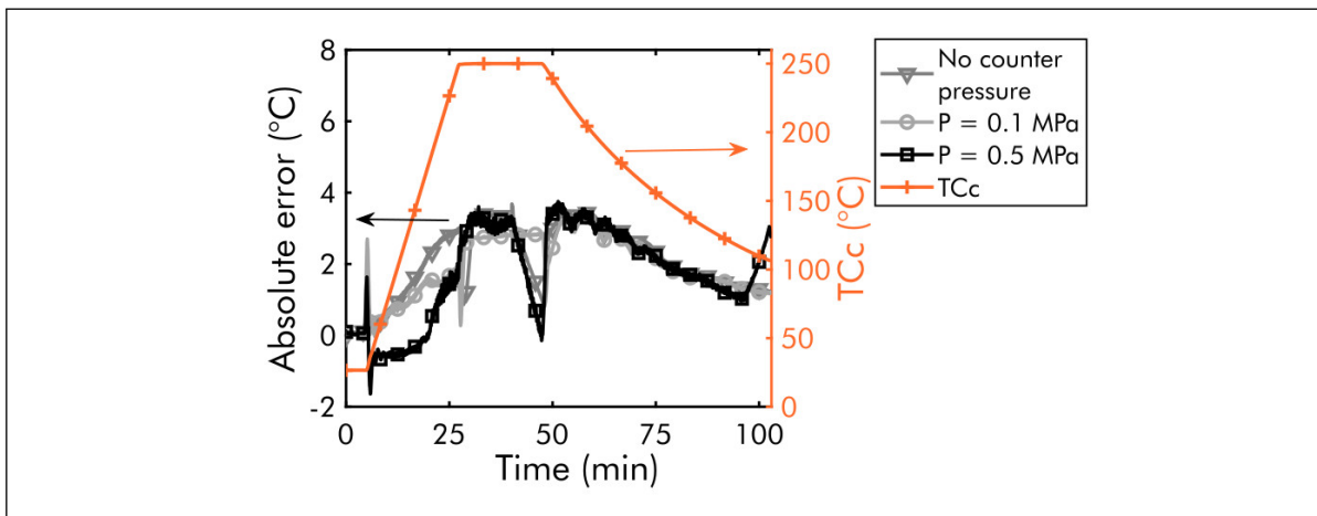
Figure 5.10: Model validation at a different pressures.
