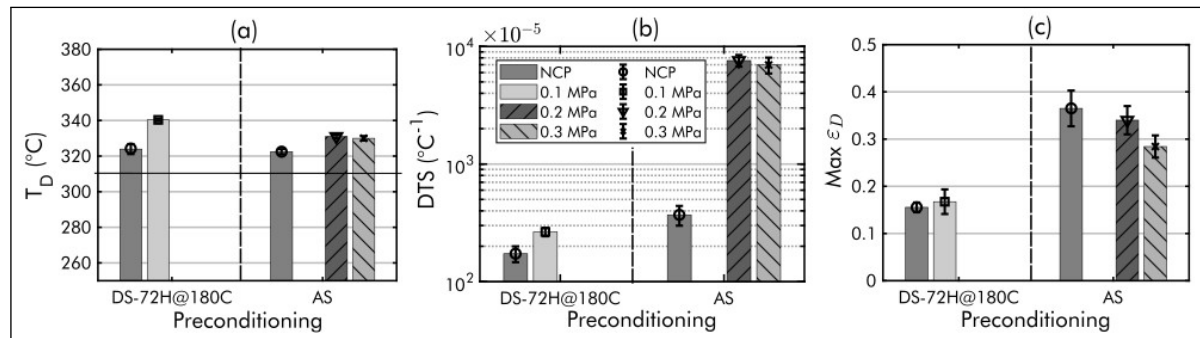
Figure 7.14: Effect of pressure on deconsolidation temperature T_D (a), deconsolidation's thermal sensitivity DTS (b) and the maximum deconsolidation strain \text{Max } \varepsilon_D (c) of AS and DS-72H@180C UD-HP samples tested at 10^\circ\text{C}/\text{min} under different counter pressure.
