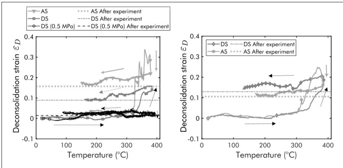
Figure 5.14: Deconsolidation graphs obtained at the sample center. Deconsolidation of Dried Sample (DS) and Ambient Storage sample (AS) samples heated at 10^{\circ}\text{C}/\text{min} (left) and at 60^{\circ}\text{C}/\text{min} (right).
