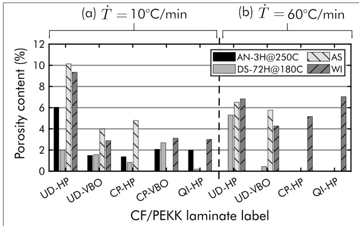
Figure 7.5: Final porosity content of some deconsolidated samples at 10^\circ\text{C}/\text{min} (a) and at 60^\circ\text{C}/\text{min} (b) under No Counter Pressure (NCP).
