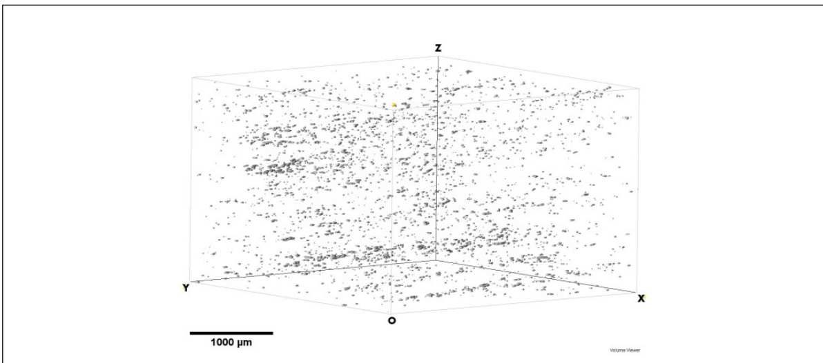
Figure 5.6: 3D image of the porosity distribution in a sample of 20 mm diameter cut from the consolidated laminate (Region Of Interest size: 3.81 mm \times 3.81 mm \times 2.48 mm). The porosity content is 0.02 %.
