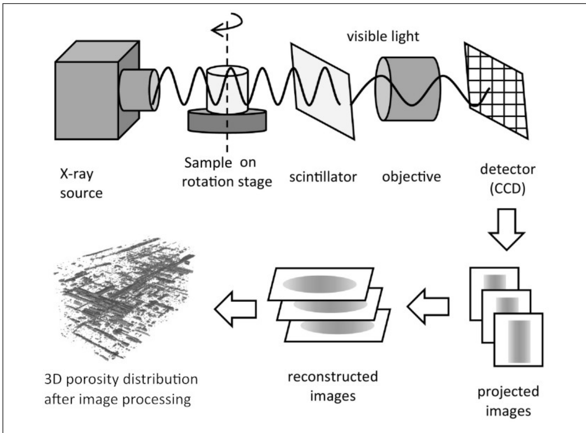
Figure 3.7: Schematic illustration of X-ray microtomography [39, 52].
