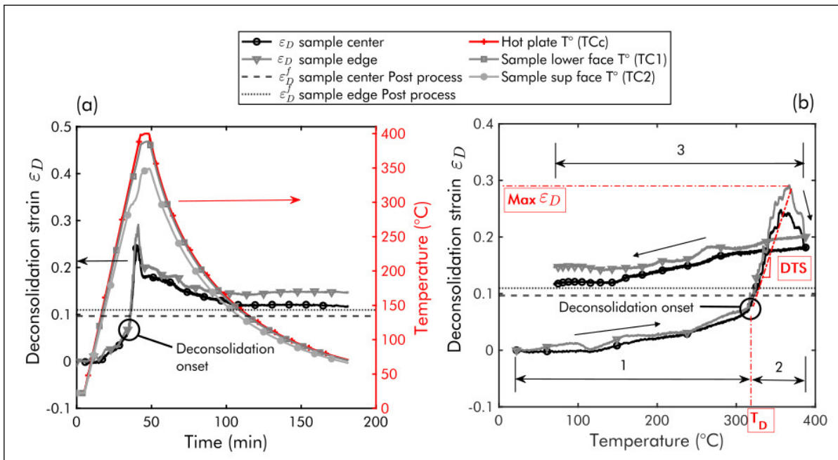
Figure 7.8: Continuous and online deconsolidation monitoring. Through thickness deconsolidation strain \epsilon_D vs time (a) and deconsolidation strain \epsilon_D vs the sample lower face temperature ( TC1 ) estimated with the thermal model (b) of a quasi isotropic ([0/90/+45/-45]_{2S}) laminate sample consolidated in Hot Press and stored in water at 23^\circ\text{C} for 1 year and then heated at 10^\circ\text{C}/\text{min} under No Counter Pressure (NCP).
