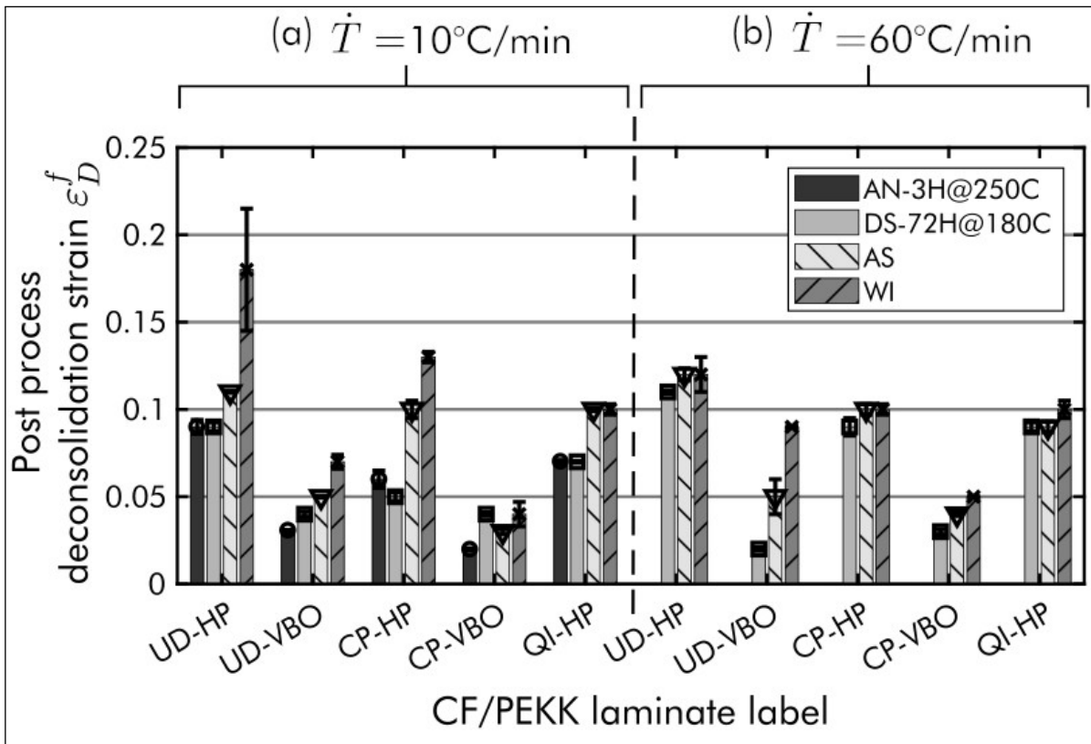
Figure 7.3: Post-process deconsolidation strain \varepsilon_D^f of the deconsolidated samples at 10^\circ\text{C}/\text{min} (a) and 60^\circ\text{C}/\text{min} (b) under No Counter Pressure (NCP).
