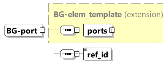
FIGURE 3.14 – XSD du BG-port
