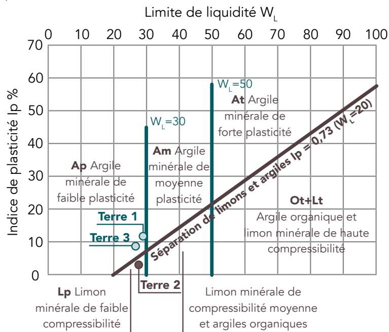
Figure 116 Fraction fine de la terre – classification.
