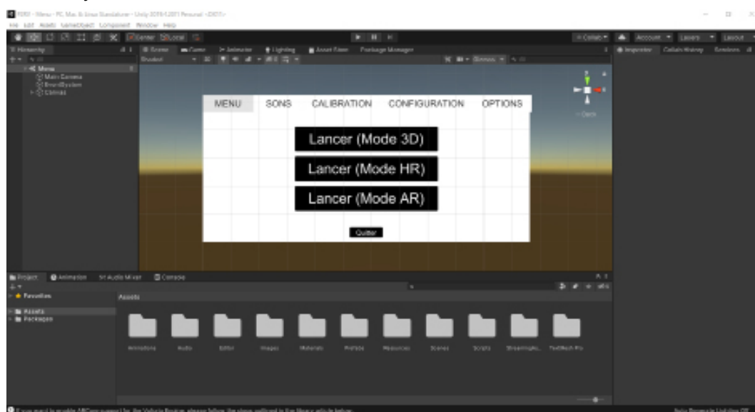
Figure 251 Unity Editor
