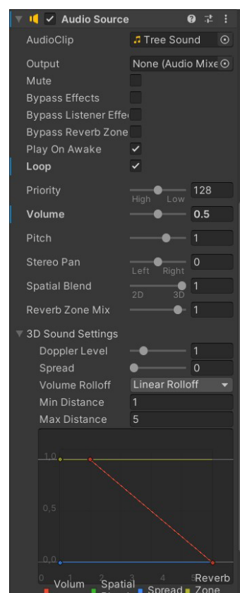
Figure 257 Audio Source.
