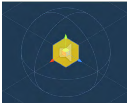
Figure 283 Cube Sound.
