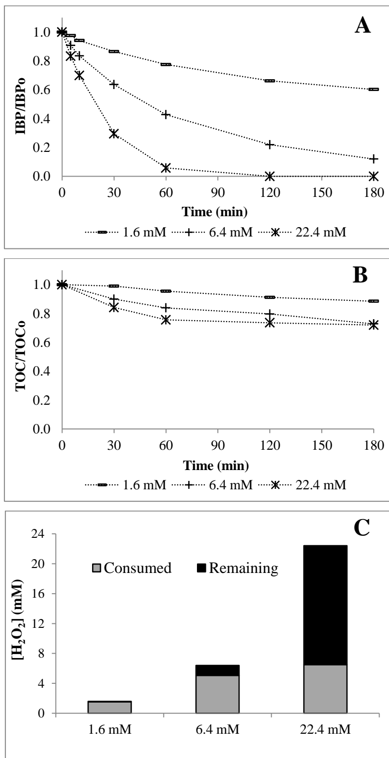
Figure 4.9. Effect of H 2 O 2 concentration on Fenton oxidation over Fe-MFI: evolution of (A) IBP and (B) TOC concentration, and (C) H 2 O 2 consumption ([IBP] 0 = 20 mg/L, [Fe-MFI] = 4.8 g/L, [H 2 O 2 ] = 1.6 – 22.4 mM (0.5 – 7 times stoichiometric amount), pH 0 = 4.3, T = 25°C)
