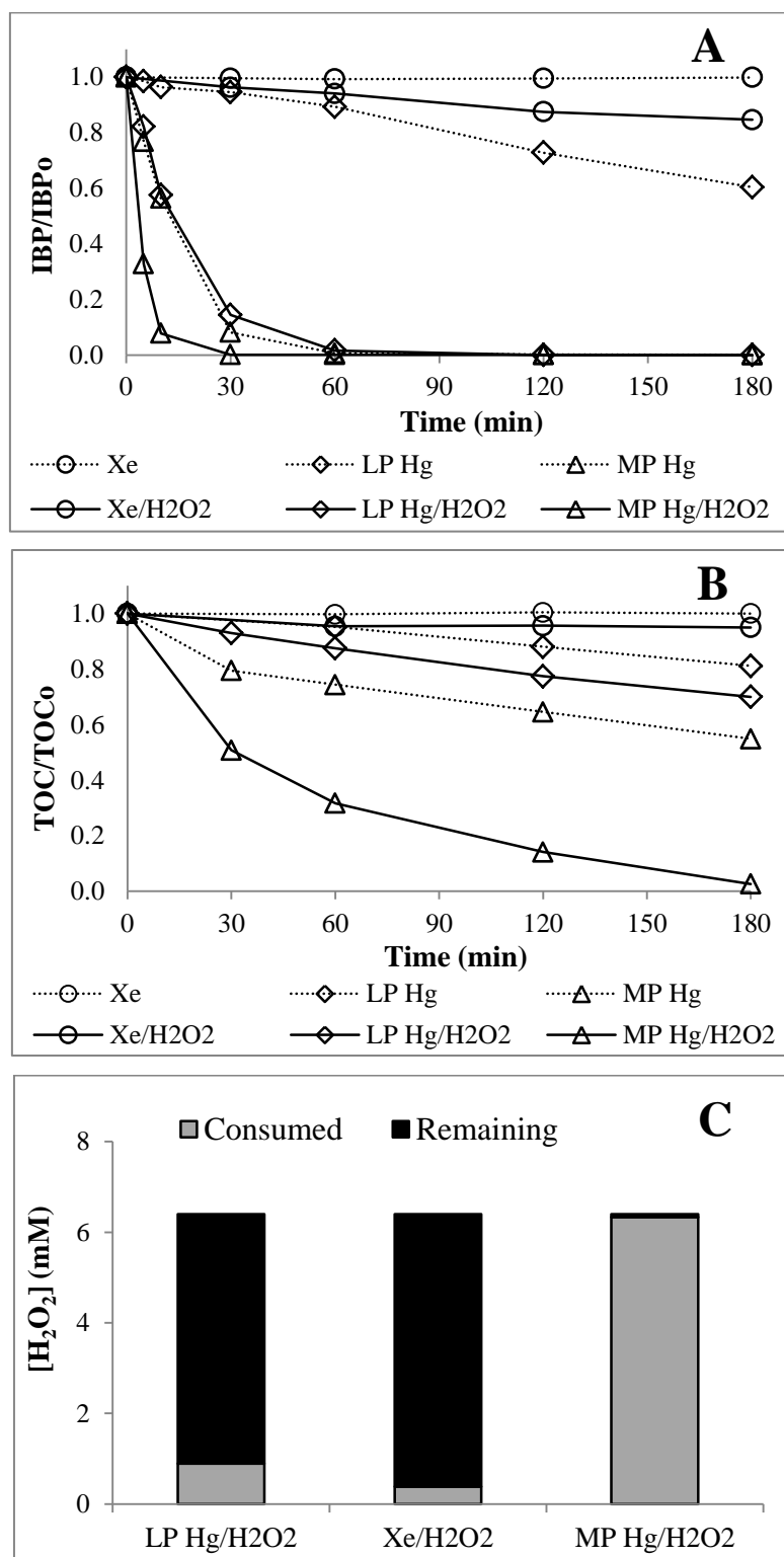
Figure 3.13. Effect of lamp type on photo-oxidation of IBP: (A) IBP and (B) TOC concentration-time profiles, and (C) H 2 O 2 consumption ([IBP] 0 = 20 mg/L, pH 0 = 4.3, T = 25°C, irradiated volume = 500 mL, total volume = 1500 mL, lamp = 6W LP Hg (UV), 150W Xe (Vis), or 150W MP Hg (UV-Vis), [H 2 O 2 ] 0 = 6.4 mM). Photolysis results are recalled for comparison purpose
