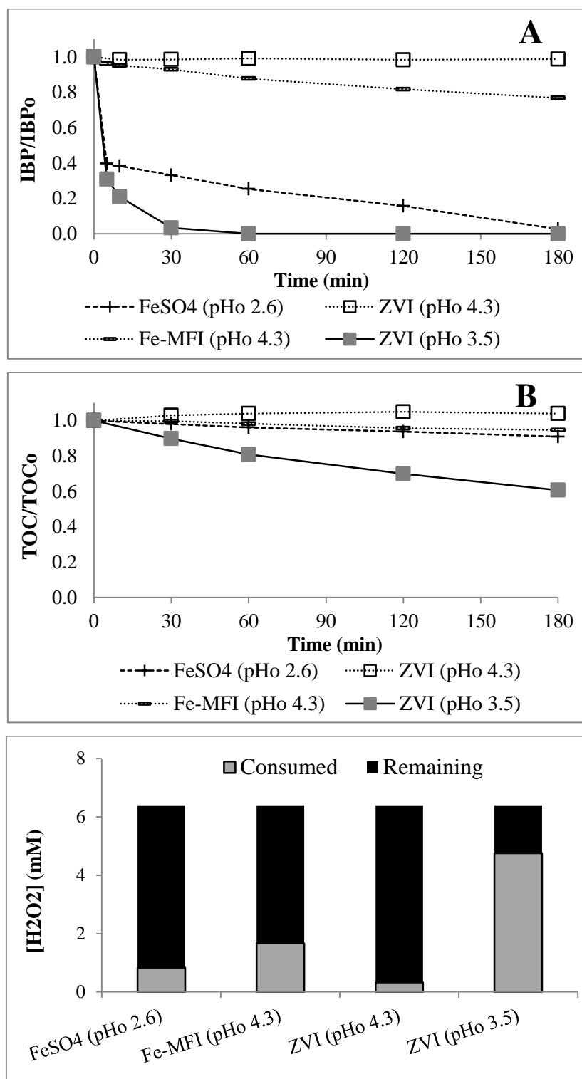
Figure 4.3. Fenton oxidation of ibuprofen over ZVI and Fe-MFI catalysts: evolution of (A) IBP and (B) TOC concentration and (C) H 2 O 2 consumption ([IBP] 0 = 20 mg/L, [Fe-MFI] = 1 g/L, [ZVI] = 0.056 g/L, [H 2 O 2 ] 0 = 6.4 mM, T = 25°C). Homogeneous Fenton oxidation using 0.13 mM of FeSO 4 ·7H 2 O was recalled for comparison
