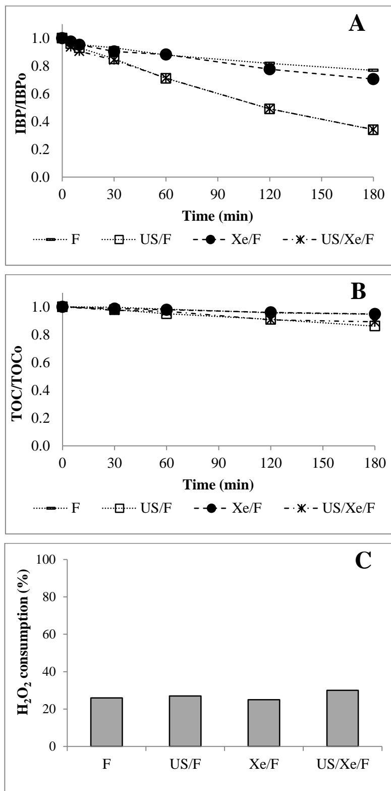
Figure 4.23. Sono-photo-Fenton oxidation with Fe-MFI under Vis light and 20 kHz US, and comparison with other Fenton-based processes: evolution of (A) IBP and (B) TOC concentration, and (C) H 2 O 2 consumption ([IBP] 0 = 20 mg/L, [Fe-MFI] = 1 g/L, [H 2 O 2 ] 0 = 6.4 mM, pH 0 = 4.3, T = 25°C, f US = 20 kHz, D US = 50W/L, Vis lamp: Xenon 150 W)
