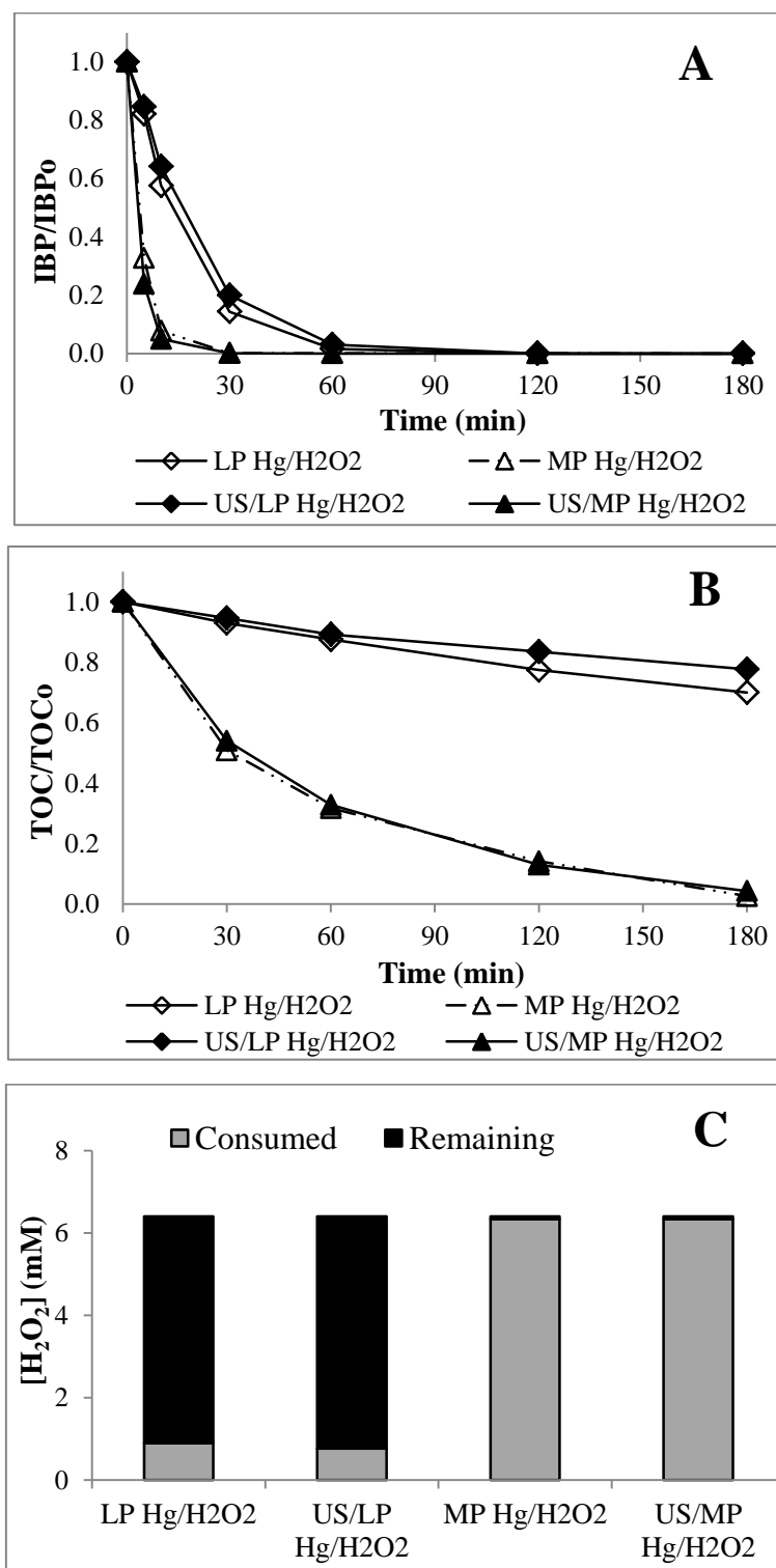
Figure 3.17. Sonophoto-oxidation of IBP: (A) IBP and (B) TOC concentration-time profiles, and (C) H 2 O 2 consumption.
