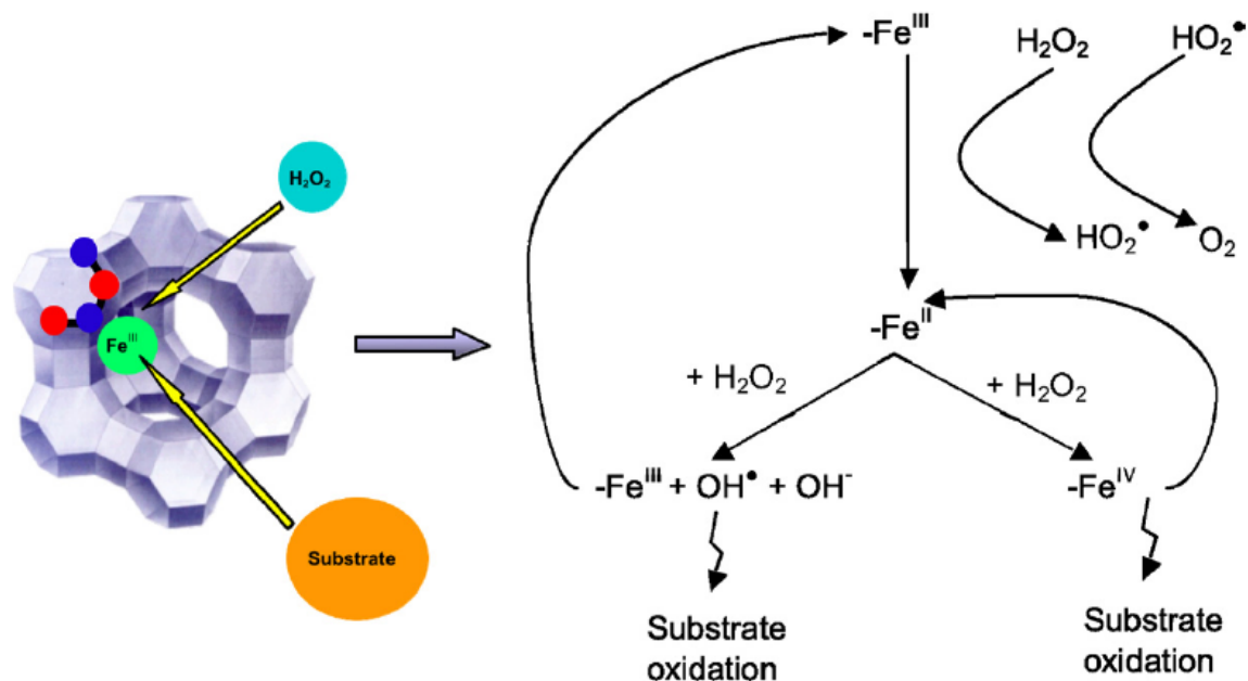
Figure 1.6. Representation of possible mechanisms involved in heterogeneous Fenton-like reactions catalyzed by Fe-zeolites (adapted from reference [50])
