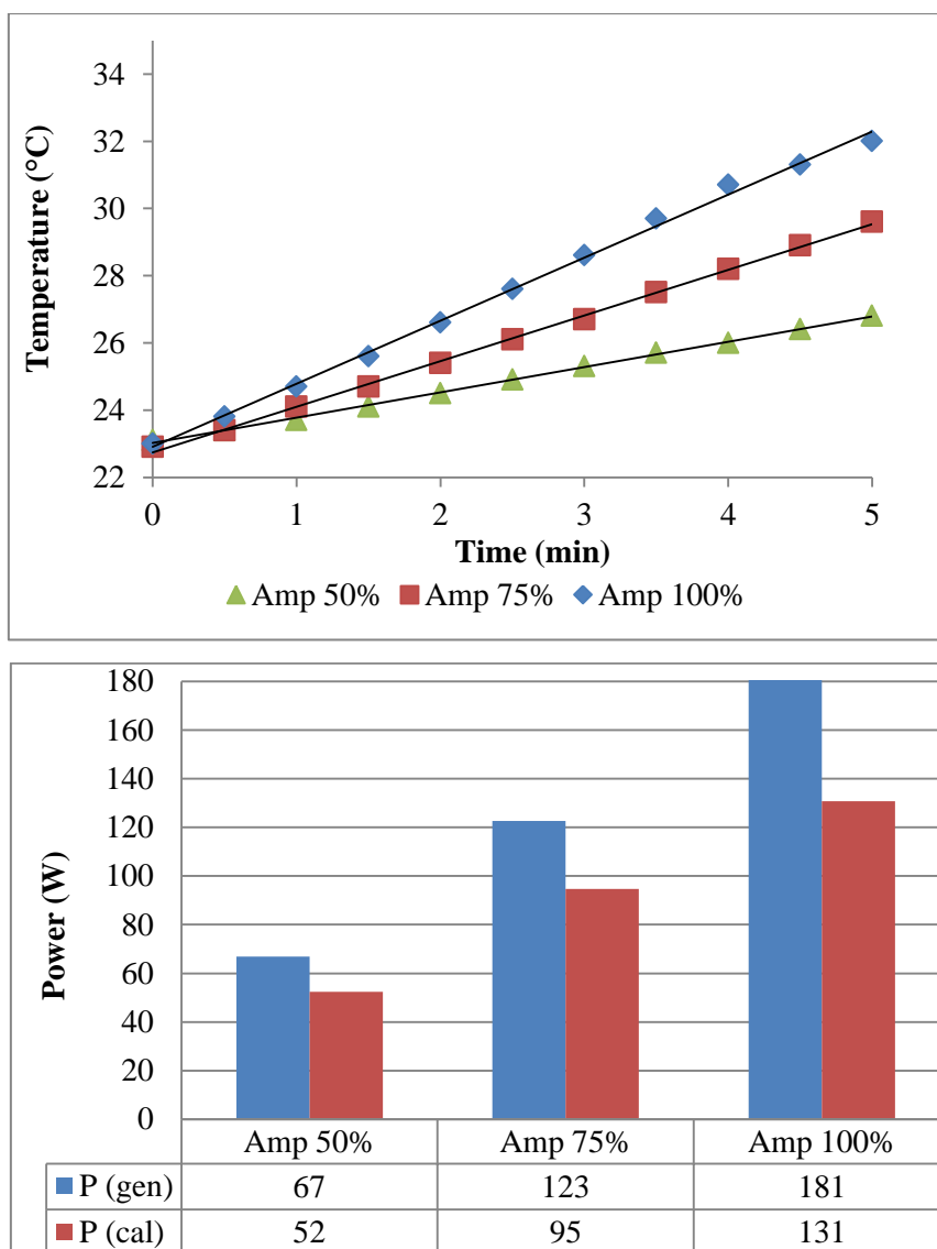
Figure 2.19. Calorimetric evaluation of ultrasonic equipment 1 Amp: Amplitude, P_{gen} : Electrical power consumed by US generator (W), P_{cal} : calorimetric power (W)
