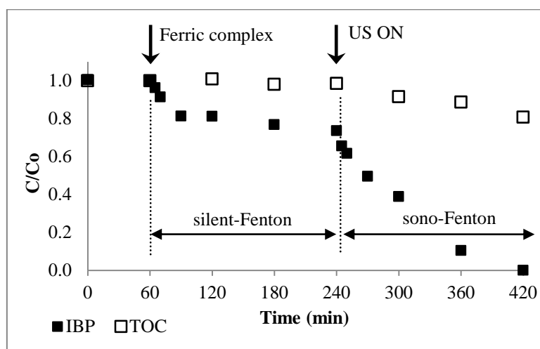
Figure 3.19. Effect of sonication on Fenton catalyst regeneration ([IBP] 0 = 20 mg/L, pH 0 = 2.6, T = 25°C, f US = 20 kHz, D US = 50W/L, [H 2 O 2 ] 0 = 6.4 mM, [Fe 2+ ] 0 = 0.134 mM)
