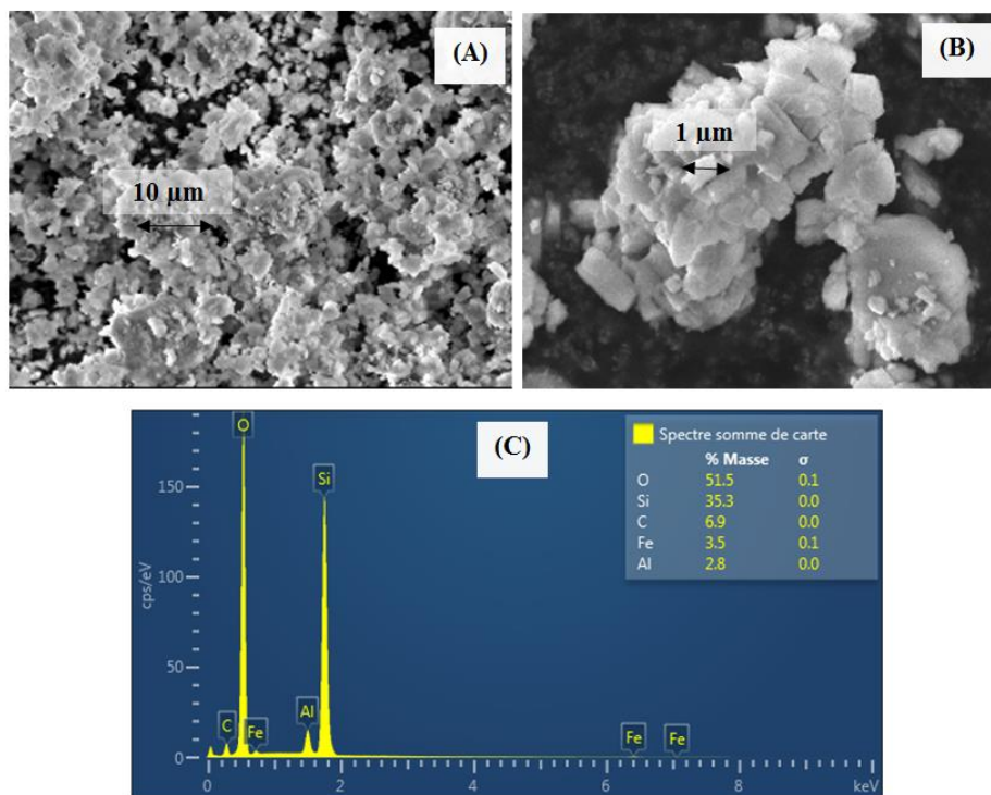
Figure 2.11. SEM images (A and B) and EDX analysis (C) of fresh Fe-MFI catalyst
