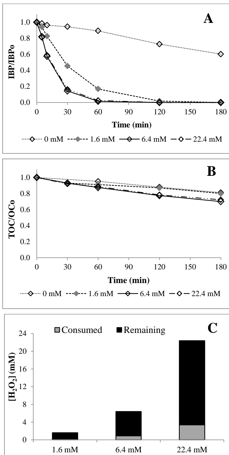
Figure 3.12. Effect of H 2 O 2 concentration on photo-oxidation of IBP: (A) IBP and (B) TOC concentration-time profiles, and (C) H 2 O 2 consumption ([IBP] 0 = 20 mg/L, pH 0 = 4.3, T = 25°C, irradiated volume = 500 mL, total volume = 1500 mL, lamp = 6W LP Hg, [H 2 O 2 ] 0 = 0 – 22.4 mM)
