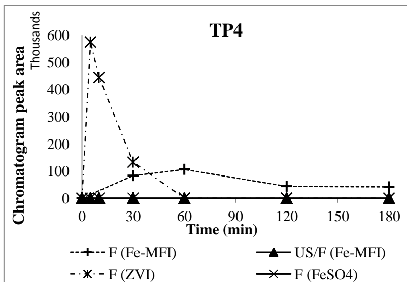
Figure 4.30. Evolution of TP4 concentration during heterogeneous Fenton-based processes (results of homogeneous Fenton reaction with ferrous iron salt were recalled for comparison purpose) ( \text{pH}_0 \text{ Fe-MFI} = 4.3 ; \text{pH}_0 \text{ ZVI} = 3.5 ; \text{pH}_0 \text{ FeSO}_4 = 2.6 )
