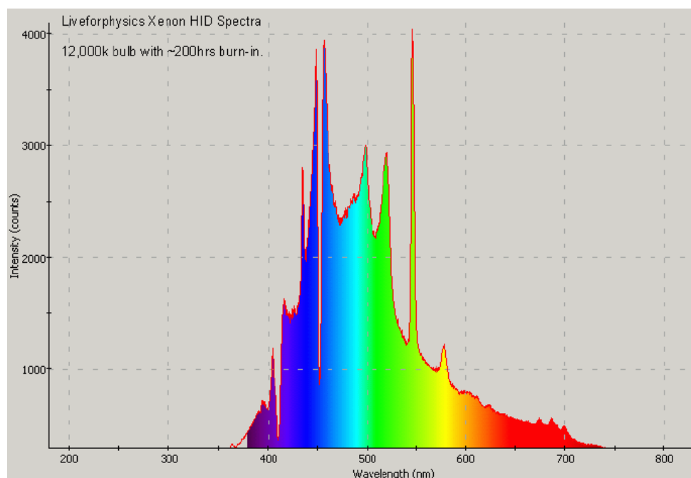
Figure 2.22. Spectral distribution of lamp TXE150 lamp (xenon arc lamp) (Data provided by supplier)
