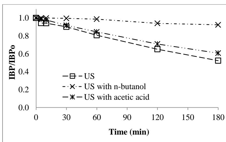
Figure 3.2. Sonolysis of IBP and effect of radical scavenger ([IBP] 0 = 20 mg/L, pH 0 = 4.3, T = 25°C, f US = 20 kHz, D US = 50 W/L, [Scavengers] 0 = 50 mM)
