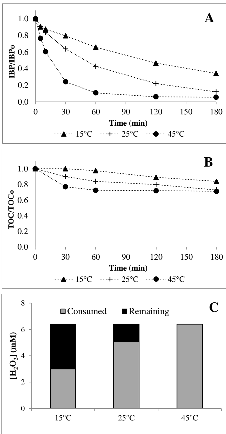
Figure 4.11. Effect of temperature on Fenton oxidation over Fe-MFI: evolution of (A) IBP and (B) TOC concentration, and (C) H 2 O 2 consumption ([IBP] 0 = 20 mg/L, [Fe-MFI] = 4.8 g/L, [H 2 O 2 ] 0 = 6.4 mM, pH 0 = 4.3, T = 15 – 45°C)
