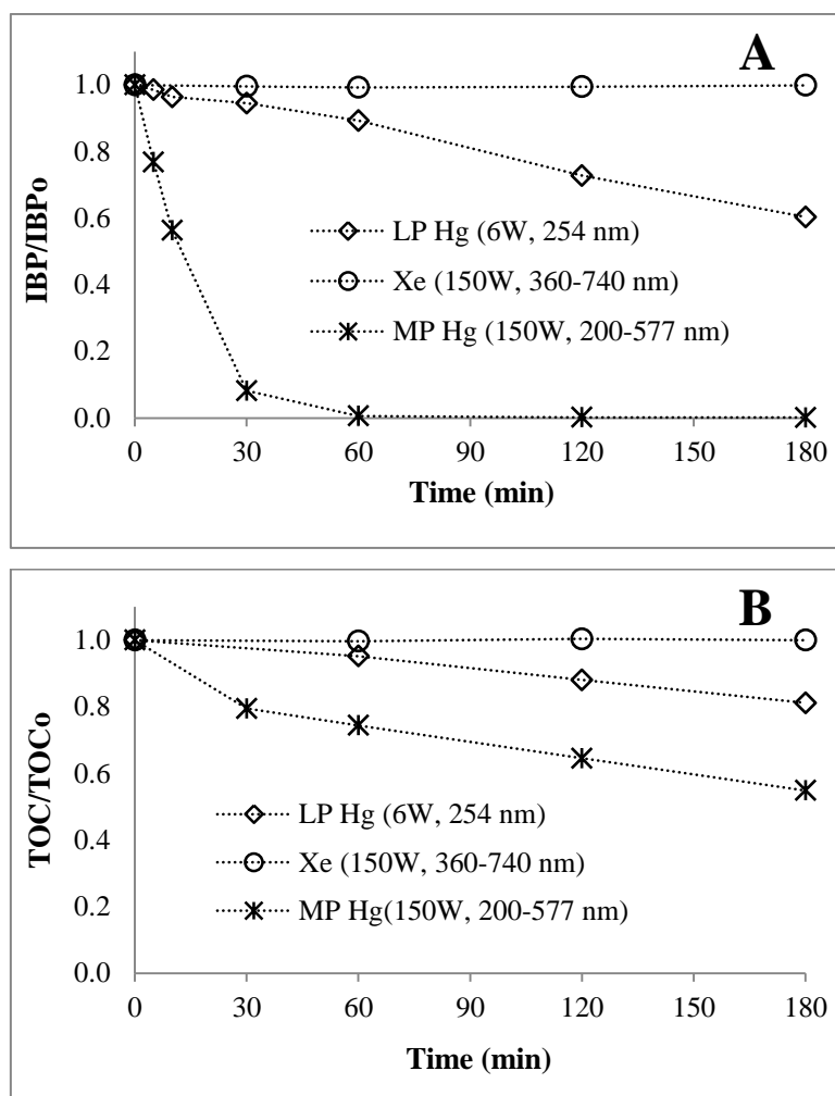
Figure 3.11. Effect of lamp type on IBP photolysis: (A) IBP and (B) TOC concentration-time profiles ([IBP] 0 = 20 mg/L, pH 0 = 4.3, T = 25°C, irradiated volume = 500 mL, total volume = 1500 mL, lamp = 6W LP Hg, 150W Xe, or 150W MP Hg)
