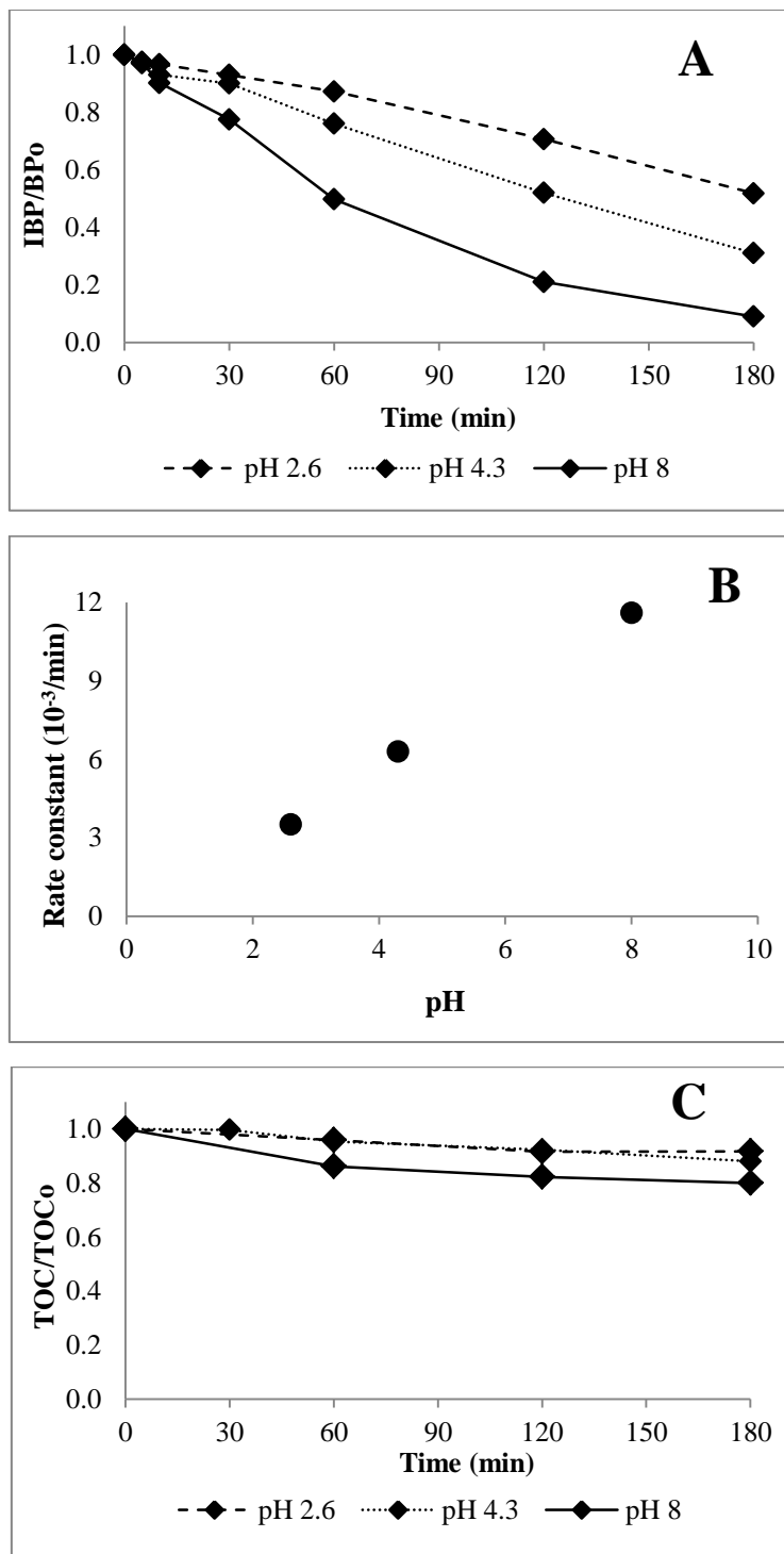
Figure 3.9. Effect of the solution pH on IBP photolysis: (A) IBP concentration-time profile, (B) first-order rate constant, (C) TOC concentration-time profile ( [IBP]_0 = 20\text{ mg/L} , pH_0 = 2.6 - 8.0 , T = 25^\circ\text{C} , irradiated volume = 500 mL, lamp = 6W LP Hg)
