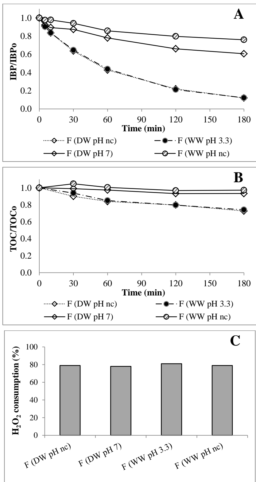
Figure 4.32. Effect of WW matrix on heterogeneous Fenton process: evolution of (A) IBP and (B) TOC concentration, and (C) H 2 O 2 consumption ([IBP] 0 = 20 mg/L, [Fe-MFI] = 4.8 g/L, [H 2 O 2 ] 0 = 6.4 mM, pH nc: pH not controlled, T = 25°C)
