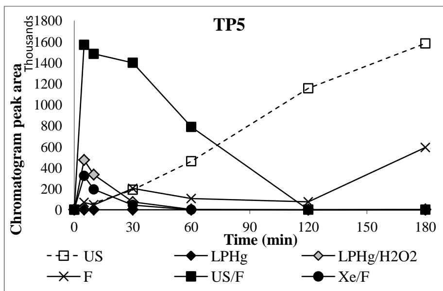
Figure 3.33. Evolution of TP5 concentration during homogeneous AOPs
