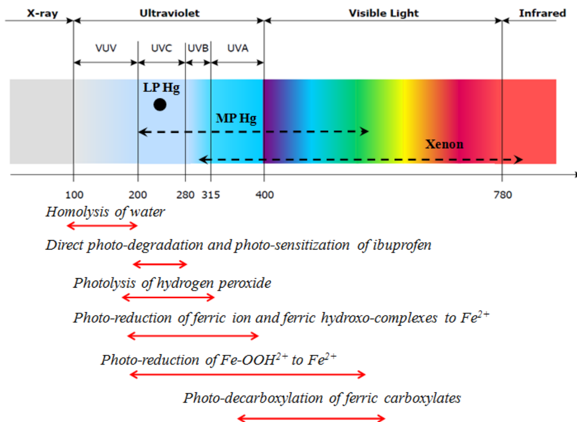
Figure 2.23. Irradiation spectrum of the lamps vs. useful ranges for the different photochemical reactions
