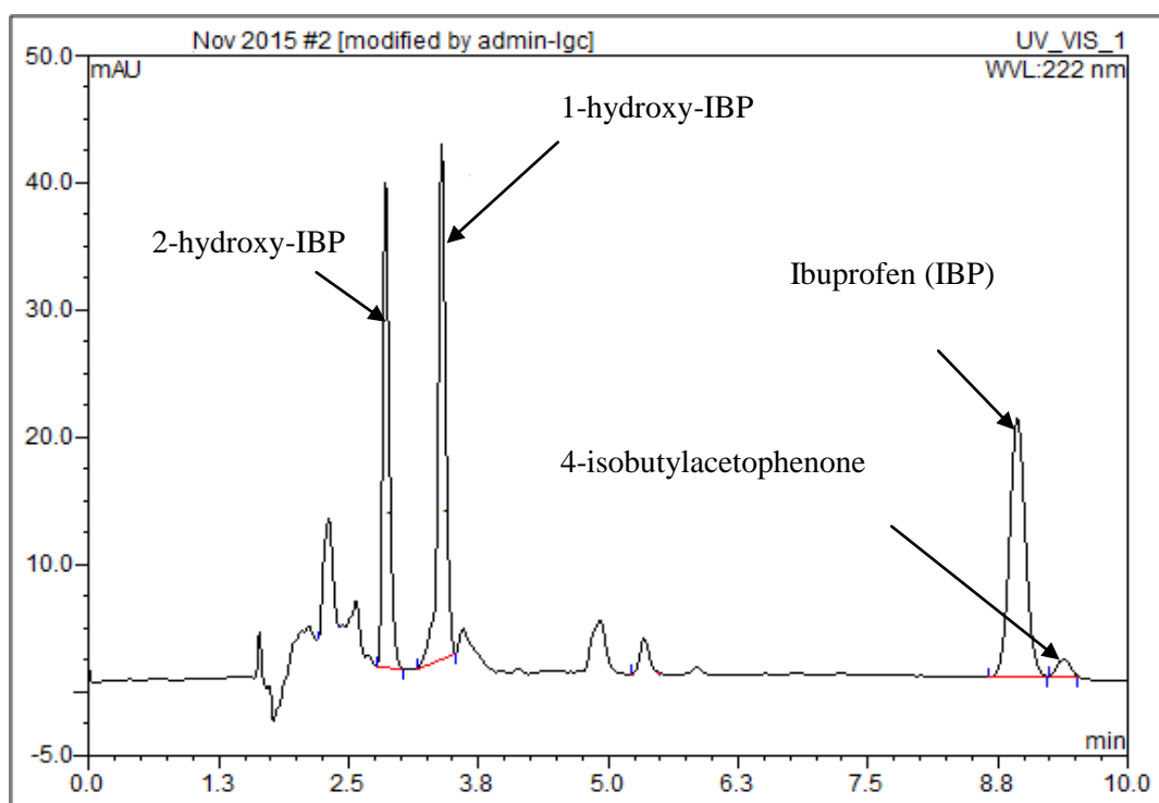
Figure I. Separation of IBP and transformation products by HPLC/UV
