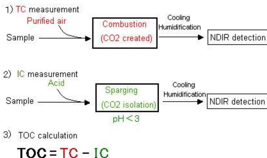
Figure 2.3. Principle of TOC measurement (adapted from reference [212])
