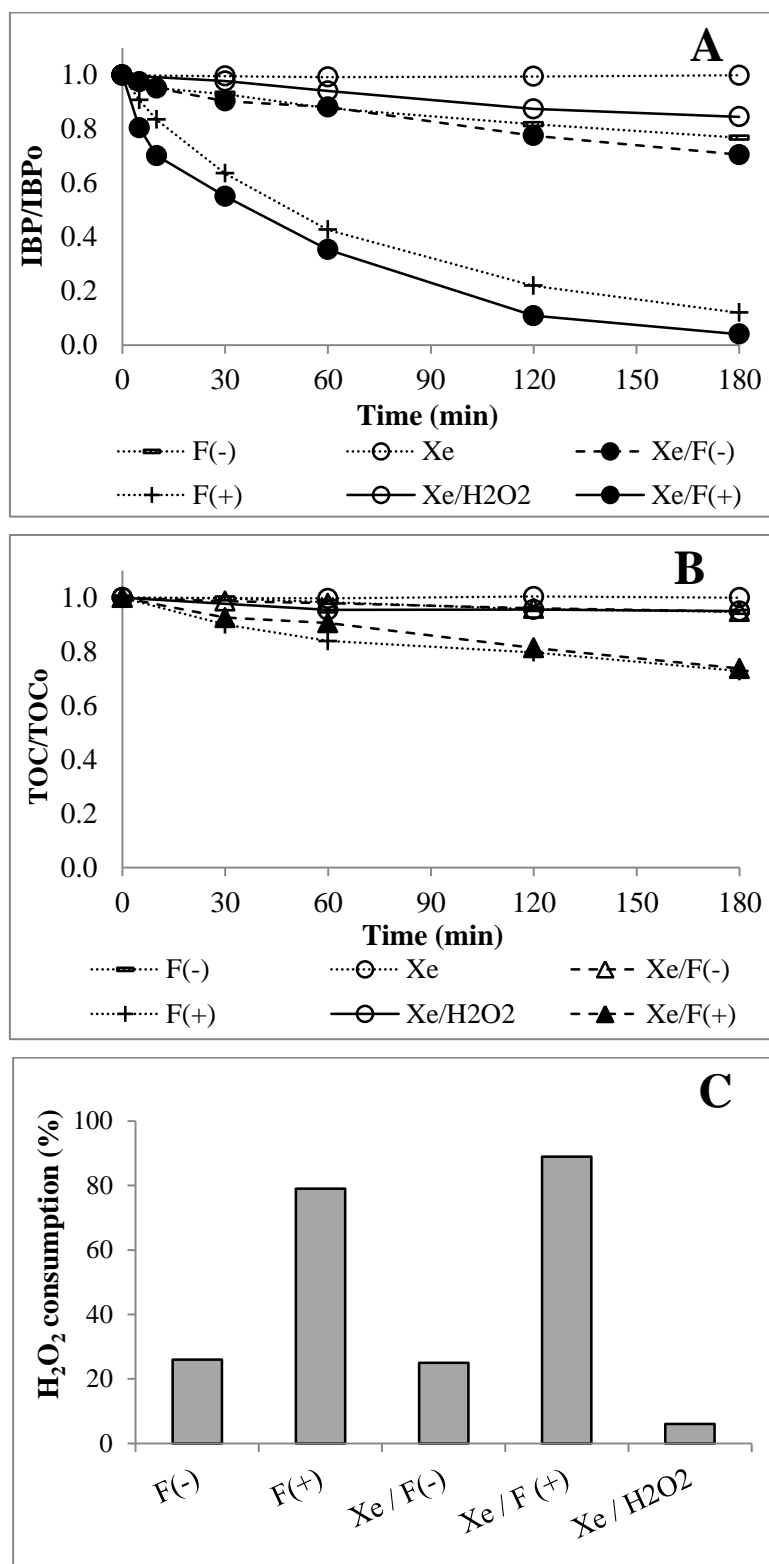
Figure 4.21. Photo-Fenton oxidation with Fe-MFI under Vis light and comparison with separate processes: evolution of (A) IBP and (B) TOC concentration and (C) H 2 O 2 consumption ([IBP] 0 = 20 mg/L, [Fe-MFI] = 1 and 4.8 g/L, [H 2 O 2 ] 0 = 6.4 mM, pH 0 = 4.3, T = 25°C, Vis lamp: Xenon 150W)
