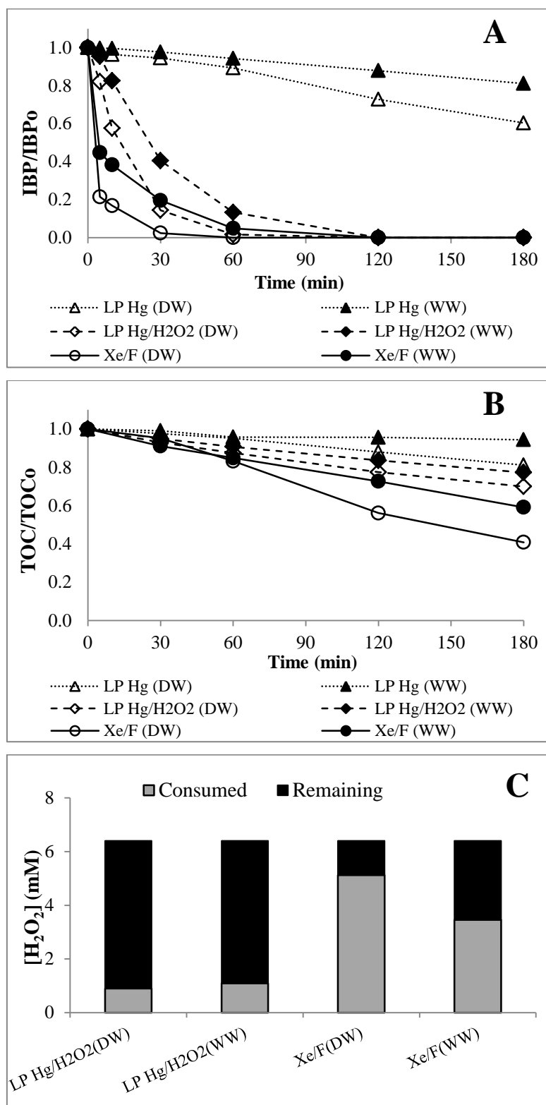
Figure 3.35. Effect of water matrix (DW: distilled water, WW: wastewater effluent) on UV photolysis (LP Hg), UV/H 2 O 2 (LP Hg/H 2 O 2 ) and photo(Vis)-Fenton (Xe/F) oxidation of IBP: (A) IBP and (B) TOC concentration-time profiles, and (C) H 2 O 2 consumption. ([IBP] 0 = 20 mg/L, pH 0 = 8.0, except for Xe/F in WW (pH 0 = 2.6), T = 25°C, irradiated vol. fraction = 1/3, lamp = 6W LP Hg (UV) or 150W Xe (Vis), [H 2 O 2 ] 0 = 6.4 mM and [Fe 2+ ] 0 = 0.134 mM for Xe/F)
