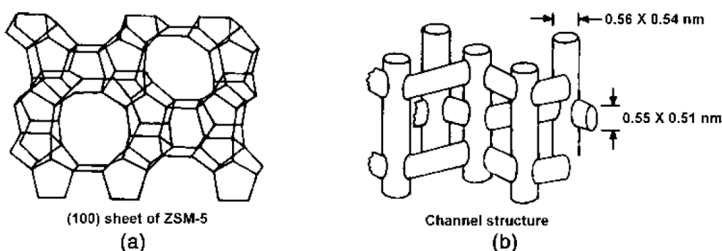
Figure 2.10. (a) Skeletal diagram of the (100) face of ZSM5, (b) Channel structure of ZSM5 (adapted from reference [234])
