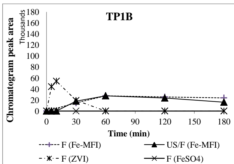
Figure 4.29. Evolution of TP1B concentration during heterogeneous Fenton-based processes (results of homogeneous Fenton reaction with ferrous iron salt were recalled for comparison purpose) ( \text{pH}_0_{\text{Fe-MFI}} = 4.3 ; \text{pH}_0_{\text{ZVI}} = 3.5 ; \text{pH}_0_{\text{FeSO}_4} = 2.6 )
