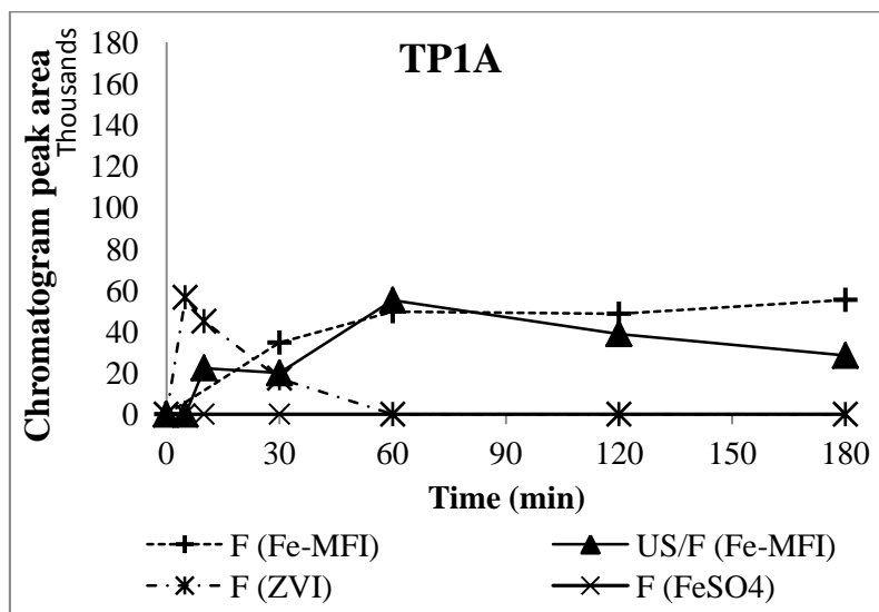
Figure 4.28. Evolution of TP1A concentration during heterogeneous Fenton-based processes (results of homogeneous Fenton reaction with ferrous iron salt were recalled for comparison purpose) ( \text{pH}_0_{\text{Fe-MFI}} = 4.3 ; \text{pH}_0_{\text{ZVI}} = 3.5 ; \text{pH}_0_{\text{FeSO}_4} = 2.6 )
