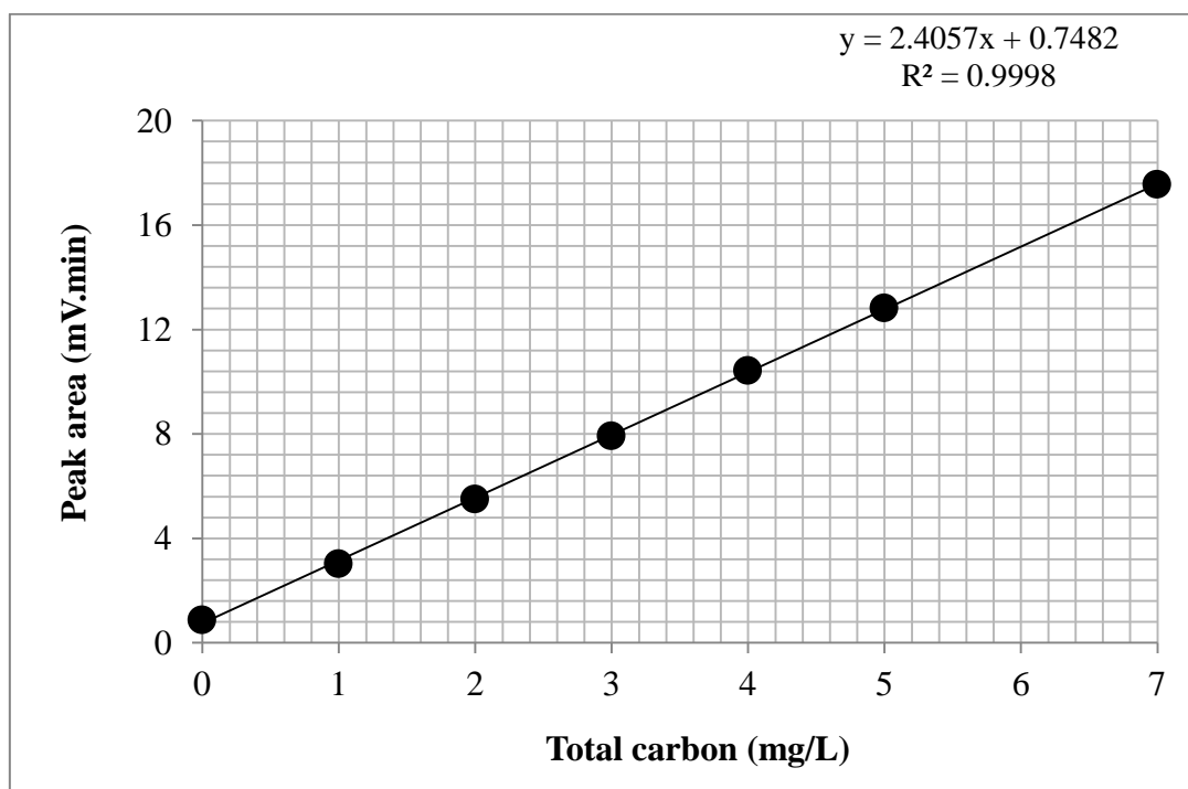
Figure III. Calibration curve of total carbon (TC)
