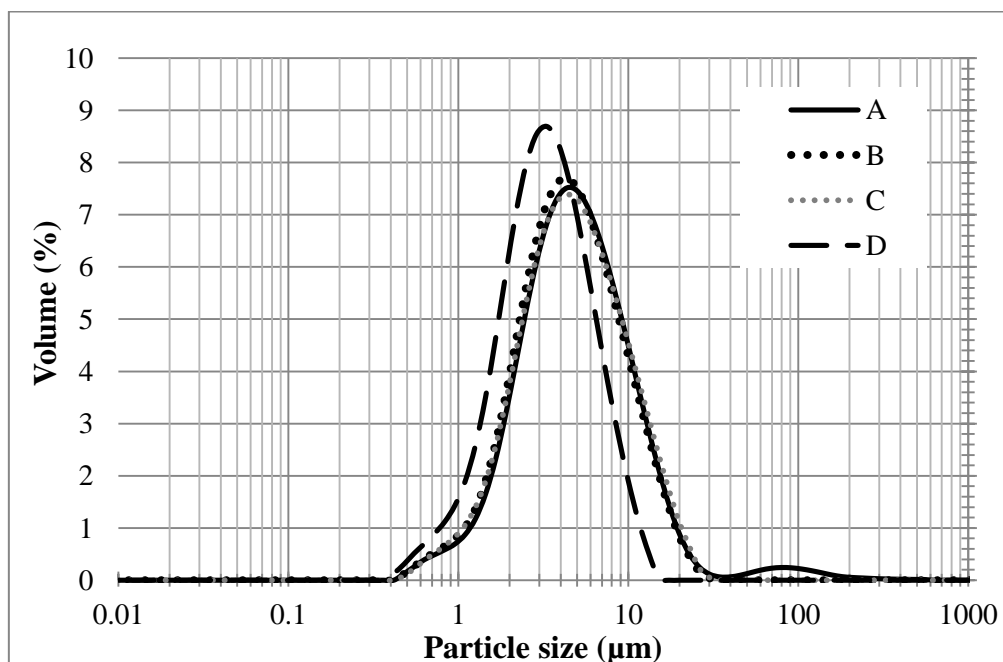
Figure 4.24. Fe-MFI particle size distribution: (A) before reaction, (B) after Fenton, (C) after photo-Fenton, (D) after sono-Fenton oxidation
