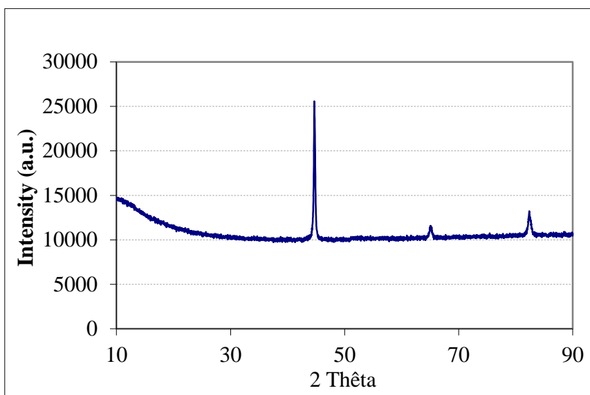
Figure 2.17. XRD pattern of fresh ZVI
