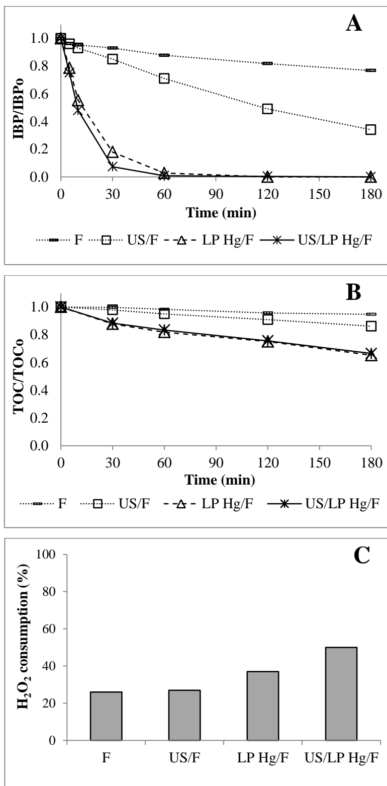
Figure 4.22. Sono-photo-Fenton oxidation with Fe-MFI under UV light and 20 kHz US, and comparison with other Fenton-based processes: evolution of (A) IBP and (B) TOC concentration, and (C) H 2 O 2 consumption ([IBP] 0 = 20 mg/L, [Fe-MFI] = 1 g/L, [H 2 O 2 ] 0 = 6.4 mM, pH 0 = 4.3, T = 25°C, f US = 20 kHz, D US = 50W/L, UV lamp: LP Hg 6 W)
