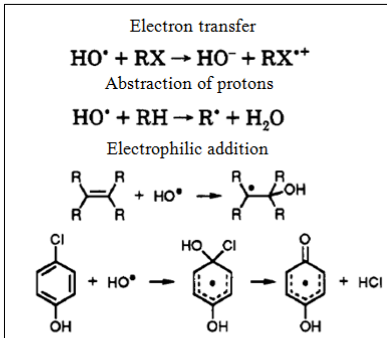
Figure 1.2. General scheme of hydroxyl radical based reactions (adapted from reference [34])
