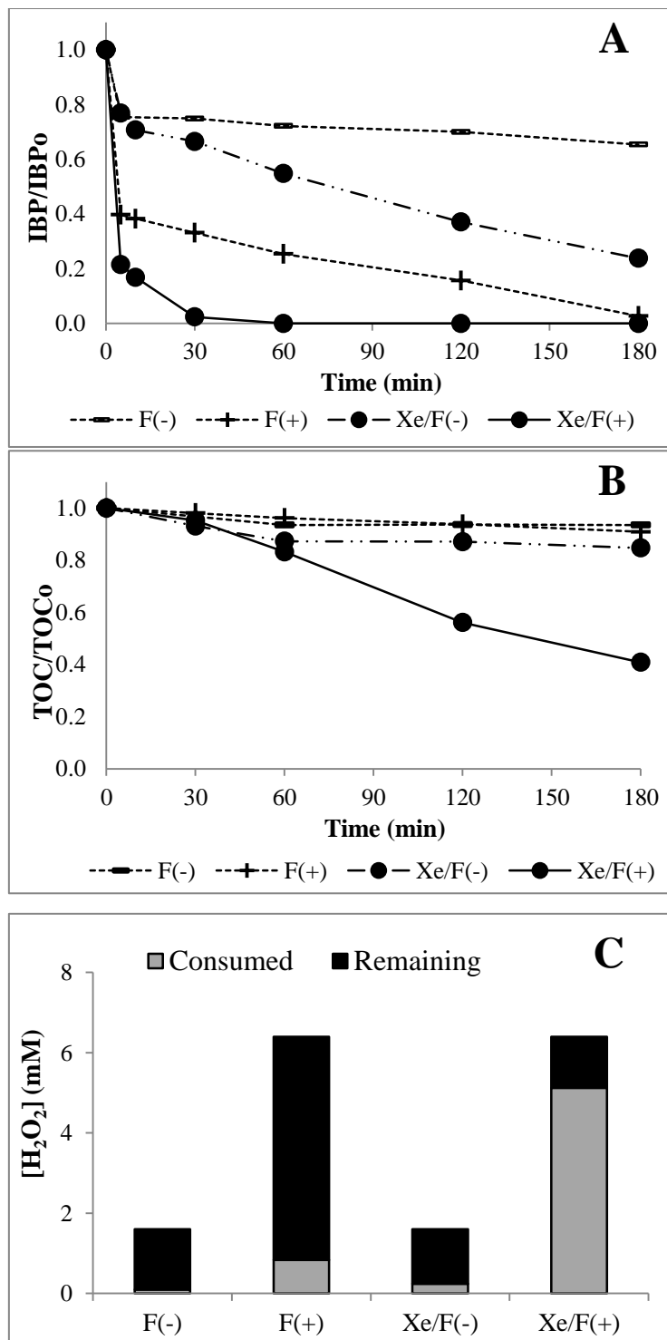
Figure 3.23. Effect of the concentration of Fenton's reagent on Fenton oxidation and photo-Fenton oxidation of IBP under visible irradiation: (A) IBP and (B) TOC concentration-time profiles ( [IBP]_0 = 20 mg/L, pH = 2.6, T = 25°C, irradiated volume fraction = 1/3, lamp = 150W Xe (Vis), F(-): [Fe^{2+}]_0 = 0.033 mM and [H_2O_2]_0 = 1.6 mM, F(+): [Fe^{2+}]_0 = 0.134 mM and [H_2O_2]_0 = 6.4 mM)
