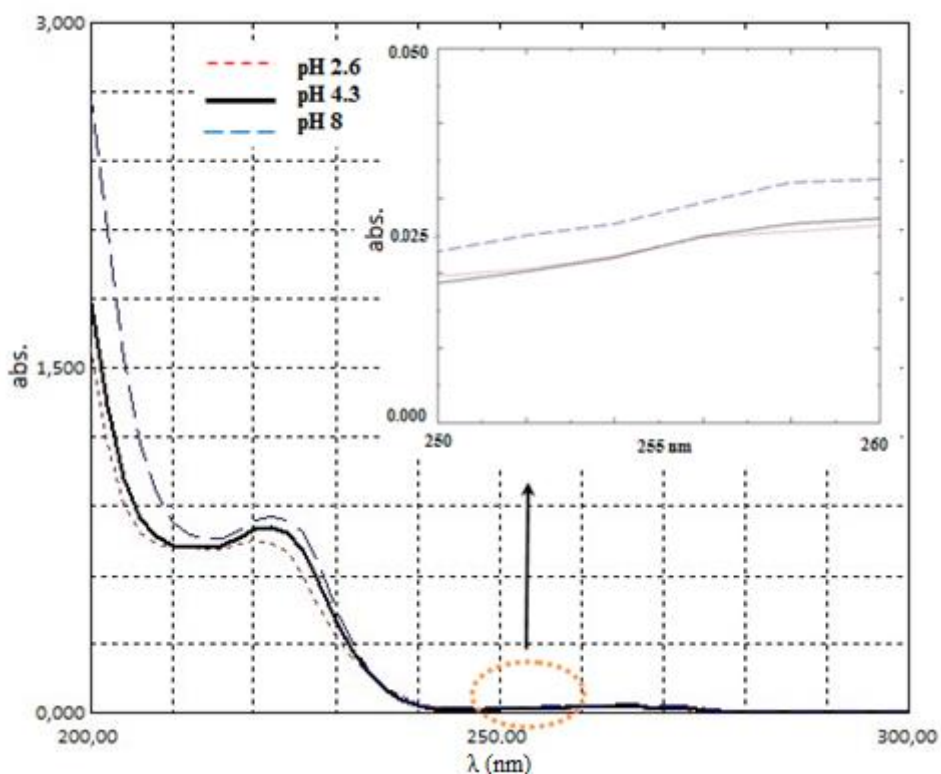
Figure 3.8. Effect of pH on UV absorption spectrum of IBP ([IBP] = 20 mg/L)
