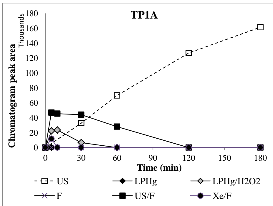
Figure 3.30. Evolution of TP1A concentration during homogeneous AOPs
