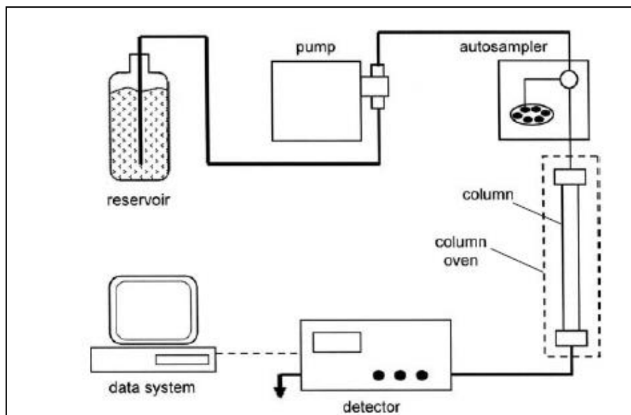
Figure 2.1. Schematic diagram of HPLC system (adapted from reference [210])
