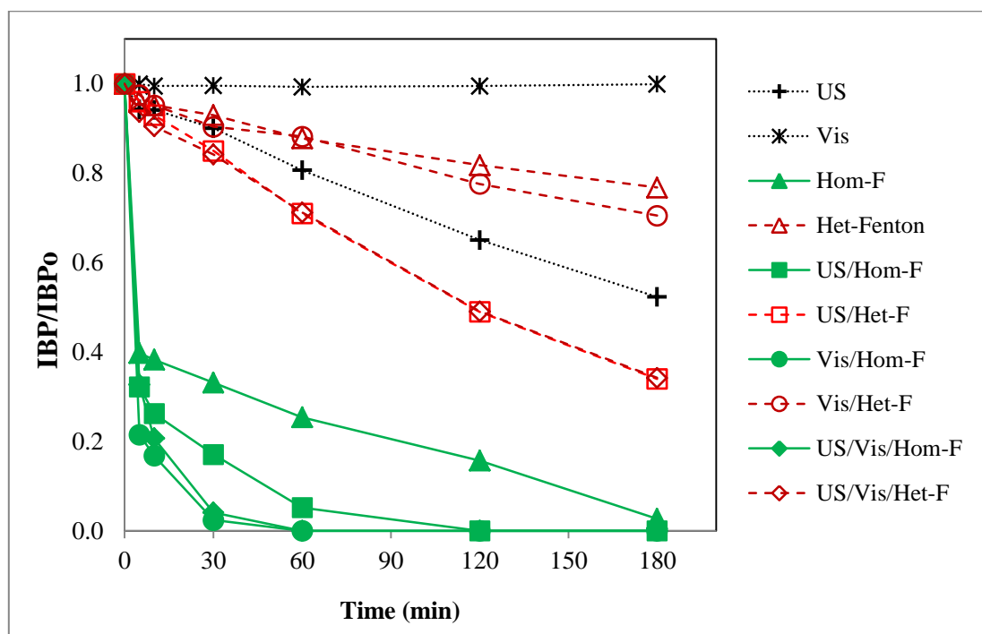
Comparison of homogeneous and heterogeneous process: IBP concentration-time profiles ( [\text{IBP}]_0 = 20 \text{ mg/L} , [\text{H}_2\text{O}_2]_0 = 6.4 \text{ mM} , [\text{Fe}^{2+}]_0 = 0.134 \text{ mM} or [\text{Fe-MFI}] = 1 \text{ g/L} , T = 25^\circ\text{C} , \text{pH}_0 = 2.6 or 4.3 , f_{\text{US}} = 20 \text{ kHz} , D_{\text{US}} = 50\text{W/L} , lamp = 150\text{W Xe (Vis)} )
