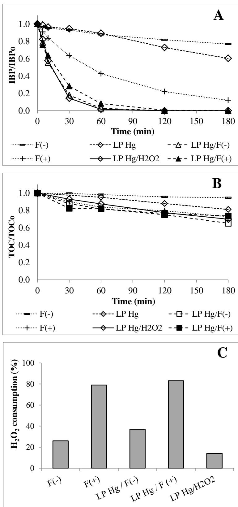
Figure 4.20. Photo-Fenton oxidation with Fe-MFI under UV light and comparison with separate processes: evolution of (A) IBP and (B) TOC concentration, and (C) H 2 O 2 consumption ([IBP] 0 = 20 mg/L, [Fe-MFI] = 1 and 4.8 g/L, [H 2 O 2 ] = 6.4 mM, pH 0 = 4.3, T = 25°C, UV lamp: LP Hg 6W)
