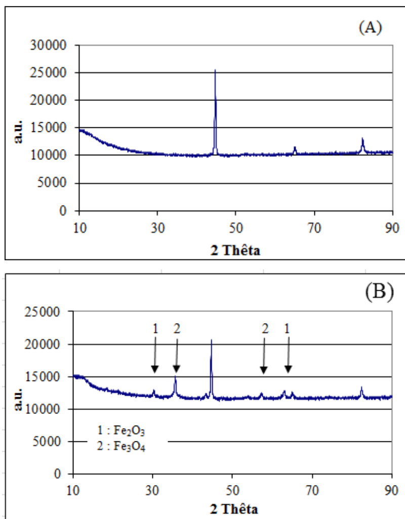
Figure 4.6. XRD analysis of (A) fresh and (B) used ZVI
