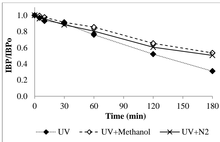
Figure 3.7. IBP photolysis and effect of radical scavenger or oxygen depletion ([IBP] 0 = 20 mg/L, pH 0 = 4.3, T = 25°C, irradiated volume = 500 mL, lamp = 6W LP Hg)
