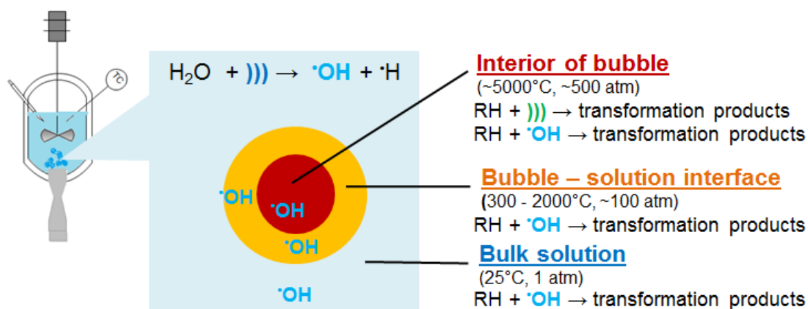
Figure 1.8. General mechanism of sonochemical reactions (adapted from reference [92])
