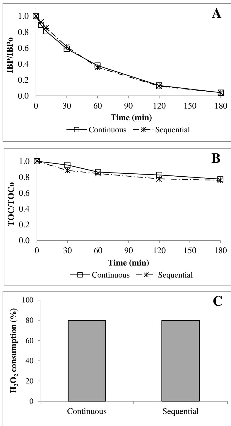
Figure 4.16. Effect of US application mode on sono-Fenton oxidation with Fe-MFI: evolution of (A) IBP and (B) TOC concentration, and (C) H 2 O 2 consumption ([IBP] 0 = 20 mg/L, pH 0 = 4.3, T = 25°C, [H 2 O 2 ] 0 = 6.4 mM, [Fe-MFI] = 4.8 g/L, f US = 20 kHz, E US = 540 kJ/kg, sequential mode: 10 s US ON / 10 s US OFF)
