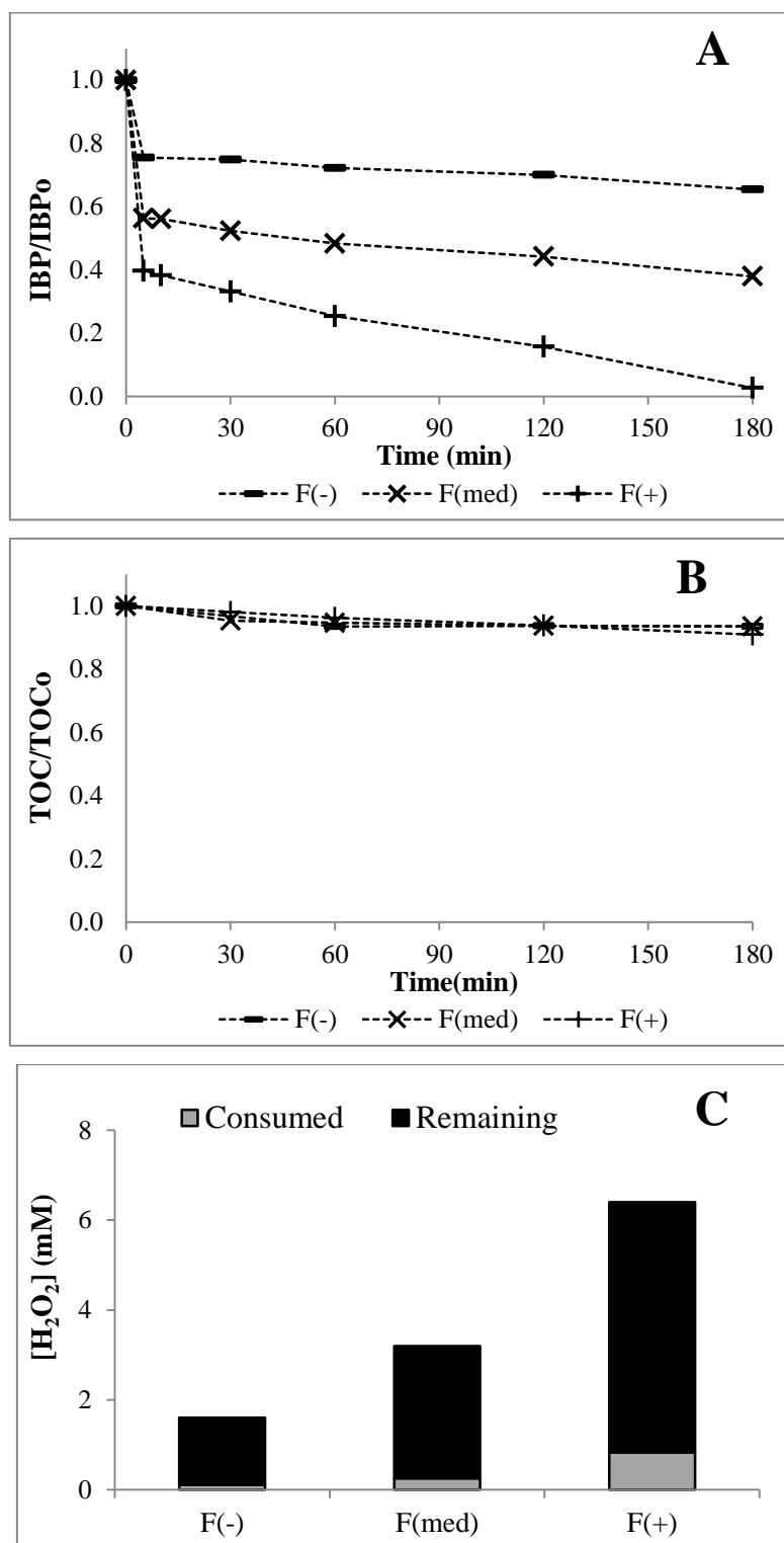
Figure 3.14. Effect of Fenton's reagent concentration on IBP oxidation: (A) IBP and (B) TOC concentration-time profiles, and (C) H 2 O 2 consumption ([IBP] 0 = 20 mg/L, pH 0 = 2.6, T = 25°C, F(-): [Fe 2+ ] 0 = 0.033 mM and [H 2 O 2 ] 0 = 1.6 mM, F(med): [Fe 2+ ] 0 = 0.067 mM and [H 2 O 2 ] 0 = 3.2 mM, F(+): [Fe 2+ ] 0 = 0.134 mM and [H 2 O 2 ] 0 = 6.4 mM)
