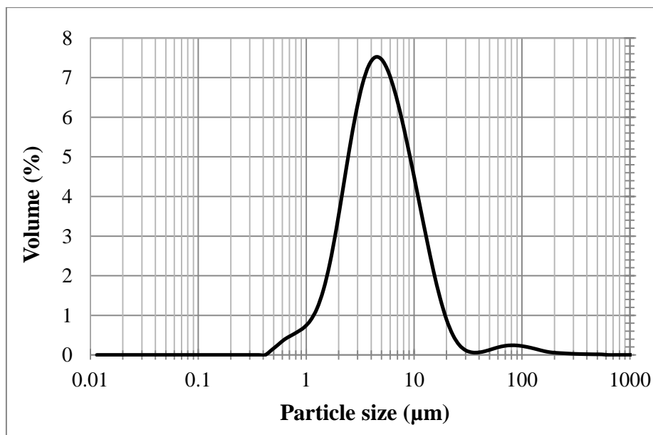
Figure 2.12. Particles size distribution of Fe-MFI (in suspension)
