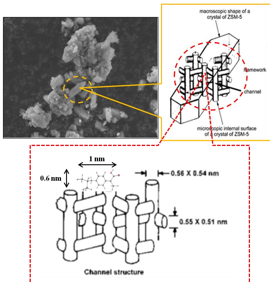
Figure 4.2. Illustration of IBP adsorption on zeolite surface
