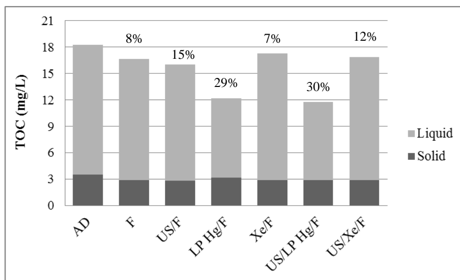
Figure 4.27. Carbon speciation after adsorption, Fenton oxidation and coupled processes ( [IBP]_0 = 20 mg/L, [Fe-MFI] = 1 g/L, [H_2O_2] = 6.4 mM, pH_0 = 4.3 , T = 25^\circ C ; US(-): f_{US} = 20 kHz, D_{US} = 50 W/L, UV: LP Hg lamp 6W, Vis: Xe lamp 150 W). Overall mineralization yield accounting for both liquid and solid phases is given above each bar
