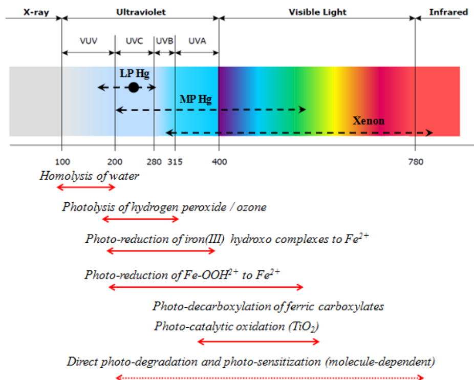
Figure 1.11. Classification of photo-based AOPs according to lamp type and wavelength
