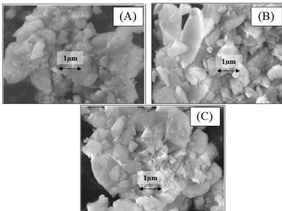
Figure 4.25. SEM images of (A) fresh and used Fe-MFI from (B) Fenton and (C) sono-Fenton oxidation
