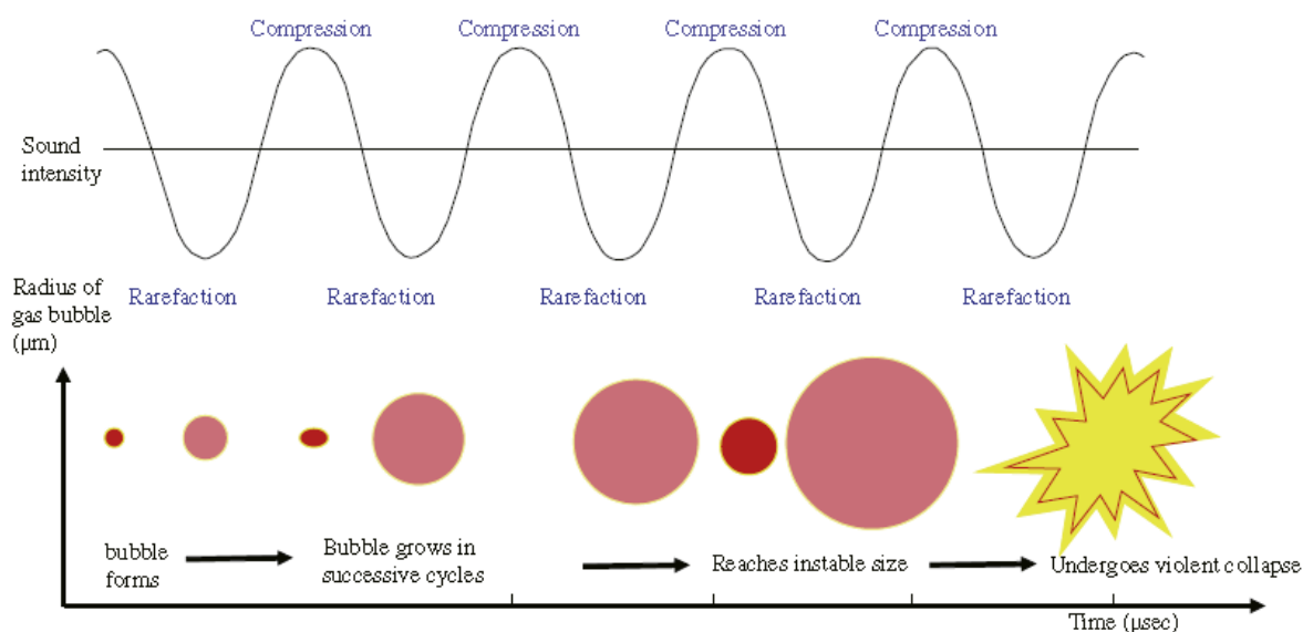
Figure 1.7. Typical scheme of acoustic cavitation (adapted from reference [89])
