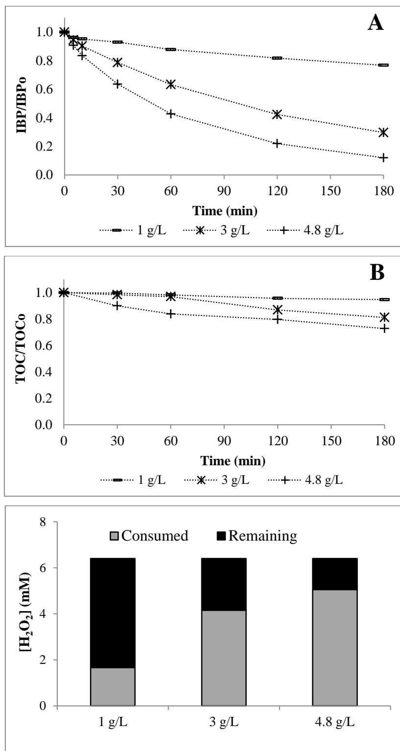
Figure 4.8. Effect of Fe-MFI concentration on Fenton oxidation: evolution of (A) IBP and (B) TOC concentration, and (C) H 2 O 2 consumption ([IBP] 0 = 20 mg/L, [Fe-MFI] = 1 – 4.8 g/L, [H 2 O 2 ] 0 = 6.4 mM, pH 0 = 4.3, T = 25°C)
