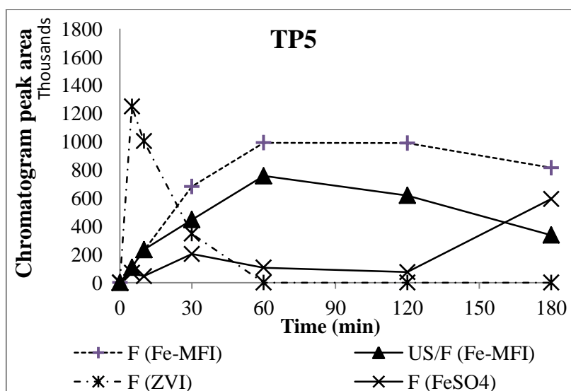
Figure 4.31. Evolution of TP5 concentration during heterogeneous Fenton-based processes (results of homogeneous Fenton reaction with ferrous iron salt were recalled for comparison purpose) ( \text{pH}_0 \text{ Fe-MFI} = 4.3 ; \text{pH}_0 \text{ ZVI} = 3.5 ; \text{pH}_0 \text{ FeSO}_4 = 2.6 )
