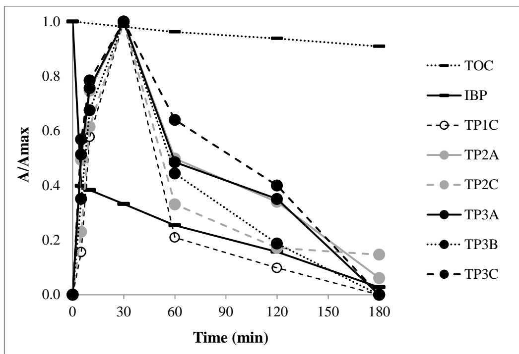
Figure 3.29. Evolution of normalized* concentration of hydroxylated IBP compounds during homogeneous Fenton reaction (*based on the maximum peak area measured for each compound)
