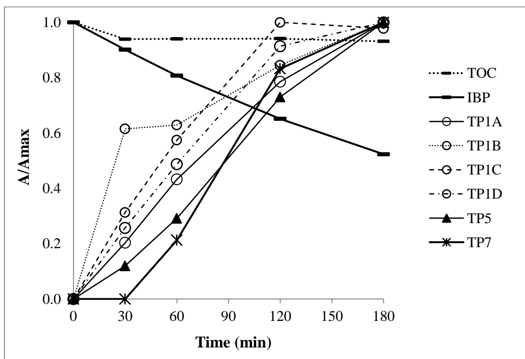
Figure 3.27. Evolution of normalized* concentration of IBP transformation products during US (*based on the maximum peak area measured for each compound)
