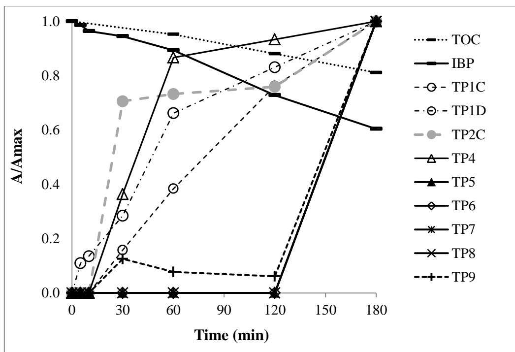
Figure 3.28. Evolution of normalized* concentration of IBP transformation products during UV-photolysis with LP Hg lamp (*based on the maximum peak area measured for each compound)
