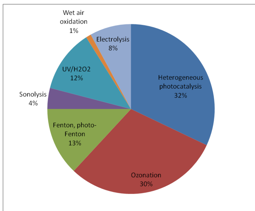
Figure 1.3. Distribution of studies on pharmaceuticals removal by AOPs (adapted from reference [37])
