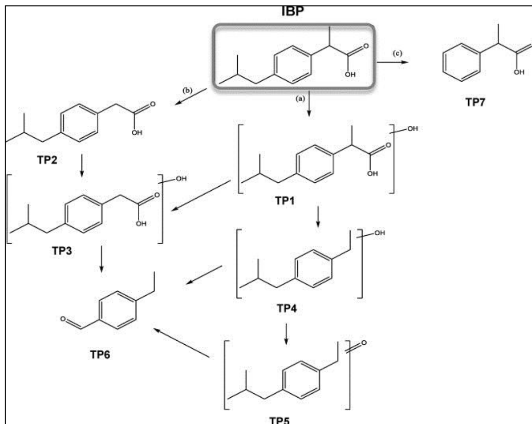
Figure 1.4. Possible transformation pathways of IBP during TiO_2 photocatalysis under UV-A and simulated solar irradiation, and sono-photocatalysis (adapted from reference [52])
