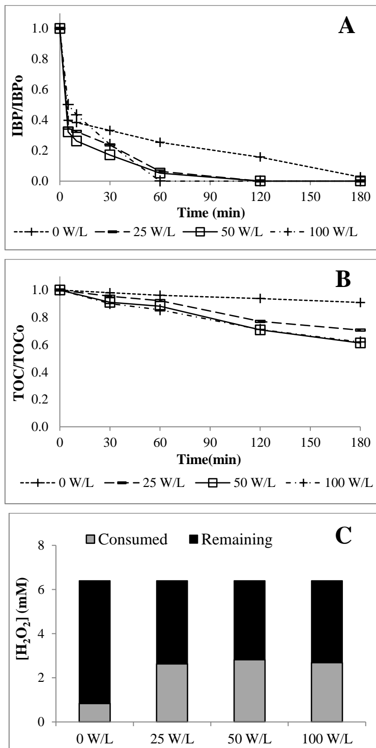
Figure 3.20. Effect of D_{US} on sono-Fenton oxidation of IBP: (A) IBP and (B) TOC concentration-time profiles ([IBP] 0 = 20 mg/L, pH 0 = 2.6, T = 25°C, f_{US} = 20 kHz, D_{US} = 25-100 W/L, [H 2 O 2 ] 0 = 6.4 mM, [Fe 2+ ] 0 = 0.134 mM). Fenton oxidation result is recalled for comparison purpose
