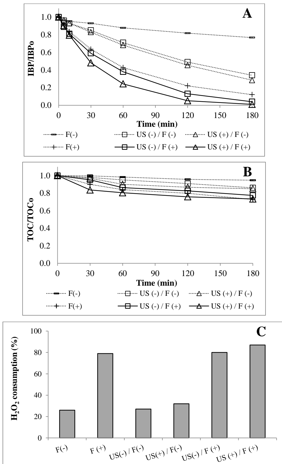
Figure 4.18. Effect of US density on Fenton oxidation with Fe/MFI: evolution of (A) IBP and (B) TOC concentration, and (C) H 2 O 2 consumption ([IBP] 0 = 20 mg/L, pH 0 = 4.3, T = 25°C, [H 2 O 2 ] 0 = 6.4 mM, [Fe-MFI] = 1 and 4.8 g/L, D US = 50 – 100 W/L, f US = 20 kHz)
