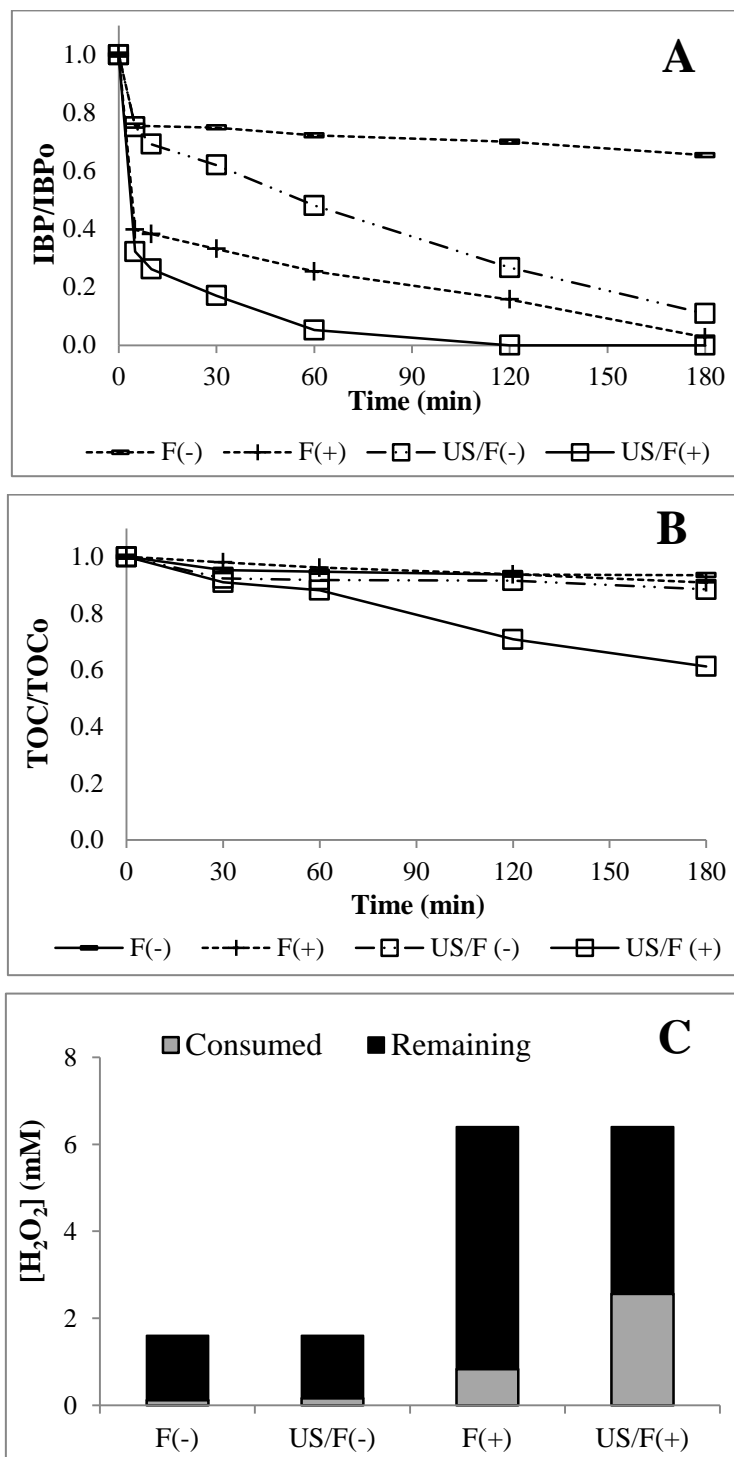
Figure 3.18. Fenton (F) and sono-Fenton oxidation (US/F) of IBP: (A) IBP and (B) TOC concentration-time profiles, and (C) H 2 O 2 consumption ([IBP] 0 = 20 mg/L, pH 0 = 2.6, T = 25°C, f US = 20 kHz, D US = 50W/L, F(-): [Fe 2+ ] 0 = 0.033 mM and [H 2 O 2 ] 0 = 1.6 mM, (+): [Fe 2+ ] 0 = 0.134 mM and [H 2 O 2 ] 0 = 6.4 mM)
