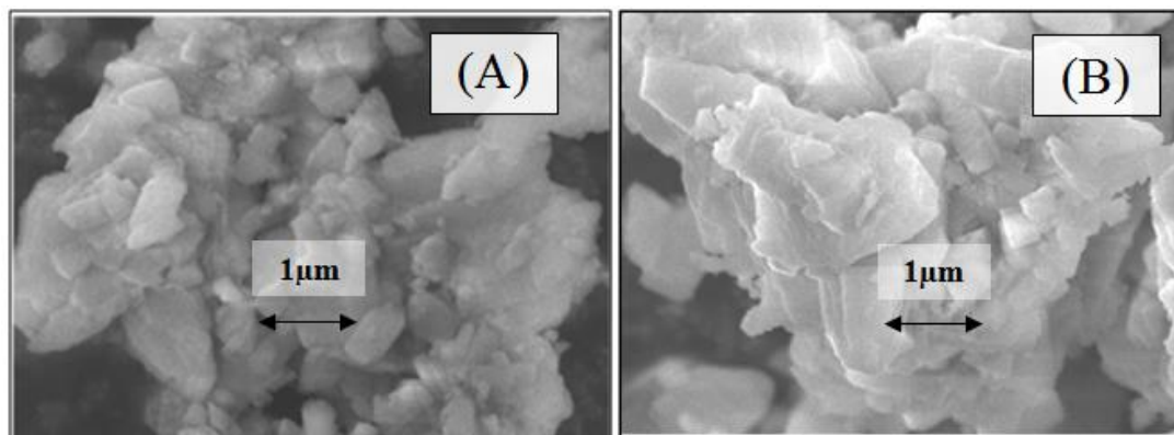
Figure 4.4. SEM images of (A) fresh and (B) used Fe-MFI catalyst after Fenton oxidation
