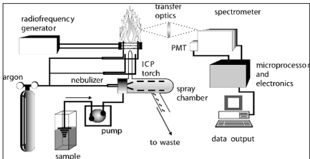
Figure 2.5. Schematic diagram of ICP-AES apparatus (adapted from reference [215])
