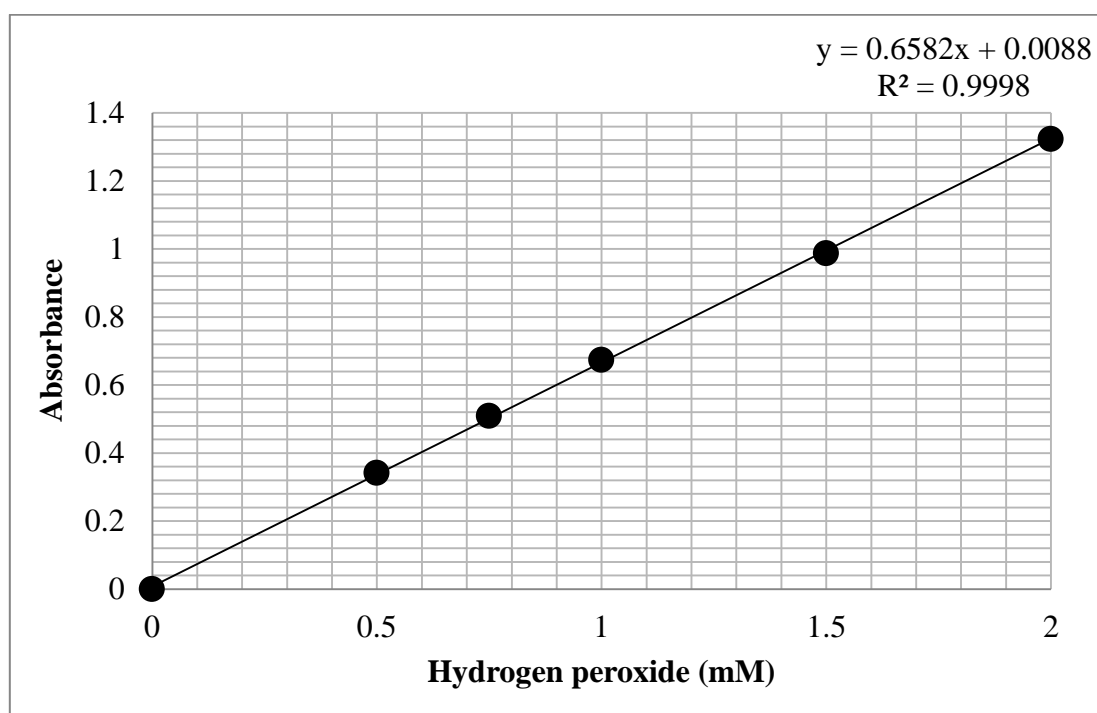
Figure V. Calibration curve of hydrogen peroxide ( \text{H}_2\text{O}_2 )
