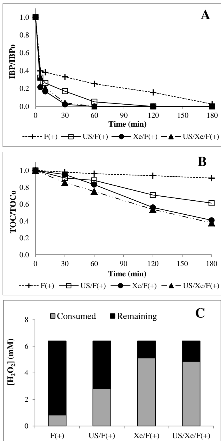
Figure 3.25. Comparison of sono-photo-Fenton and other Fenton-related processes, for high reagent concentration: (A) IBP and (B) TOC concentration-time profiles, and (C) H 2 O 2 consumption ([IBP] 0 = 20 mg/L, pH 0 = 2.6, T = 25°C, f US = 20 kHz, D US = 50 W/L, irradiated volume fraction = 1/3, lamp = 150 W Xe (Vis), [H 2 O 2 ] 0 = 6.4 mM and [Fe 2+ ] 0 = 0.134 mM)
