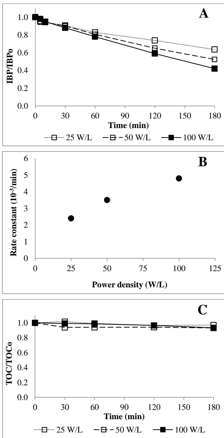
Figure 3.4. Effect of ultrasound density on IBP sonolysis: (A) IBP concentration-time profile, (B) first-order rate constant and (C) TOC concentration-time profile ( [IBP]_0 = 20 mg/L, pH_0 = 4.3 , T = 25^\circ C , f_{US} = 20 kHz, D_{US} = 25 - 100 W/L)
