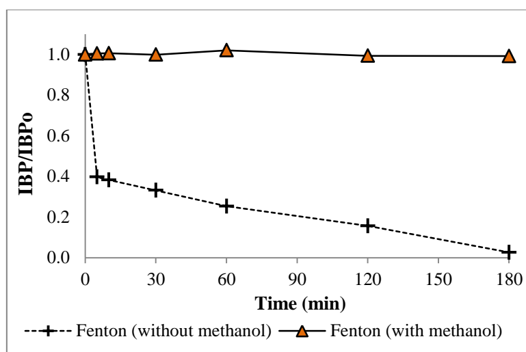
Figure 3.15. Effect of methanol on Fenton oxidation of IBP ([IBP] 0 = 20 mg/L, pH 0 = 2.6, T = 25°C, [Fe 2+ ] 0 = 0.134 mM, [H 2 O 2 ] 0 = 6.4 mM, [MeOH] 0 = 50 mM)
