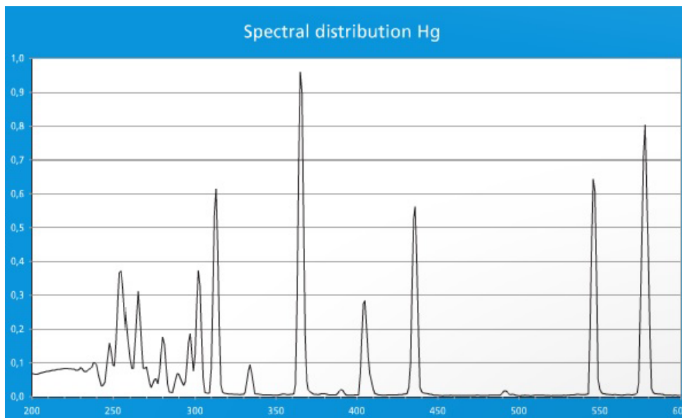
Figure 2.21. Spectral distribution of TQ150 lamp (medium pressure Hg vapor lamp) (Data provided by supplier)
