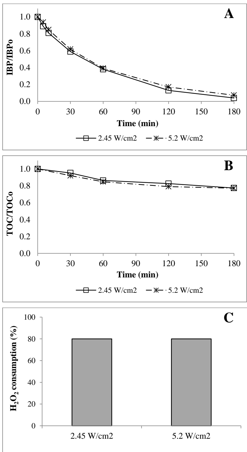
Figure 4.17. Effect of US intensity on Fenton oxidation with Fe-MFI: evolution of (A) IBP and (B) TOC concentration, and (C) H 2 O 2 consumption ([IBP] 0 = 20 mg/L, pH 0 = 4.3, T = 25°C, [H 2 O 2 ] 0 = 6.4 mM, [Fe-MFI] = 4.8 g/L, f US = 20 kHz, I US = 2.45 – 5.2 W/cm 2 )
