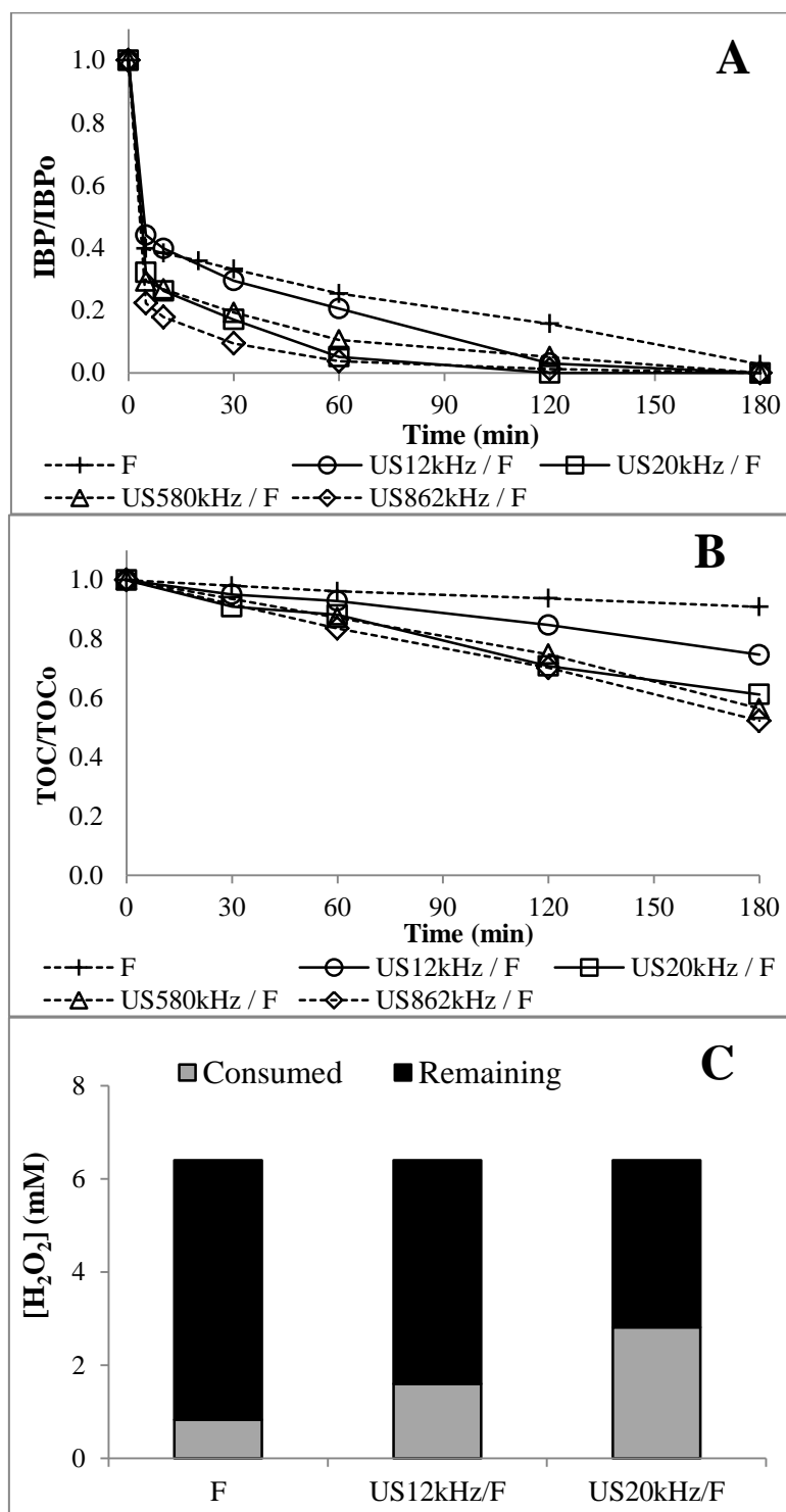
Figure 3.21. Effect of sonication frequency on sono-Fenton oxidation of IBP: (A) IBP and (B) TOC concentration-time profiles, and (C) H 2 O 2 consumption ([IBP] 0 = 20 mg/L, pH 0 = 2.6, T = 25°C, f US = 12-862 kHz, D US = 50W/L, [H 2 O 2 ] 0 = 6.4 mM, [Fe 2+ ] 0 = 0.134 mM). Fenton oxidation result is recalled for comparison purpose
