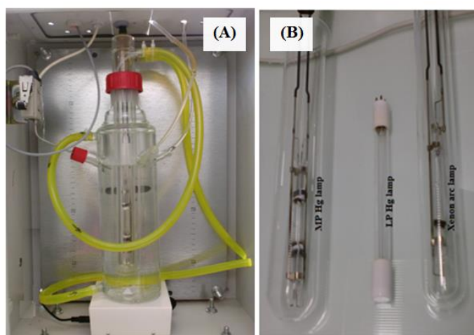
Figure 2.20. Photo-reactor (A) and investigated lamps (B)
