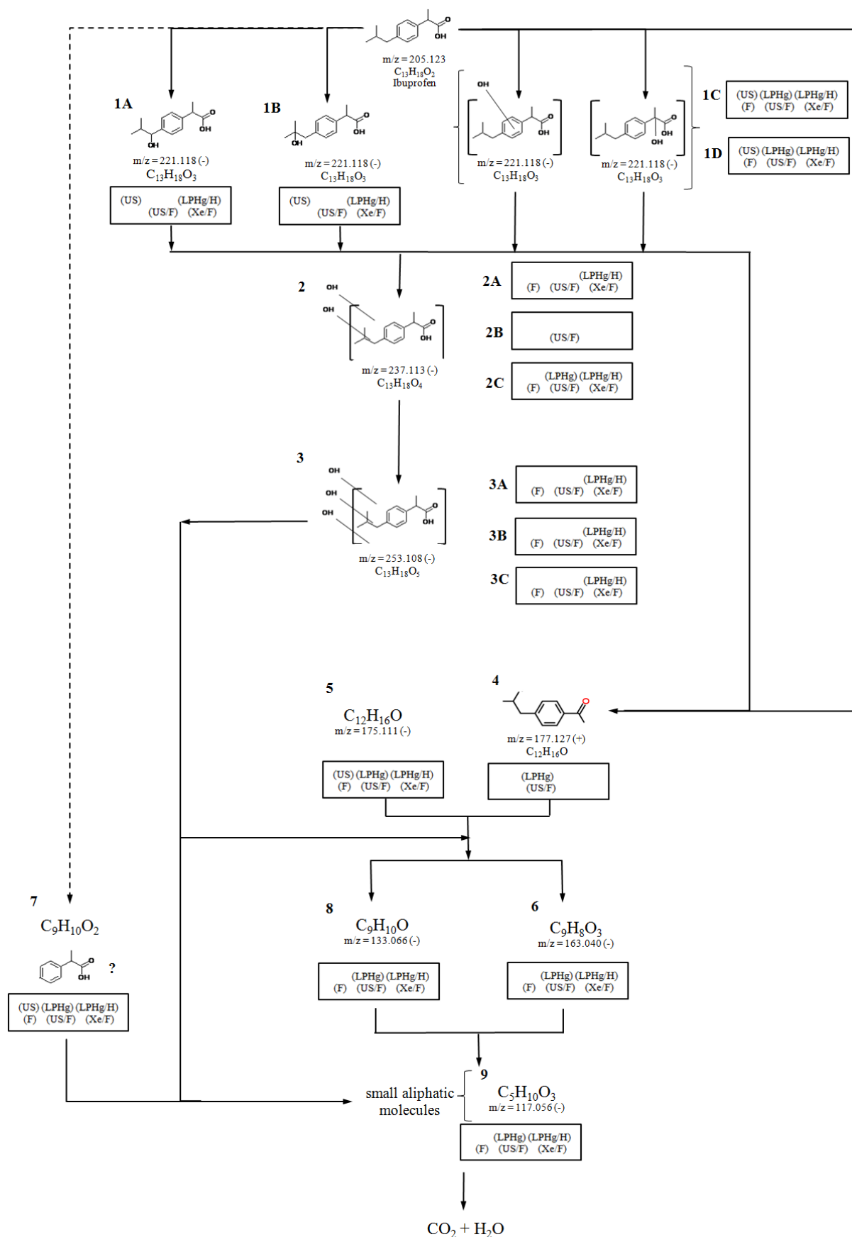
Figure 3.26. Proposed reaction scheme for degradation of ibuprofen by homogeneous AOPs
