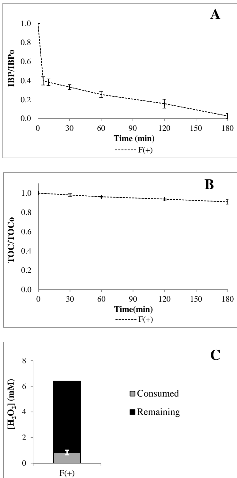
Figure VI. Example of experiment with error bars Degradation of IBP by Fenton oxidation: (A) IBP and (B) TOC concentration-time profiles, and (C) H 2 O 2 consumption ([IBP] 0 = 20 mg/L, pH 0 = 2.6, T = 25°C, [Fe 2+ ] 0 = 0.134 mM and [H 2 O 2 ] 0 = 6.4 mM)
