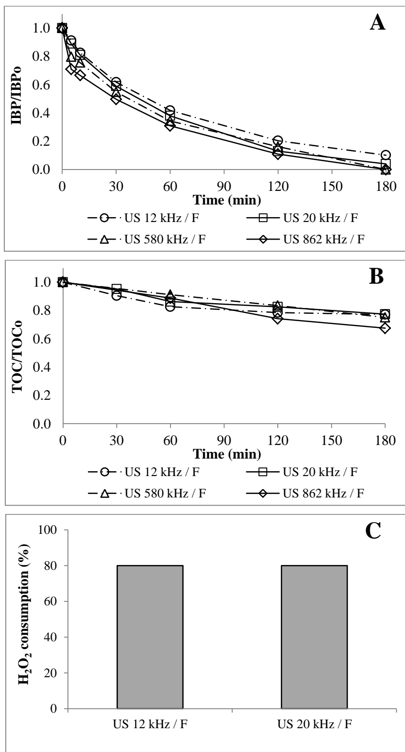
Figure 4.19. Effect of sound frequency on sono-Fenton oxidation with Fe-MFI: evolution of (A) IBP and (B) TOC concentration, and (C) H 2 O 2 consumption ([IBP] 0 = 20 mg/L, pH 0 = 4.3, T = 25°C, [H 2 O 2 ] 0 = 6.4 mM, [Fe-MFI] = 4.8 g/L, D US = 50 W/L, f US = 12 – 862 kHz)
