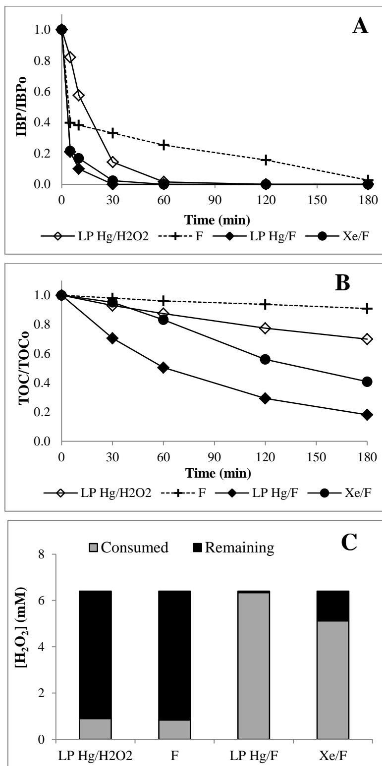
Figure 3.22. Effect of irradiation spectrum on photo-Fenton oxidation of IBP: (A) IBP and (B) TOC concentration-time profiles, and (C) H 2 O 2 consumption ([IBP] 0 = 20 mg/L, pH 0 = 2.6 (photo-Fenton) and 4.3 (LP Hg/H 2 O 2 ), T = 25°C, irradiated volume fraction = 1/3, lamp = 6W LP Hg or 150W Xe, [H 2 O 2 ] 0 = 6.4 mM and [Fe 2+ ] 0 = 0.134 mM). Fenton and LP Hg/H 2 O 2 oxidation results are recalled for comparison purpose
