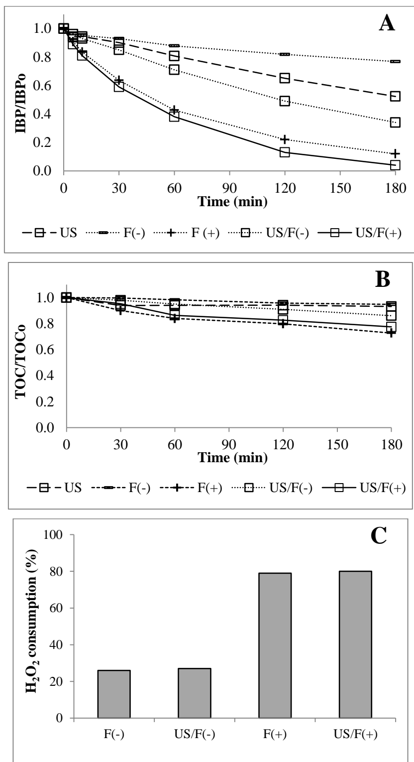
Figure 4.15. Comparison of Fenton and sono-Fenton oxidation with Fe-MFI: evolution of (A) IBP and (B) TOC concentration, and (C) H 2 O 2 consumption ([IBP] 0 = 20 mg/L, pH 0 = 4.3, T = 25°C, [H 2 O 2 ] 0 = 6.4 mM, [Fe-MFI] = 1 and 4.8 g/L, f US = 20 kHz, D US = 50 W/L)
