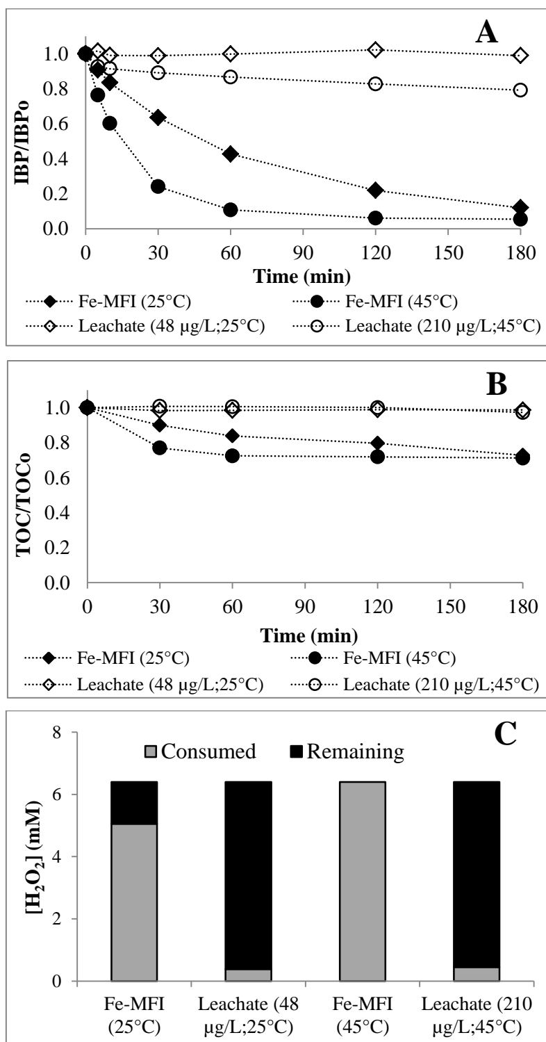
Figure 4.13. Activity of leachate for Fenton oxidation: evolution of (A) IBP and (B) TOC concentration, and (C) H 2 O 2 consumption ([IBP] 0 = 20 mg/L, [Fe-MFI] = 4.8 g/L, [Fe] leachate = 48 µg/L (25°C) and 210 µg/L (45°C), [H 2 O 2 ] 0 = 6.4 mM, pH 0 Fe-MFI* = 4.3, pH 0 leachate = 3.2, T = 25°C and 45°C) (*before contact). Corresponding Fenton oxidations were recalled for comparison
