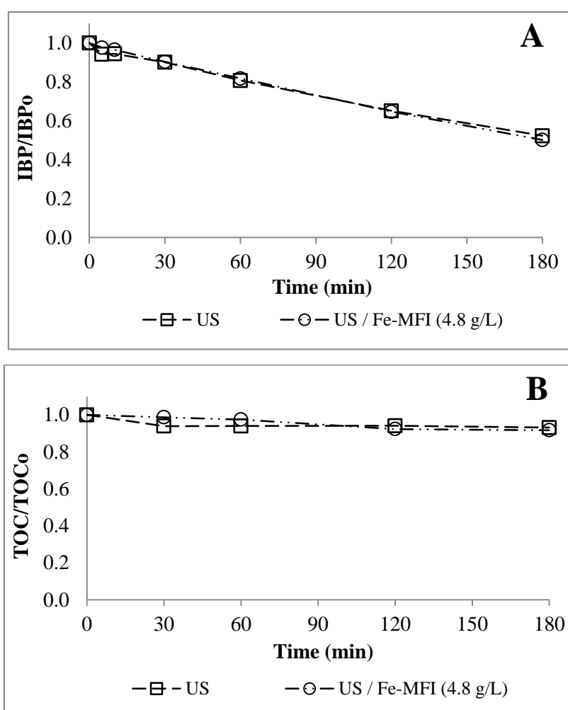
Figure 4.14. Effect of Fe-MFI on sonolysis: evolution of (A) IBP and (B) TOC concentration. ([IBP] 0 = 20 mg/L, [Fe-MFI] = 4.8 g/L, pH 0 = 4.3, T = 25°C, f US = 20 kHz, D US = 50 W/L)
