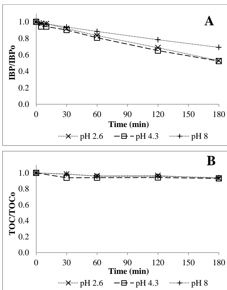
Figure 3.3. Effect of the solution pH on: (A) IBP and (B) TOC removal by sonolysis ([IBP] 0 = 20 mg/L, pH 0 = 2.6 – 8, T = 25°C, f US = 20 kHz, D US = 50 W/L)
