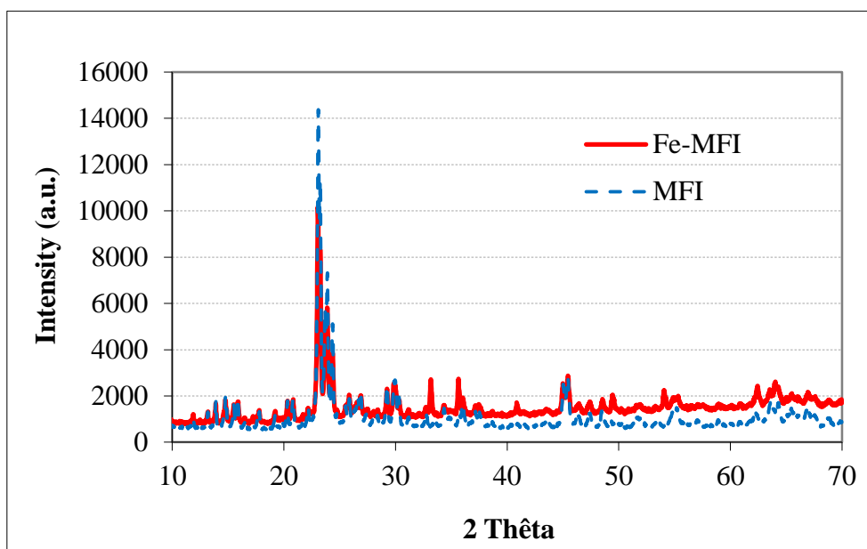
Figure 2.13. XRD patterns of fresh Fe-MFI and MFI
