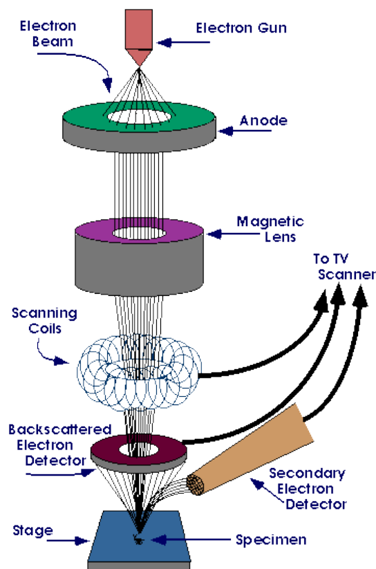
Figure 2.6. Schematic diagram of SEM (adapted from reference [216])
