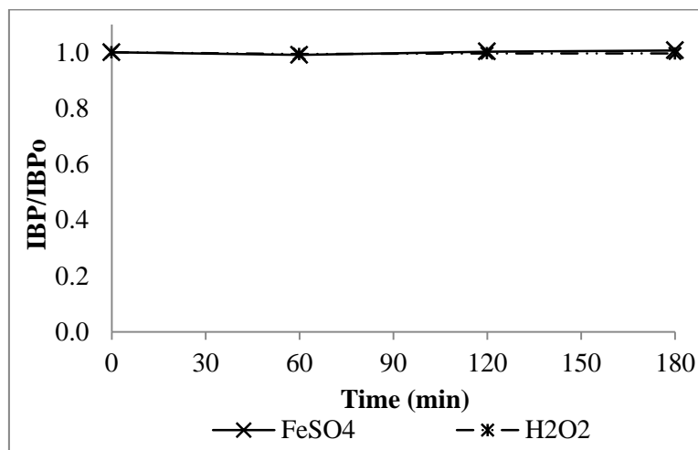
Figure 3.1. Effect of addition of H 2 O 2 (alone) or iron salt (without H 2 O 2 ) ([IBP] 0 = 20 mg/L, pH 0 = 2 – 8, T = 25°C, [FeSO 4 ·7H 2 O] 0 = 0.13 mM, [H 2 O 2 ] 0 = 6.4 – 22.4 mM)
