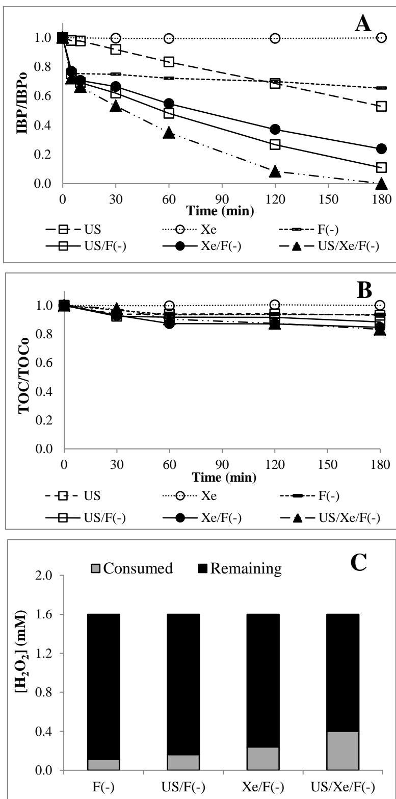
Figure 3.24. Comparison of sono-photo-Fenton and other Fenton-related processes, for low reagent concentration: (A) IBP and (B) TOC concentration-time profiles, and (C) H 2 O 2 consumption. ([IBP] 0 = 20 mg/L, pH 0 = 2.6, T = 25°C, f US = 20 kHz, D US = 50W/L, irradiated volume fraction = 1/3, lamp = 150W Xenon, [H 2 O 2 ] 0 = 1.6 mM and [Fe 2+ ] 0 = 0.033 mM)
