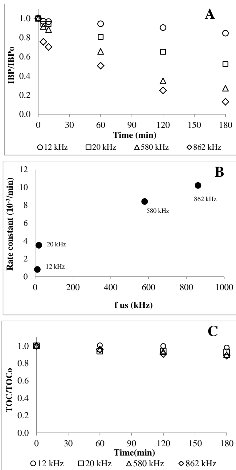
Figure 3.5. Effect of sonication frequency on IBP sonolysis: (A) IBP concentration-time profile, (B) first-order rate constant, (C) TOC concentration-time profile ([IBP] 0 = 20 mg/L, pH 0 = 4.3, T = 25°C, f US = 12-862 kHz, D US = 50 W/L)
