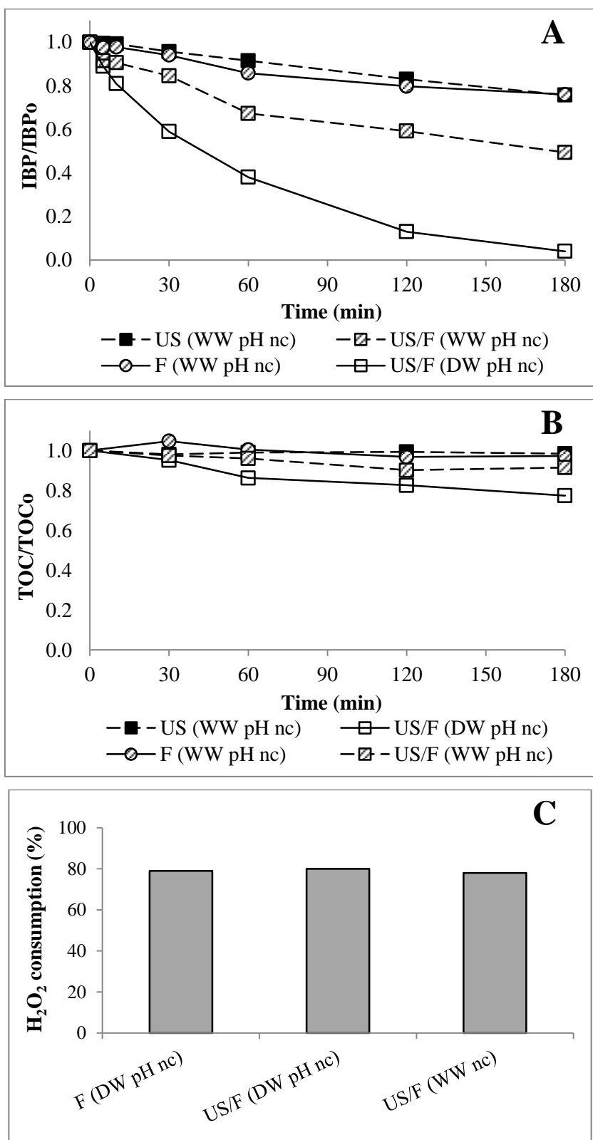
Figure 4.33. Effect of WW matrix on heterogeneous sono-Fenton process: evolution of (A) IBP and (B) TOC concentration, and (C) H 2 O 2 consumption ([IBP] 0 = 20 mg/L, [Fe-MFI] = 4.8 g/L, [H 2 O 2 ] 0 = 6.4 mM, pH nc: pH not controlled, T = 25°C, D US = 50 W/L, f US = 20 kHz)
