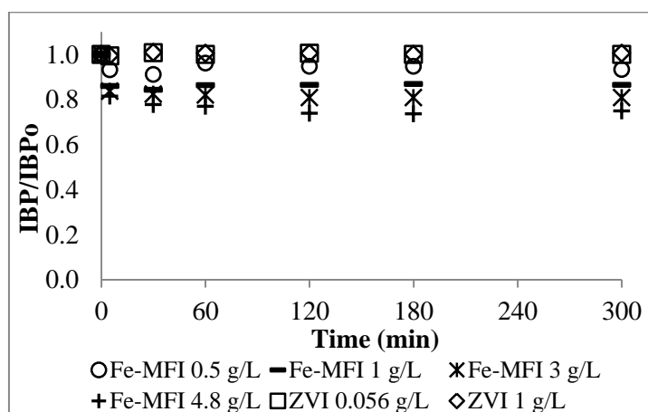
Figure 4.1. Adsorption of ibuprofen over ZVI and Fe-MFI catalysts ([IBP] 0 = 20 mg/L, [Fe-MFI] = 0.5 – 4.8 g/L, [ZVI] = 0.056 and 1 g/L, pH 0 = 4.3, T = 25°C)
