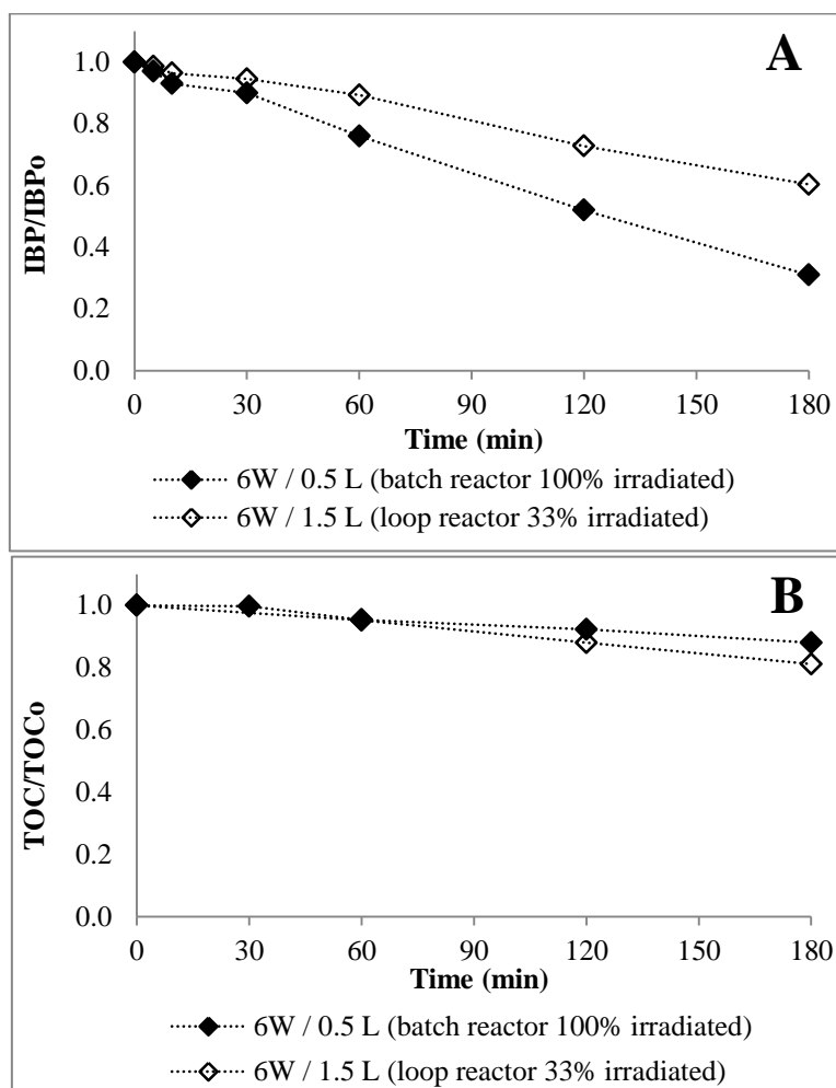
Figure 3.10. Effect of irradiated volume fraction on IBP photolysis: (A) IBP and (B) TOC concentration-time profiles ([IBP] 0 = 20 mg/L, pH 0 = 4.3, T = 25°C, irradiated volume = 500 mL, total volume = 500 and 1500 mL, lamp = 6W LP Hg)
