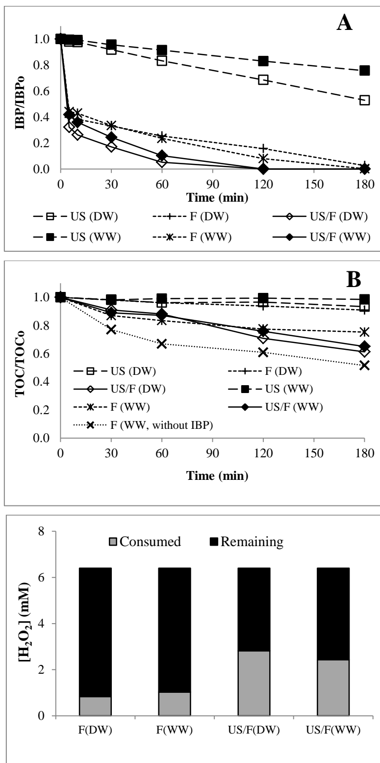
Figure 3.34. Effect of water matrix (DW: distilled water, WW: wastewater effluent) on sonolysis (US), Fenton (F) and sono-Fenton (US/F) oxidation of IBP: (A) IBP and (B) TOC concentration-time profiles, and (C) H 2 O 2 consumption.
