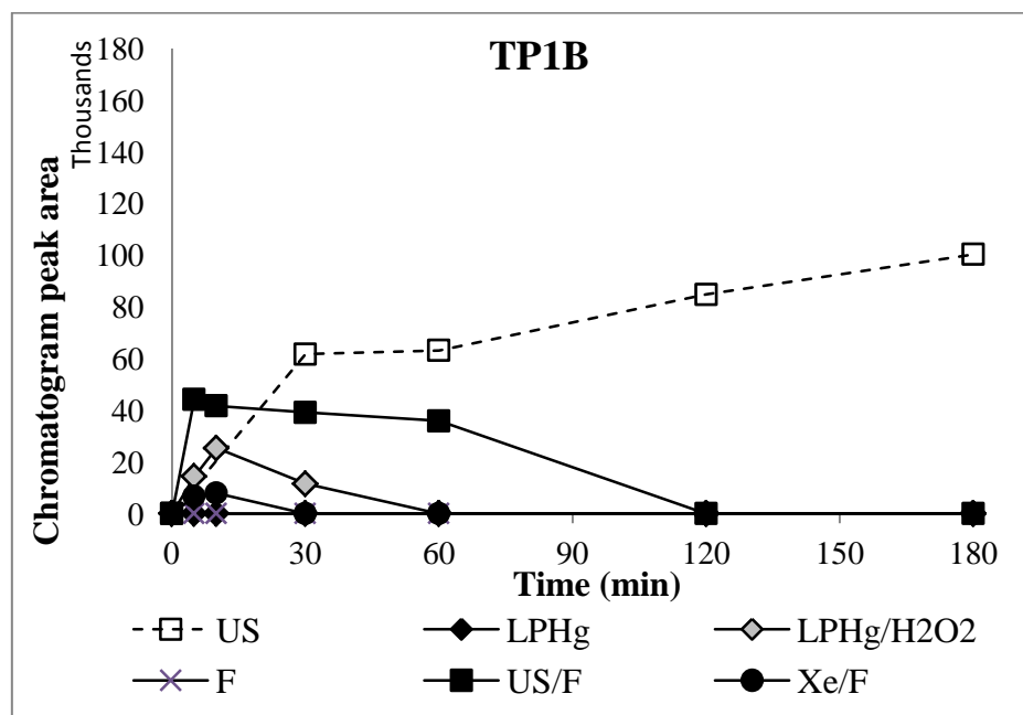
Figure 3.31. Evolution of TP1B concentration during homogeneous AOPs
