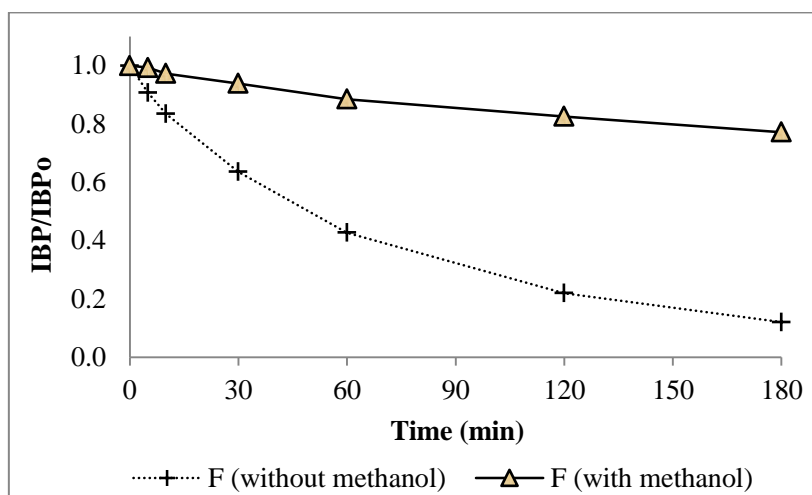
Figure 4.7. Effect of methanol on heterogeneous Fenton oxidation of IBP over Fe-MFI ([IBP] 0 = 20 mg/L, [Fe-MFI] = 4.8 g/L, [H 2 O 2 ] 0 = 6.4 mM, T = 25°C)
