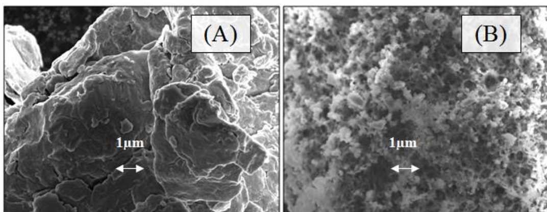
Figure 4.5. SEM images of (A) fresh and (B) used ZVI ( \text{pH}_0 = 3.5 )
