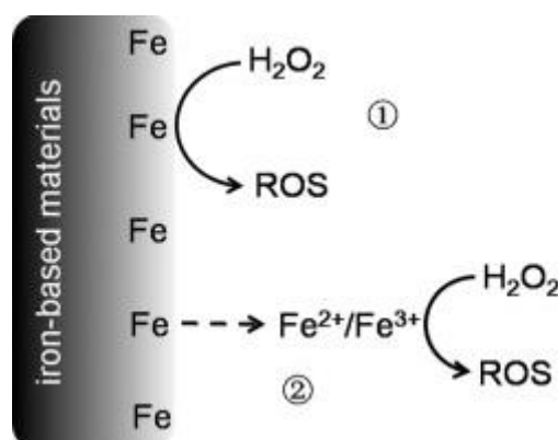
Figure 1.5. Schematic diagram of Fenton reaction using iron containing solids: (1) heterogeneous mechanism induced by iron surface species and (2) homogeneous mechanism induced by leached iron (adapted from reference [65])
