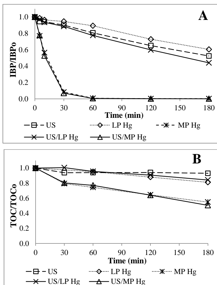
Figure 3.16. Sonophotolysis of IBP: (A) IBP and (B) TOC concentration-time profiles ([IBP] 0 = 20 mg/L, pH 0 = 4.3, T = 25°C, irradiated volume = 500 mL, total volume = 1500 mL, lamp = 6W LP Hg (UV) or 150W MP Hg (UV-Vis), f US = 20 kHz, D US = 50W/L)
