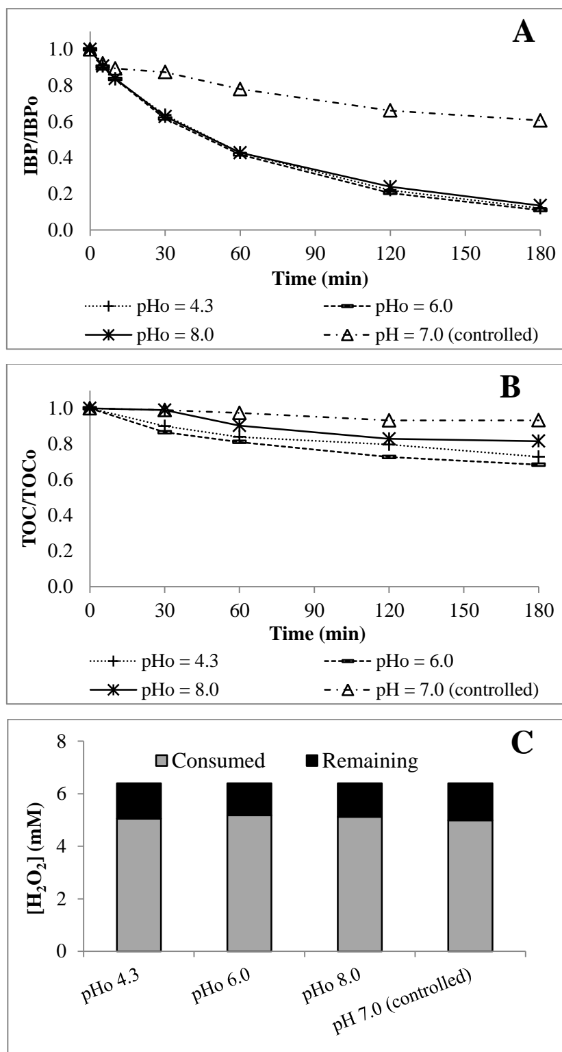
Figure 4.12. Effect of pH on Fenton oxidation over Fe-MFI: evolution of (A) IBP and (B) TOC concentration, and (C) H 2 O 2 consumption ([IBP] 0 = 20 mg/L; [Fe-MFI] = 4.8 g/L, [H 2 O 2 ] 0 = 6.4 mM, pH 0 = 4.3-8 or pH controlled at 7, T = 25°C)
