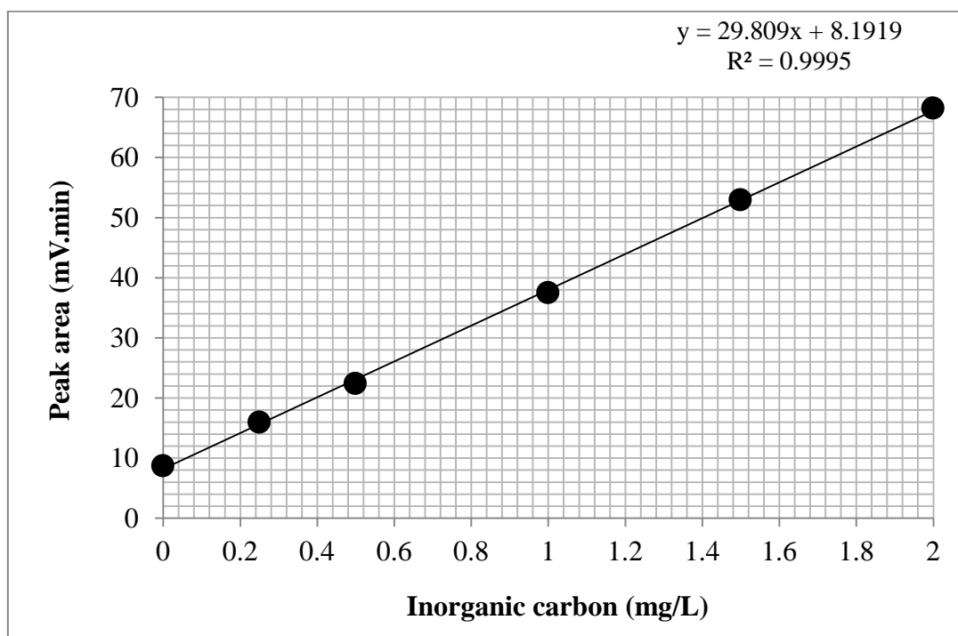
Figure IV. Calibration curve of inorganic carbon (IC)
