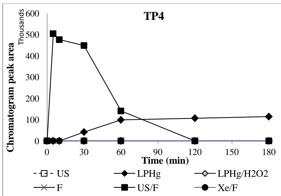
Figure 3.32. Evolution of TP4 concentration during homogeneous AOPs
