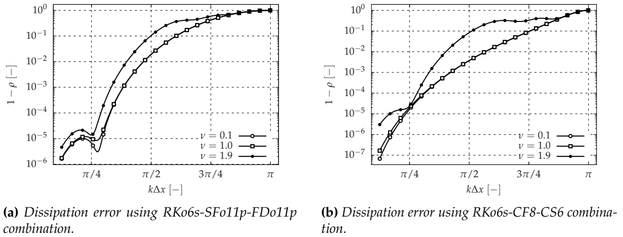
Fig. 9.6. Effect of time integration on dissipation for the proposed FD schemes.
