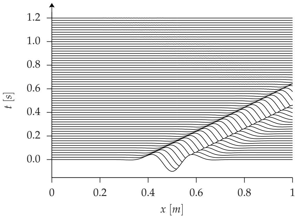
(b) kh = \frac{\pi}{20} .
