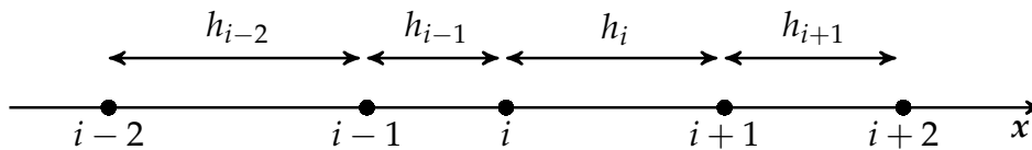
Fig. 8.1. Stencil for the third-order Successive Corrections Method (SCM3).
