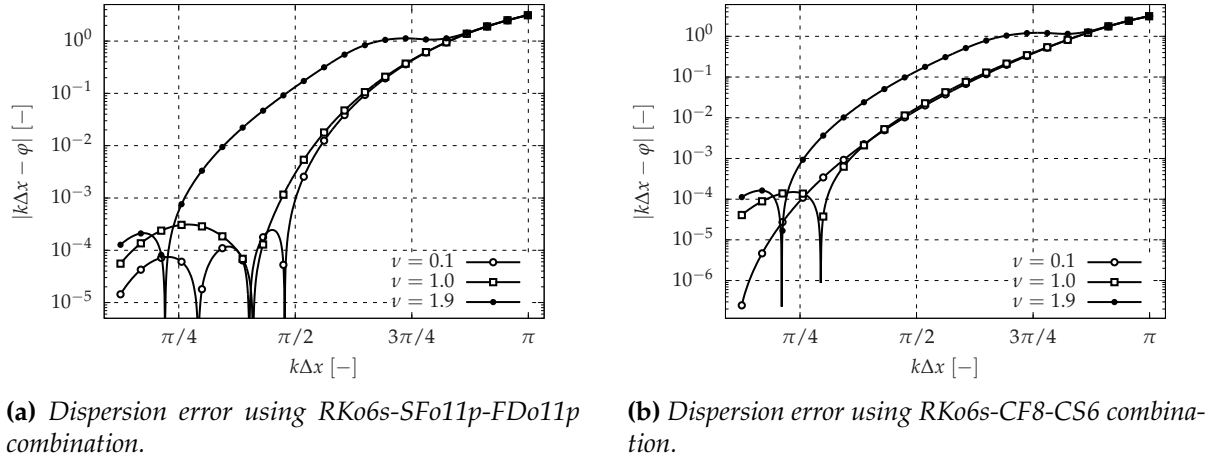
Fig. 9.5. Effect of time integration on dispersion for the proposed FD schemes.
