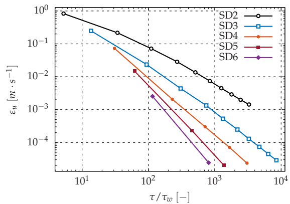
Fig. 1.3. \ell^2 -norm of the error \varepsilon_u of x -component of the velocity fluctuation versus the computational time. The test case deals with the convection of an isentropic compressible vortex (COVO).
