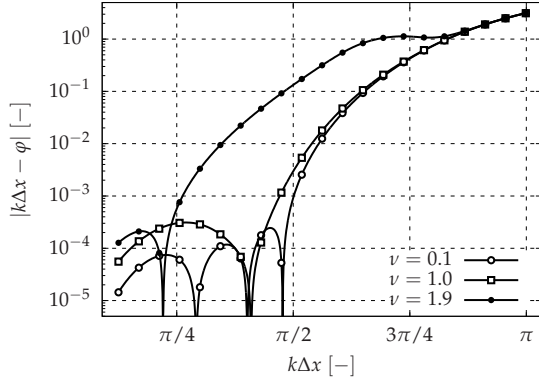
(a) Dispersion error using RK06s-SFo11p-FDo11p combination.
