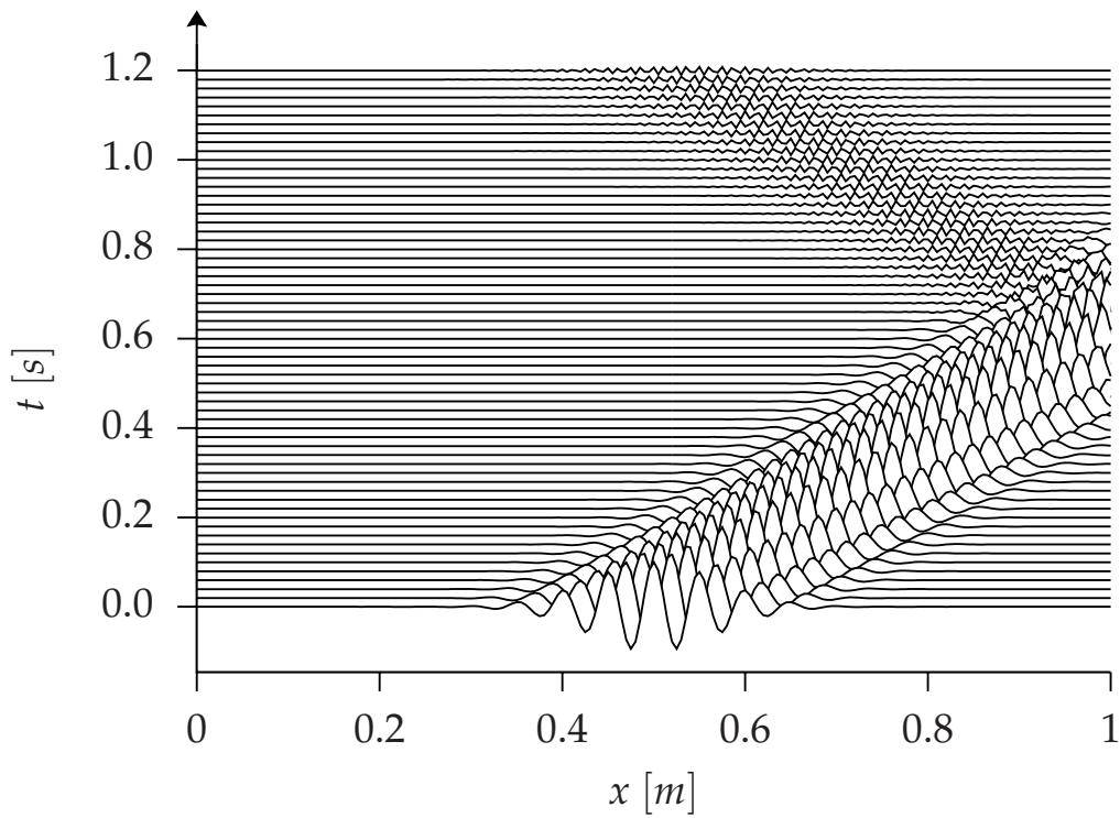
Fig. 3.2. Advection with Dirichlet boundary conditions.
