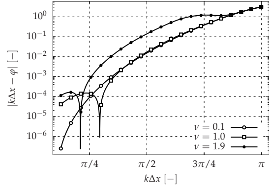
(b) Dispersion error using RK06s-CF8-CS6 combination.
