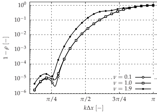
(a) Dissipation error using RK06s-SFo11p-FDo11p combination.
