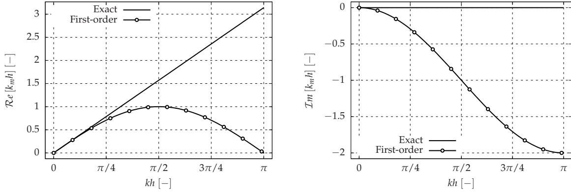
(a) Dispersion for the first-order upwind Finite Difference scheme.
