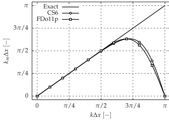
(a) Modified wavenumber for the sixth-order compact schemes CS6 and the fourth-order explicit schemes using 11 points FDo11p.
