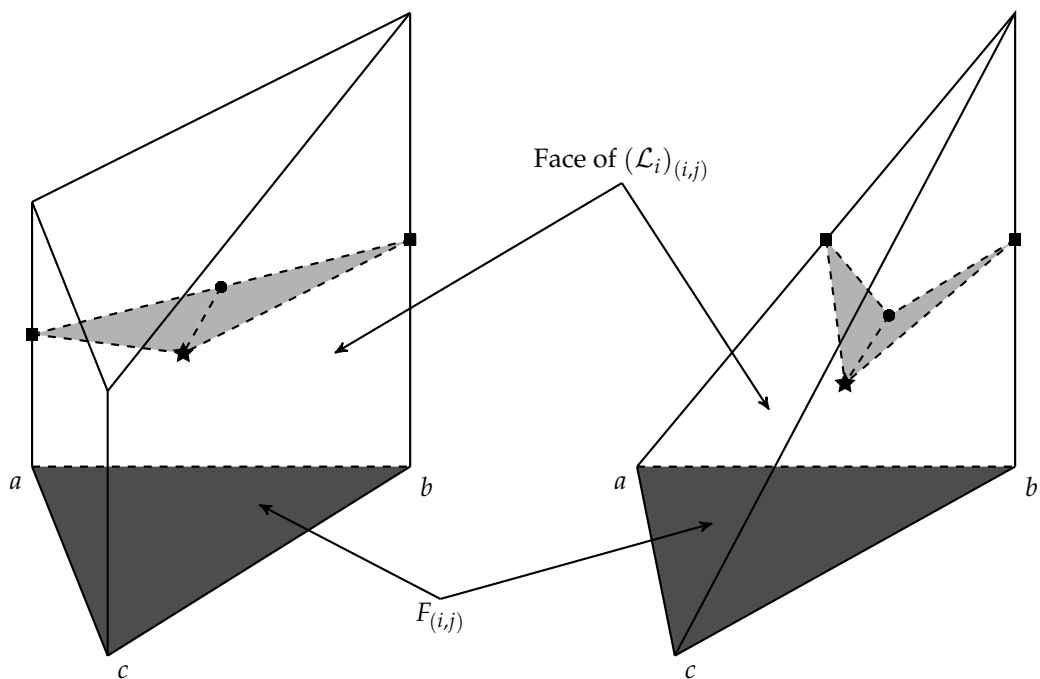
Fig. 7.10. Part of the dual cell for the face (a, b, c) of a prism and a tetrahedron. The (background) face of interest is dark gray and the facets of the dual cell are in light gray. The square symbol represent edge midpoint while the circle represent the face center and the star is the cell center.
