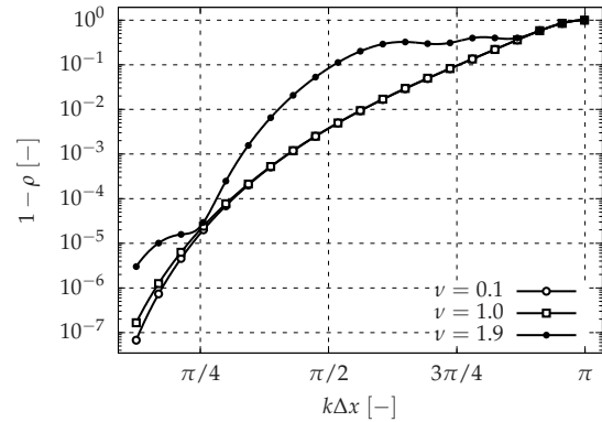
(b) Dissipation error using RK06s-CF8-CS6 combination.
