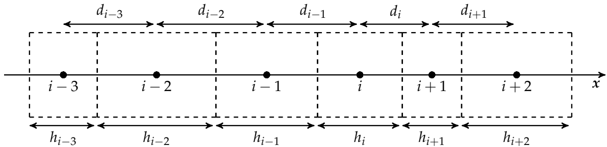
Fig. 8.2. Stencil for the third-order Successive Corrections Method (SCM3). The black dots are the cell centers. h_i is the size of cell i and d_i = (h_i + h_{i+1})/2 is the distance between the center of cell i and the center of cell i+1 .
