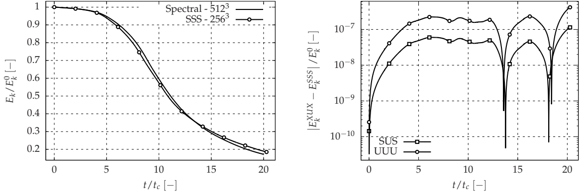
(a) The dimensionless kinetic energy for the SSS mesh. (b) The kinetic energy difference for the SUS and UUU meshes with respect to the SSS mesh.
