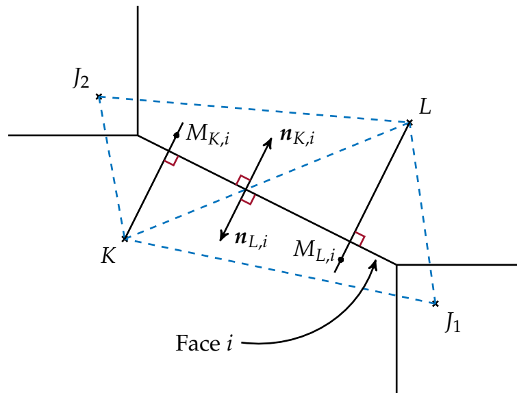
Fig. 7.3. Definition of M_{K,i} and M_{L,i} points. The rays [KM_{K,i}] and [LM_{L,i}] are orthogonal to the face i . M_{K,i} (resp. M_{L,i} ) belongs to the triangle KLJ_2 (resp. KLJ_1 ).
