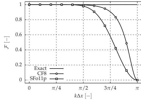
(b) Dissipation rate for the eighth-order compact filter CF8 and the sixth-order explicit filter using 11 points with \sigma_d = 1.0 SFo11p.
