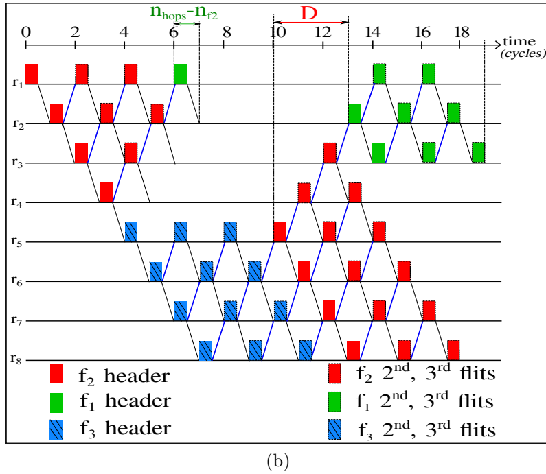
Figure 5.11: An example illustrating the case where n_{hops} > n_{f_j}
