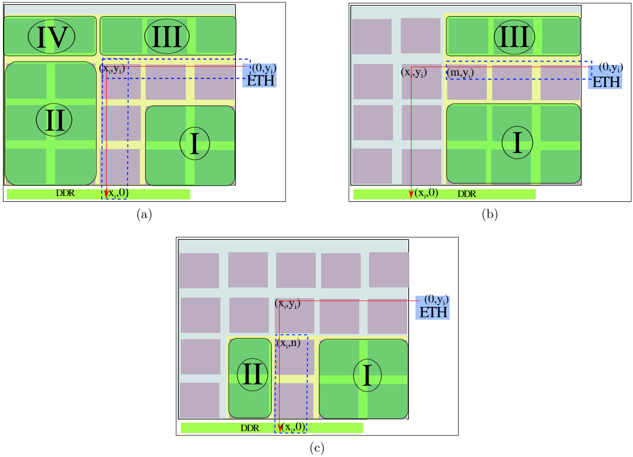
Figure 6.8: For each possible configuration of a critical path, the defined areas and their order in the tasks mapping.
