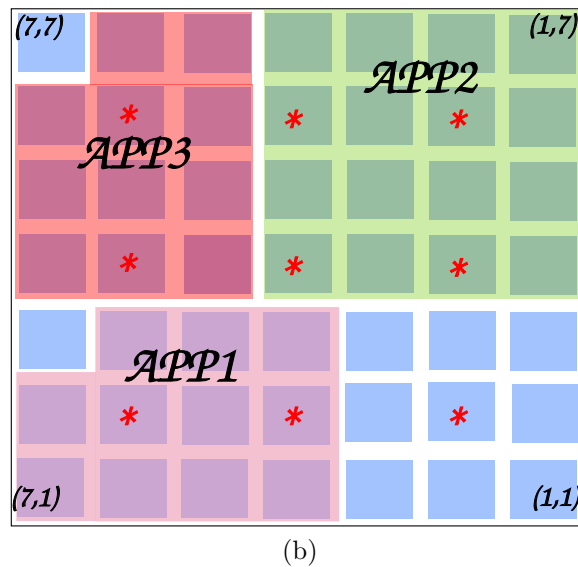
Figure 3.3: Allocating App_3 using SHiC method presented in[FDLP13].
