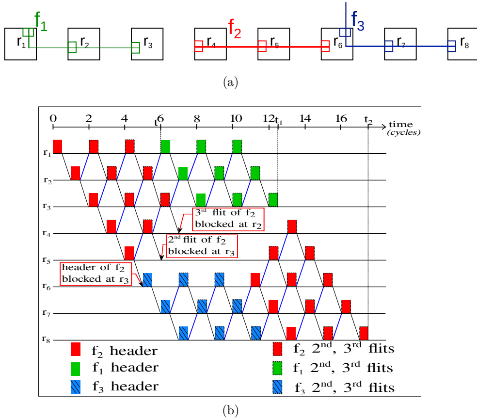
Figure 5.15: Transmission of flows f_1 , f_2 and f_3 of the case in Figure 5.14 where we consider a size of 3 flits for each packet.
