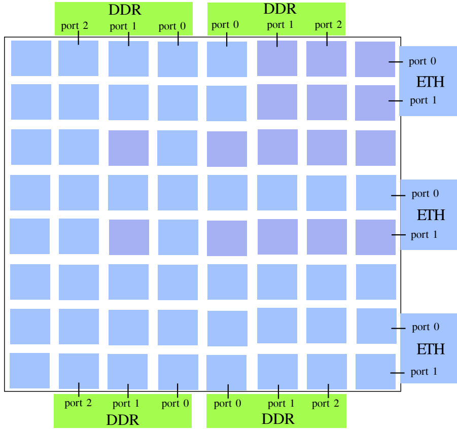
Figure 4.1: An overview of a Tiler architecture.
