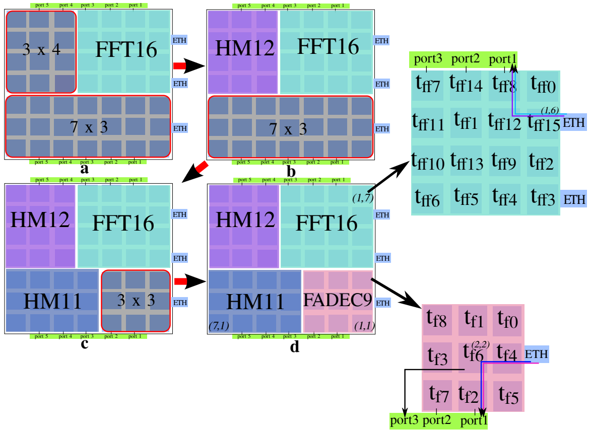
Figure 6.1: The different steps of our approach Map IO for mapping FADEC, HM and FFT applications of case study A.
