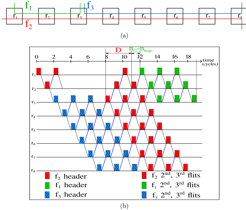
Figure 5.12: An example illustrating the case where n_{hops} < n_{f_2} .
