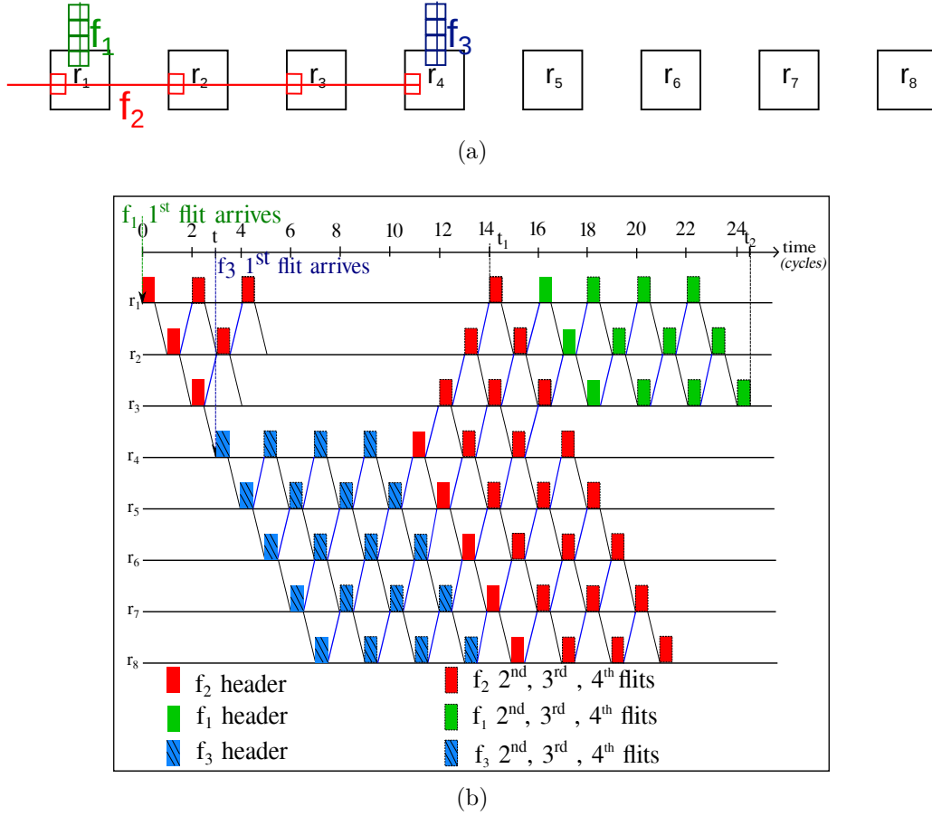
Figure 5.8: A worst-case scenario of the example in Figure 5.7 illustrating the recursion of Property 1.
