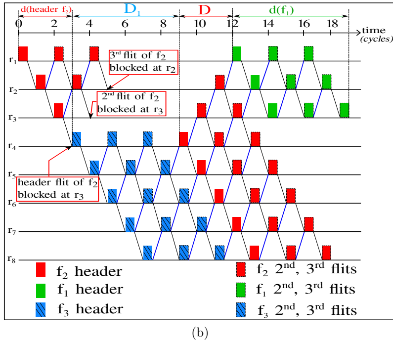
Figure 5.10: An example illustrating the case where n_{hops} = n_{f_j} .
