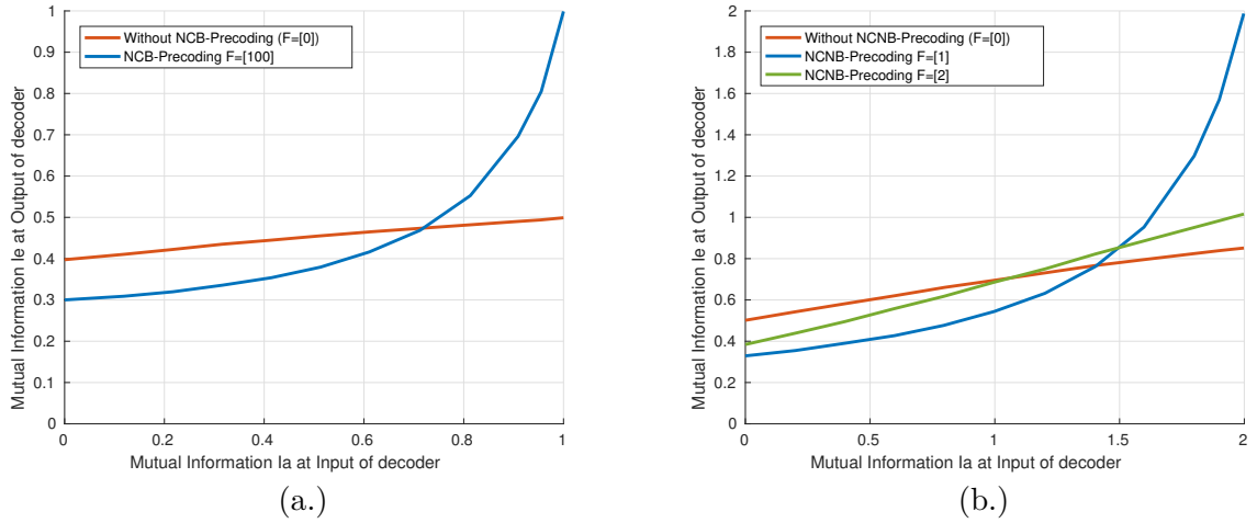
Figure 3.12: (a.) EXIT charts NCB-precoding CPMFSK h = 5/7 and M = 2 (b.) non-binary EXIT charts NCNB-precoding CPMFSK h = 3/4 and M = 4
