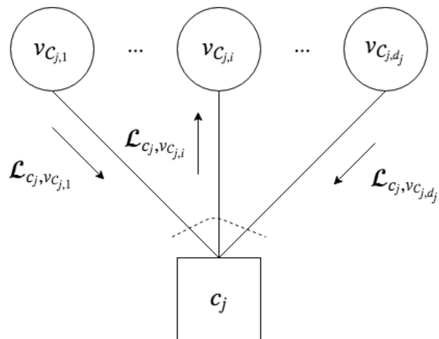
Figure 4.4: Check node update
