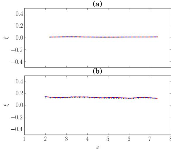
Figure IV.6: Comparison of external mass transfer coefficient for different Da . Red color corresponds to Da = 40 , blue color corresponds to Da = 200 and green color corresponds to Da = \infty . The dimensionless parameters are fixed to : a) Re = 50 , Sc = 10 , \alpha_s = 0.1 , and \gamma = 0.1 . b) Re = 10 , Sc = 10 , \alpha_s = 0.3 , and \gamma = 0.1 .
