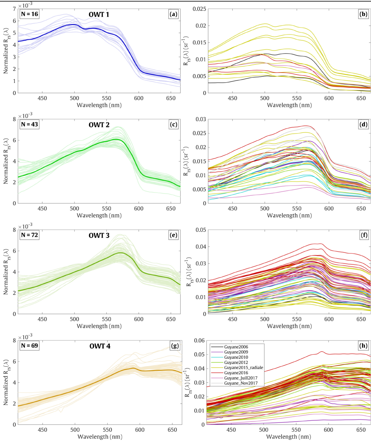
Figure 5.2. The left panels a-g ) show the normalized reflectance associated with the 4 optical OWTs defined from the in-situ dataset. The solid bold lines present the mean of the normalized R_{rs}(\lambda) . The right panels b-h ) show the raw reflectance for the corresponding OWTs with the colors indicating the names of conducted missions.
