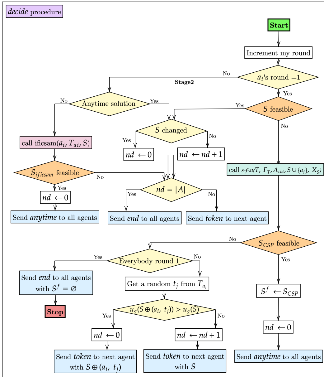
Figure 4.3: Decision process
