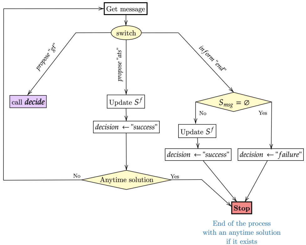
Figure 4.2: Global process
