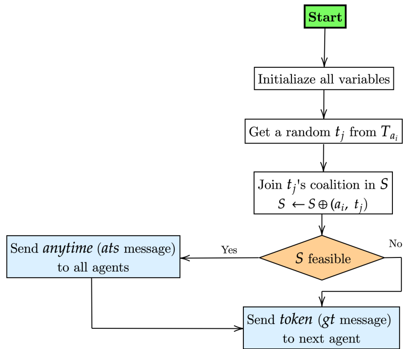
Figure 4.1: First agent process
