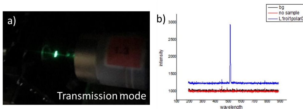
Fig.III.42 a) SHG in the irradiated sample probed by 1030nm fs laser with 100kHz, 0.1 \mu\text{J} . b) the spectra of the emitted green light (blue) and glycine background (black) and air (red)
