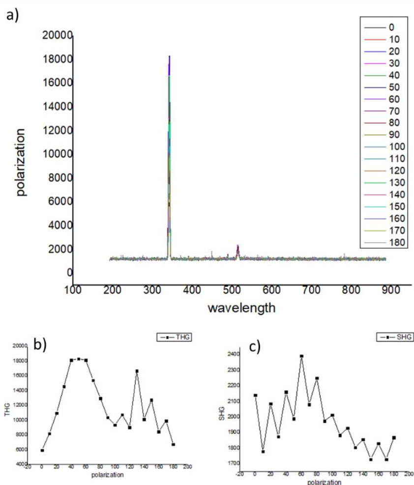
Fig.III.48 a) Spectra of alpha glycine with probe laser parameter: RR=100\text{kHz} , 0.2\mu\text{J} , polarization from 0-180 , 0^\circ is parallel with c axis. Acquisition parameters of spectrometer: exposure time 1s, average 1 time. b) and c) the THG and SHG intensity polarization dependence
