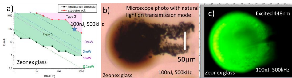
Fig.VI.3: Information related to luminescence collected from Zeonex sample a) the landscape including the experiment location at pulse energy= 0.1 \mu\text{J} – repetition rate 0.5 \text{MHz} , b) optical image in transmission with natural light, c) excitation wavelength at 448 \text{nm} , CCD detector sensitive in the visible.
