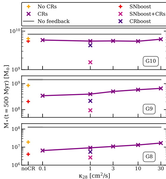
Figure 3.23: Stellar mass formed after 500 Myr for decreasing galaxy mass from top to bottom and increasing diffusion coefficient from left to right. The leftmost orange and red plus markers correspond to runs without CRs and with a fiducial and boosted SN feedback, respectively. Light purple crosses stand for runs with CRs and boosted SN feedback, and dark purple correspond to the simulations that have a SN energy injection into CRs of 40%. We show counterpart runs without feedback (no SN, no radiation, no CRs) in grey lines. The injection of more CR energy reduces star formation at any galaxy mass, and is more efficient than only boosting the SN feedback in G10.
