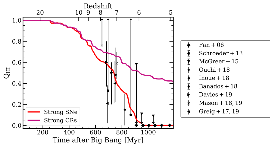
Figure 4.11: Time evolution of the volume-filling fraction of neutral gas with (in purple) and without (in red) CRs. We additionally show with black data points observational estimates from studies indicated in the legend. The reionisation history is drastically delayed with CRs, and the simulation volume is still composed of 42% of neutral hydrogen at z = 5 . With the Strong SNe model, the simulation volume is largely ionised by z = 5 , which is in much better agreement with the observational estimates.
