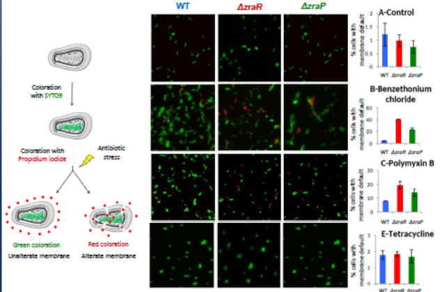
Fig 3 : Visualization of membrane default of the \Delta zraP , \Delta zraR mutants and WT strain in the presence of antibiotics. Fluorescence microscopy of cells stained with Syto9 and propidium iodide after exposure to drugs. More than 600 cells were counted. Representative fields are shown. Right panels (A-E-C-D): %number of red cells/ total number of cells.
