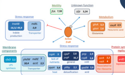
Fig 4 : The ZraR regulon identified using ChIP-Seq and RT-qPCR. Genes regulated by ZraR were grouped into categories according to their cellular function. The fold change, the ratio of gene expression of strain WT to strain \Delta zraR , is indicated for each gene.
