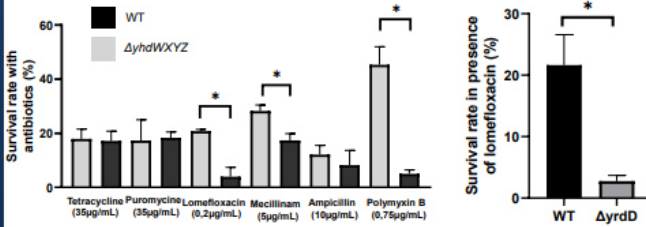
Fig 5 : Sensitivity of yhdW-Z and yrdD mutants to antibiotics. Survival ratio of the mutants were calculated as the ratio of survival percentages (WT/mutant). (*, p < 0.05). N = 4, Mann Whitney test.
