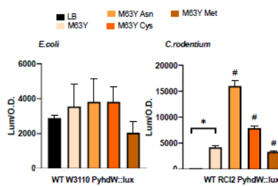
Figure 6 : Induction profile of yhdW in E.coli and C.rodentium strains in the presence of amino acids
