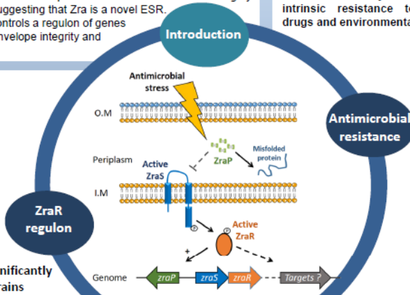
Fig 1 : ZraPSR signaling pathway
