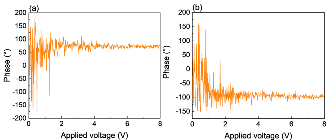
Figure 2.11: Piezoelectric phase responses corresponding to the voltage sweep on the (a) p^+ -domain of PPLN, and (b) on the p^- -domain of PPLN with the phase offset at +90 ^\circ .
