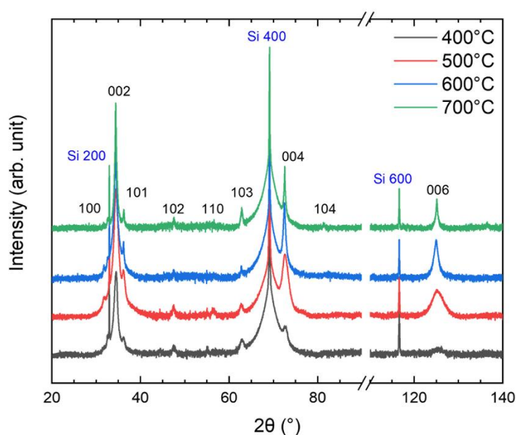
Figure 3.4: XRD patterns of ZnO deposits grown by PLI-MOCVD for a given growth temperature in the range of 400 – 700 °C. The intensity is plotted in logarithm scale.
