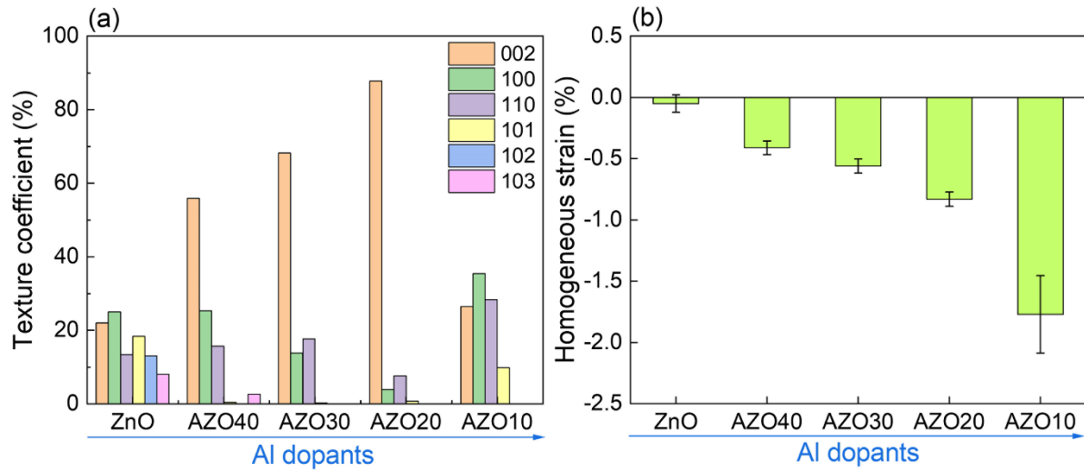
Figure 5.4: (a) The texture coefficients and (b) the mean homogeneous strain of AZO thin films grown by ALD as a function of Al doping concentration.
