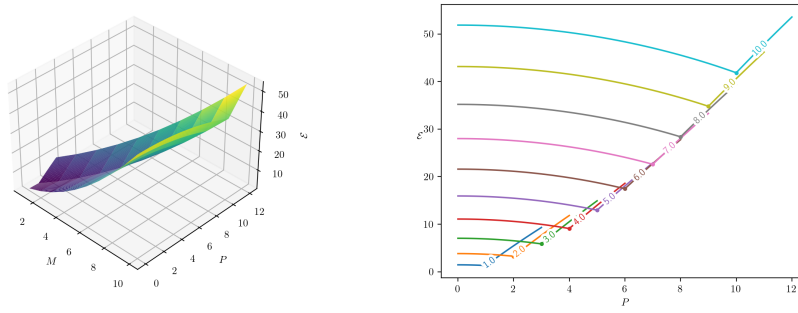
Figure 3.20 – Defocusing case with \theta = \pi .
