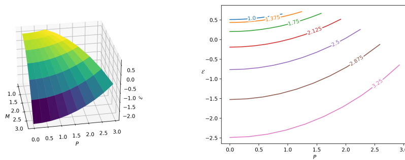
Figure 3.21 – Focusing case with a = -1 and \theta = \pi .
