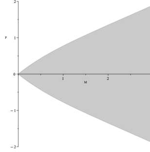
Figure 3.3 – Domain \tilde{D} .
