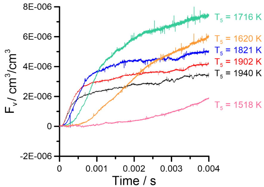
Figure A. 10 Soot volume fraction versus time of 0.07% C 7 H 8 in Argon for different temperatures
