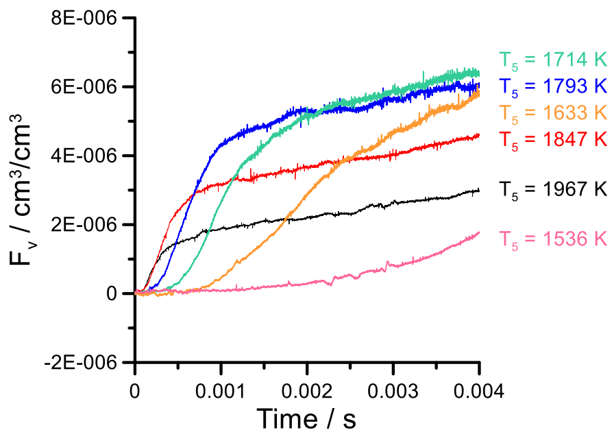
Figure A. 11 Soot volume fraction versus time of 0.08% C 6 H 6 in Argon for different temperatures
