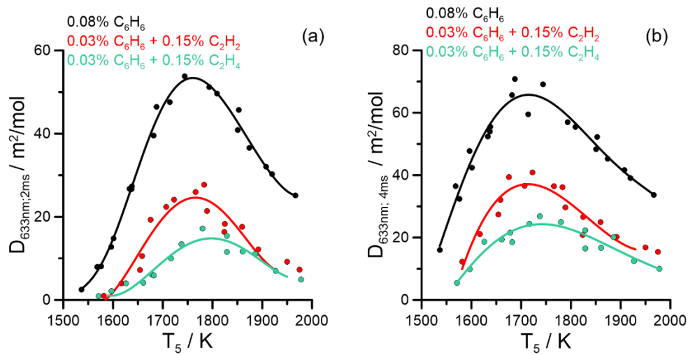
Figure 4.29 Dependence of the optical densities from the temperature - in black: 0.08% \text{C}_6\text{H}_6 in Argon, in red: 0.03% \text{C}_6\text{H}_6 + 0.15\% \text{C}_2\text{H}_2 in Argon, in green: 0.03% \text{C}_6\text{H}_6 + 0.15\% \text{C}_2\text{H}_4 in Argon; (a) at 2ms; (b) at 4ms
