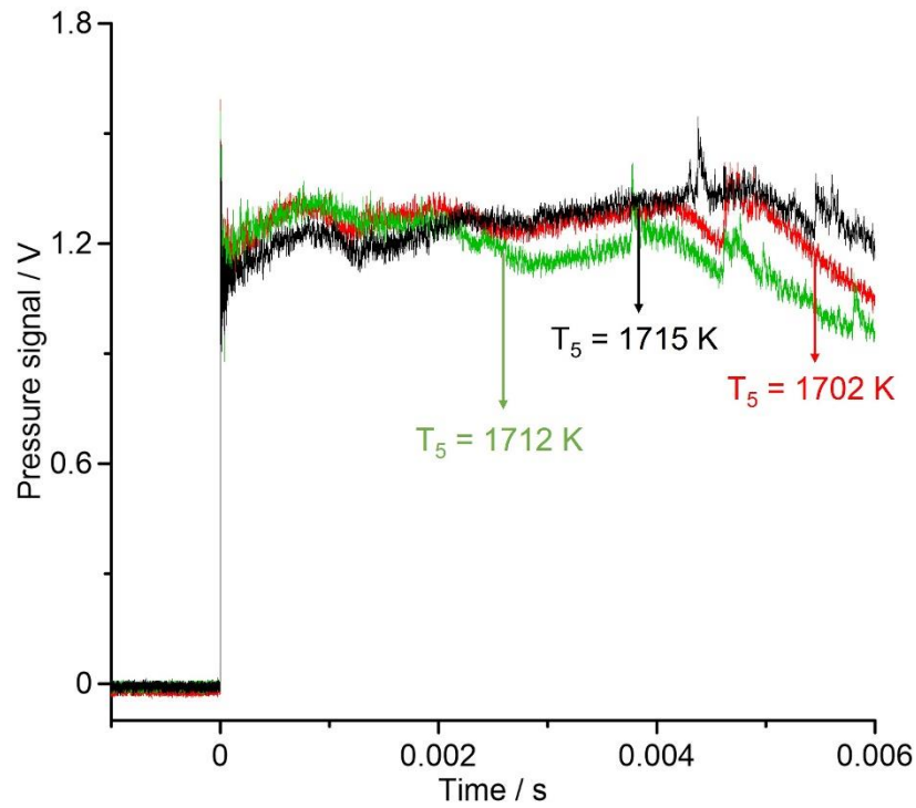
Figure 3.8 Pressure histories in the HPST behind reflected shocks of 0.1% C 7 H 8 diluted in Argon
