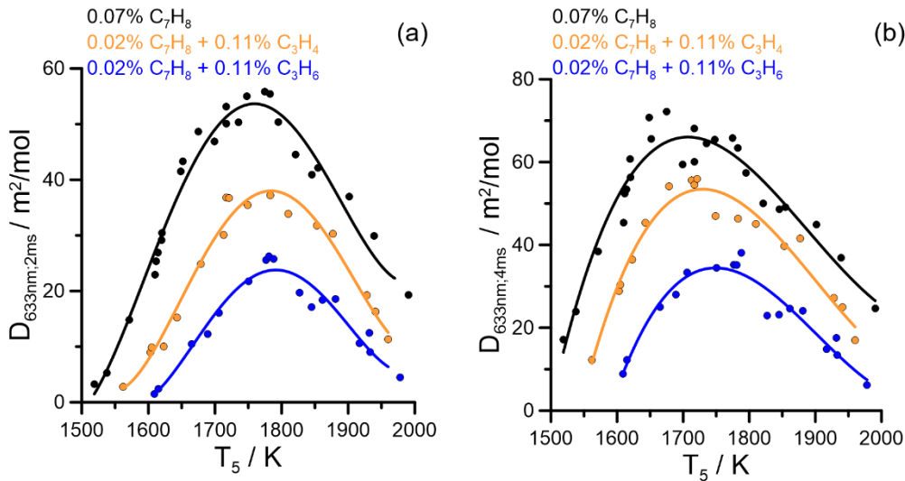
Figure 4.25 Dependence of the optical densities from the temperature – in black: 0.07% C 7 H 8 , in orange: 0.02% C 7 H 8 + 0.11% C 3 H 4 , in blue: 0.02% C 7 H 8 + 0.11% C 3 H 6 in Argon; (a) at 2ms; (b) at 4ms
