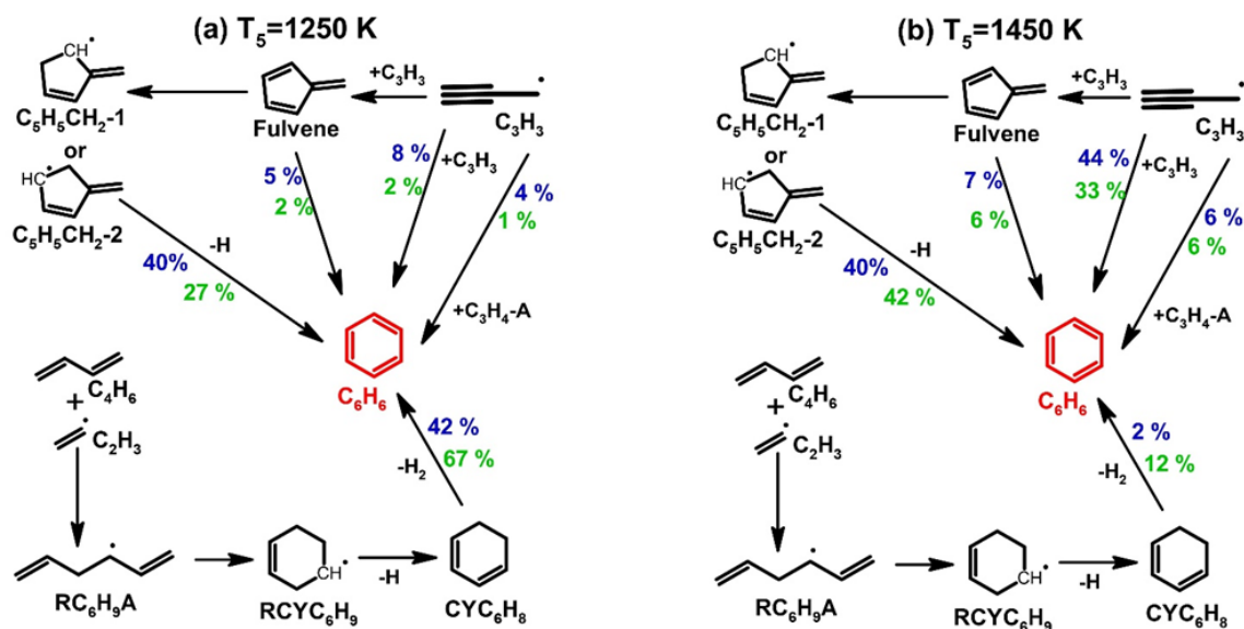
Figure 4.4 The reaction pathways leading to benzene formation at (a) T_5 = 1250\text{ K} , (b) T_5 = 1450\text{ K} in the pyrolysis of heptane. The percentage numbers (502 ppm heptane: blue normal; 2000 ppm heptane: green normal) represent the contributions to benzene formation
