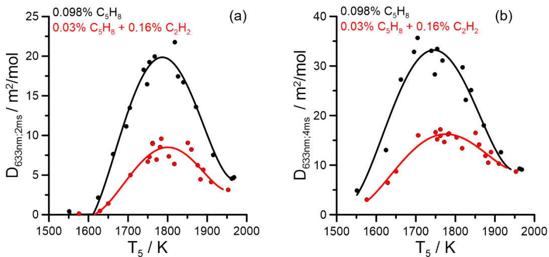
Figure 4.31 Dependence of the optical densities from the temperature - in black: 0.098% \text{C}_5\text{H}_8 in Argon, in red: 0.03% \text{C}_5\text{H}_8 + 0.16\% \text{C}_2\text{H}_2 in Argon; (a) at 2ms; (b) at 4ms
