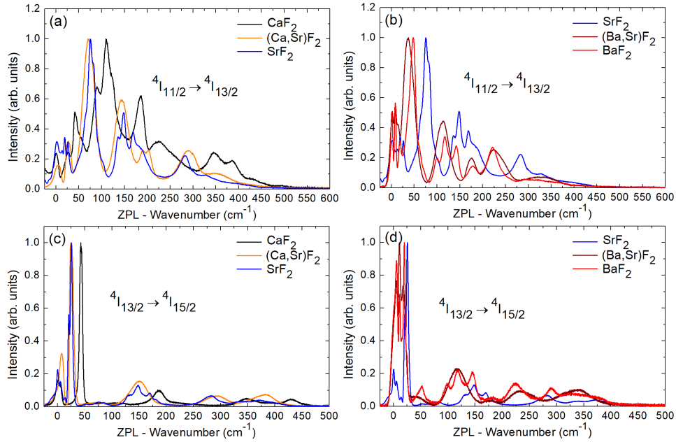
Figure IV.7: (a-d) LT (12 K) luminescence spectra of \text{Er}^{3+} ions in fluorite-type crystals: (a,b) the {}^4I_{11/2} \rightarrow {}^4I_{13/2} transition; (c,d) {}^4I_{13/2} \rightarrow {}^4I_{15/2} transition. ZPL – zero-phonon-line energy.
