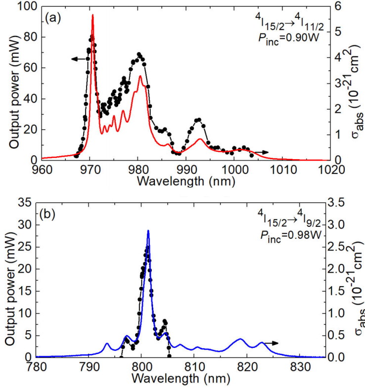
Figure IV.40: Laser excitation curves for the mid-infrared \text{Er}^{3+}:\text{KY}_3\text{F}_{10} laser for pumping: (a) into the ^4\text{I}_{11/2} state, (b) into the ^4\text{I}_{9/2} state. The absorption cross-section, \sigma_{\text{abs}} , spectra are shown for comparison.
