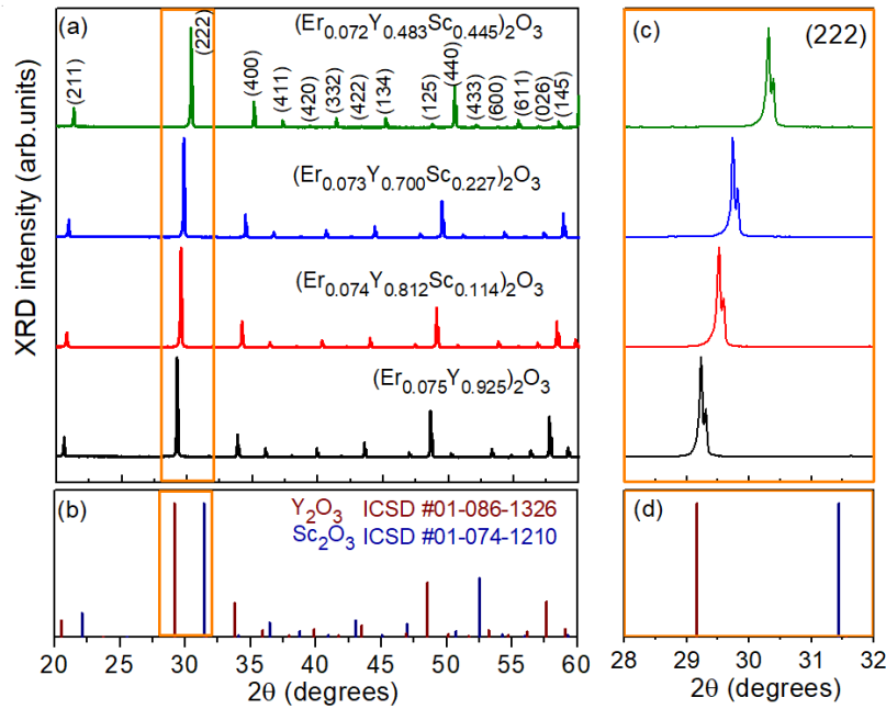
Figure V.13: (a) X-ray diffraction (XRD) patterns of the as-sintered \text{Er}:(\text{Sc}_x\text{Y}_{1-x})_2\text{O}_3 ceramics, numbers – Miller's indices ( hkl ); (b) theoretical XRD patterns of \text{Y}_2\text{O}_3 (ICSD card No. 01-086-1326) and \text{Sc}_2\text{O}_3 (ICSD card No. 01-074-1210); (c) a close look on the (222) reflection of the sesquioxide phase; (d) the corresponding theoretical reflections of \text{Y}_2\text{O}_3 and \text{Sc}_2\text{O}_3 .
