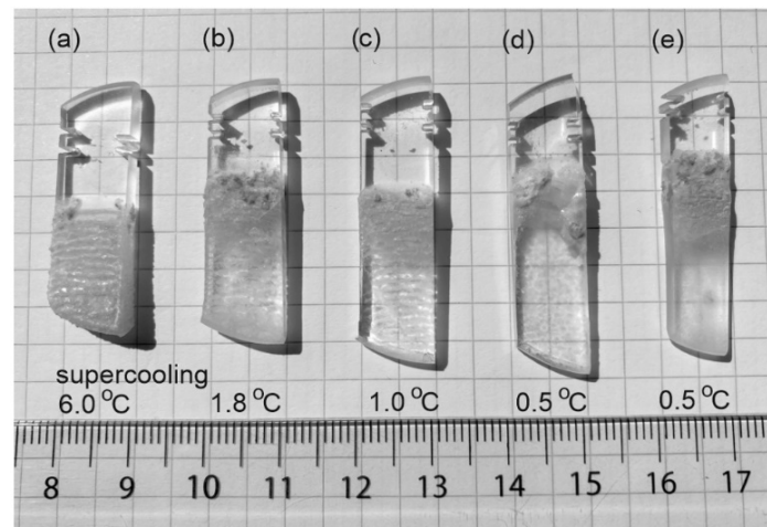
Figure III.5: Effect of the apparent supercooling on the growth behavior of Er,Gd:LiYF 4 layers on (001)-oriented LiYF 4 substrates: the supercooling is (a) 6.0 °C, (b) 1.8 °C, (c) 1.0 °C, (d) 0.5 °C (direct growth) and (e) 0.5 °C (growth after pre-dissolving the substrate at 760 °C during 5 min). The growth duration is 45 min.
