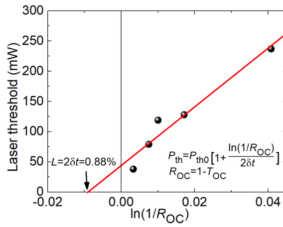
Figure V.33: Findlay-Clay analysis for the determination of the round-trip passive loss L in the \text{Er}:(\text{Y,Sc})_2\text{O}_3 ceramic laser.
