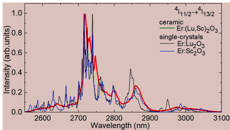
Figure V.6: A comparison of normalized mid-infrared emission spectra of \text{Er}^{3+} ions in compositionally “mixed” (\text{Lu,Sc})_2\text{O}_3 ceramic and parent single-crystalline sesquioxides, \text{Lu}_2\text{O}_3 and \text{Sc}_2\text{O}_3 at RT.
