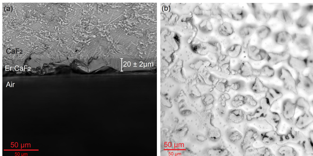
Figure III.27: Transmission mode observation of an LPE grown Er 3+ :CaF 2 layer using a confocal scanning laser microscope with \times 20 magnification: (a) polished end-facet; (b) layer top surface.
