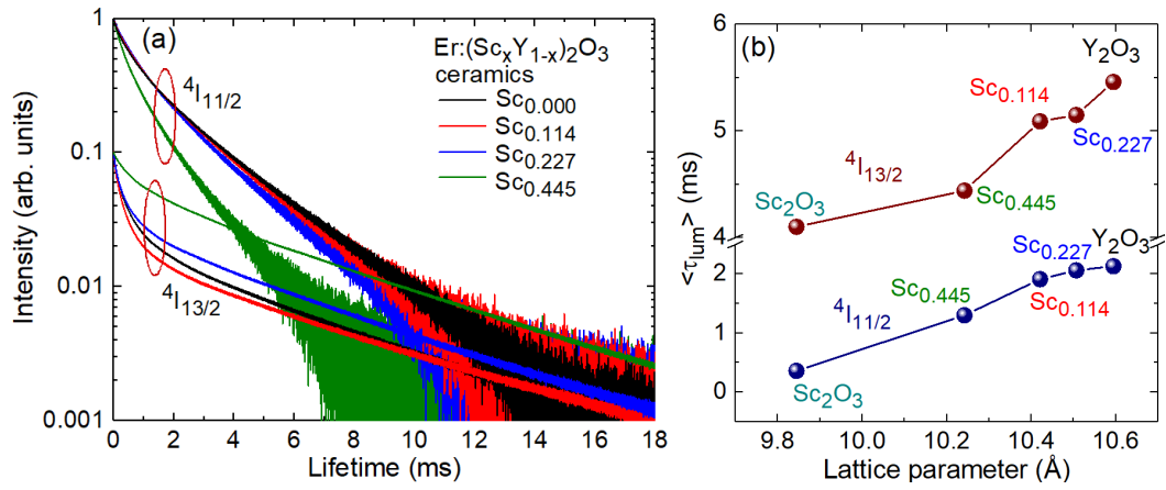
Figure V.19: (a) Luminescence decay curves for \text{Er}^{3+} ions in the (\text{Sc}_x\text{Y}_{1-x})_2\text{O}_3 ceramics for the ^4\text{I}_{11/2} state, \lambda_{\text{exc}} = 965 nm, \lambda_{\text{lum}} = 1020 nm; and ^4\text{I}_{13/2} state, \lambda_{\text{exc}} = 1460 nm, \lambda_{\text{lum}} = 1560 nm; (b) \langle\tau_{\text{lum}}\rangle plotted as a function of lattice parameter of the \text{Er}:(\text{Sc}_x\text{Y}_{1-x})_2\text{O}_3 ceramics. Solid lines are guides for the eye that have no physical meaning.
