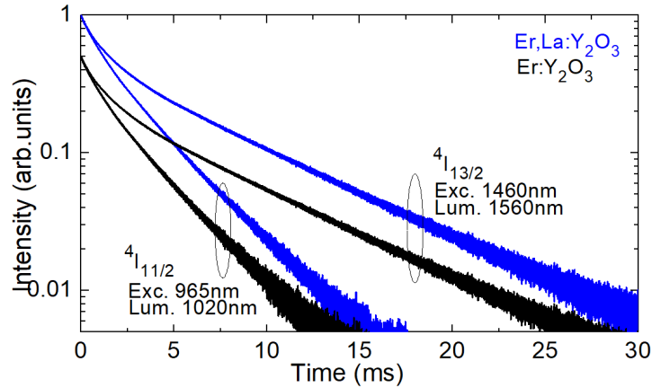
Figure V.27: Luminescence decay curves for \text{Er},\text{La}:\text{Y}_2\text{O}_3 ceramic from the {}^4\text{I}_{11/2} and {}^4\text{I}_{13/2} \text{Er}^{3+} states under resonant excitation ( {}^4\text{I}_{11/2} : \lambda_{exc} = 965 nm, \lambda_{lum} = 1020 nm; {}^4\text{I}_{13/2} : \lambda_{exc} = 1460 nm, \lambda_{lum} = 1560 nm). The decay curves for the parent ceramic, \text{Er}:\text{Y}_2\text{O}_3 , is given for comparison.
