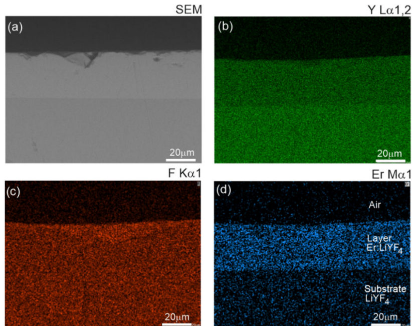
Figure III.14: Element mapping for the Er:LiYF 4 / LiYF 4 epitaxy (transversal observation): (a) SEM image, (b-d) element maps: (b) Y La 1,2 , (c) F K \alpha 1 and (d) Er M \alpha 1.
