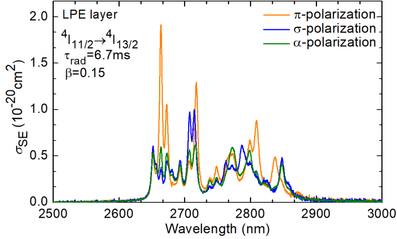
Figure III.20: Stimulated emission cross-section spectra of \text{Er}^{3+} ions from the \text{Er}:\text{LiYF}_4 epitaxial layer for the {}^4\text{I}_{11/2} \rightarrow {}^4\text{I}_{13/2} transition.
