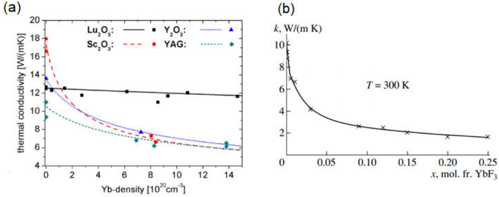
Figure I.32: Thermal conductivity versus \text{Yb}^{3+} doping concentration for some crystals of (a) sesquioxides and garnets between 0 and 15 \cdot 10^{20} \text{cm}^{-3} (corresponding to Yb:YAG (10.9 at.%), Yb:Lu 2 O 3 (5.3 at.%), Yb:Sc 2 O 3 (4.5 at.%), and Yb:Y 2 O 3 (5.6 at.%)); and (b) fluorides, namely in CaF 2 crystal. Images are taken from [Pet11, Pop08].
