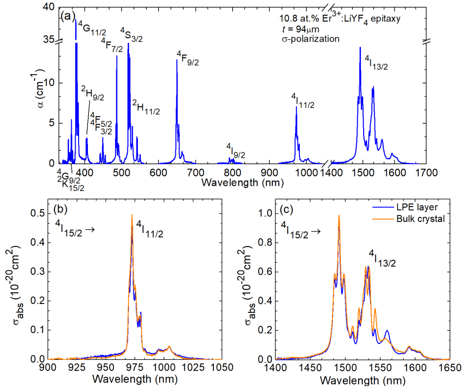
Figure III.17: Optical absorption of \text{Er}^{3+}:\text{LiYF}_4 epitaxy: (a) Overview absorption spectra in the visible and near IR spectral range; (b,c) Absorption cross-section spectra for: (b) {}^4I_{15/2} \rightarrow {}^4I_{11/2} , (c) {}^4I_{15/2} \rightarrow {}^4I_{13/2} transitions compared with the absorption cross-section, \sigma_{\text{abs}} , spectra for a 4.75 at.% \text{Er}:\text{LiYF}_4 single-crystal (in orange), both for \sigma -polarization.
