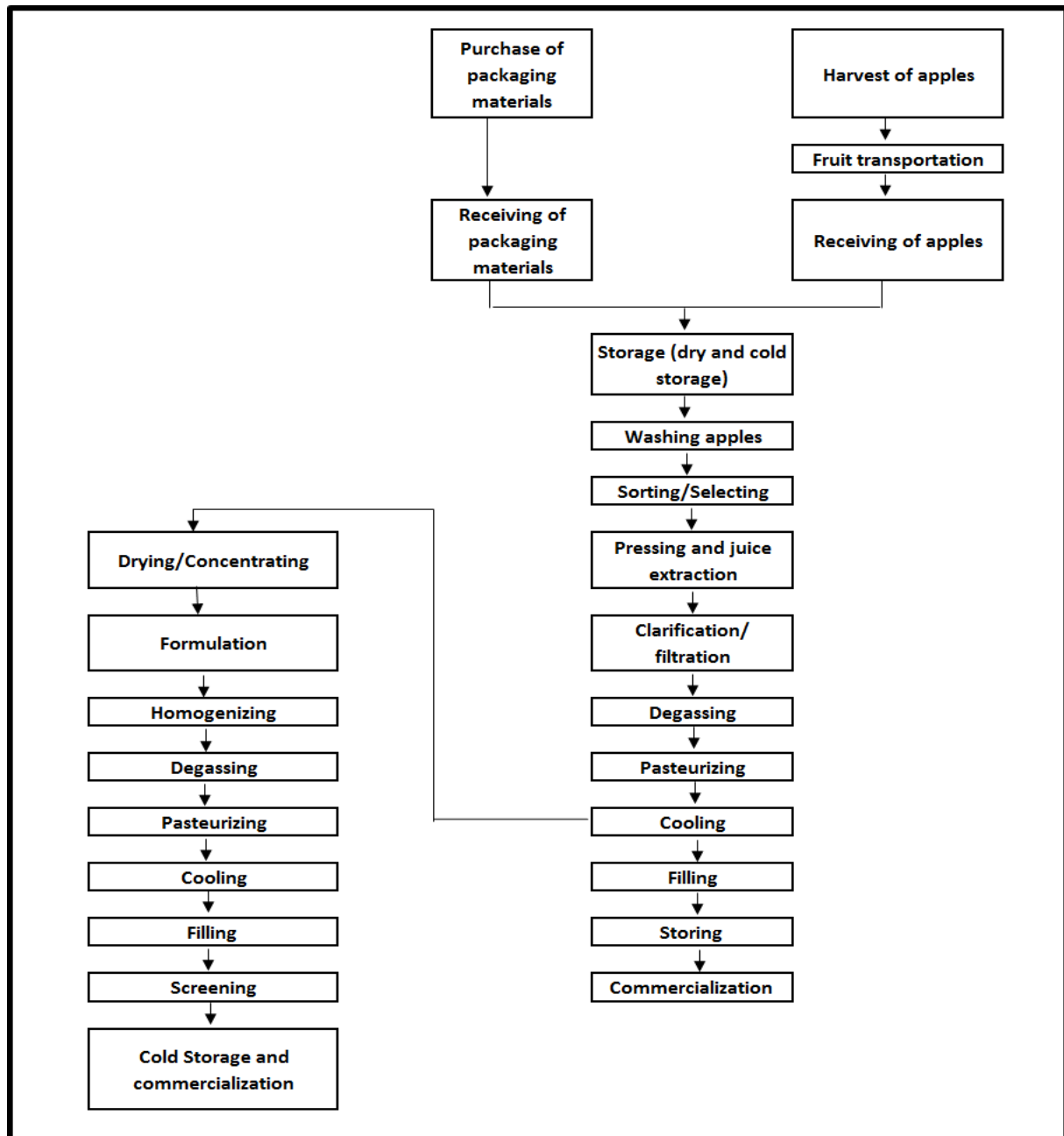
Figure 13 Apple juice processing steps adapted from Sant'Ana et al. (2008)
