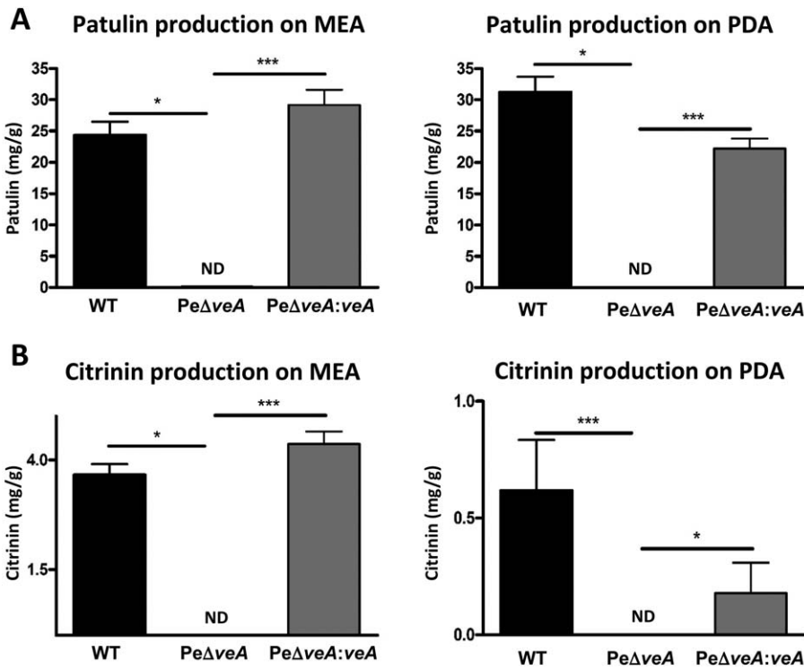
Fig. 5 Patulin and citrinin production on synthetic media by the wild-type NRRL 35695 (WT), null mutant PeΔveA and complemented PeΔveA:veA strains. (A) Production of patulin on malt extract agar (MEA) and potato dextrose agar (PDA). (B) Production of citrinin on malt extract agar (MEA) and potato dextrose agar (PDA). Patulin and citrinin production was measured by high-performance liquid chromatography by a diode array detector (HPLC-DAD) at 277 and 327 nm, respectively, at 5 days post-inoculation at 25 °C in the dark (10 4 spores). Graphs show the mean ± standard error of the mean (SEM) of eight replicates. *P < 0.05; ***P < 0.001; ND, not detectable.
