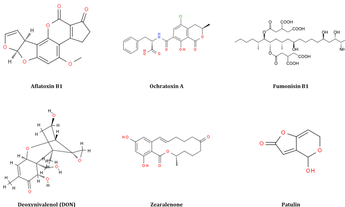
Figure 4 The chemical structures of major mycotoxins
