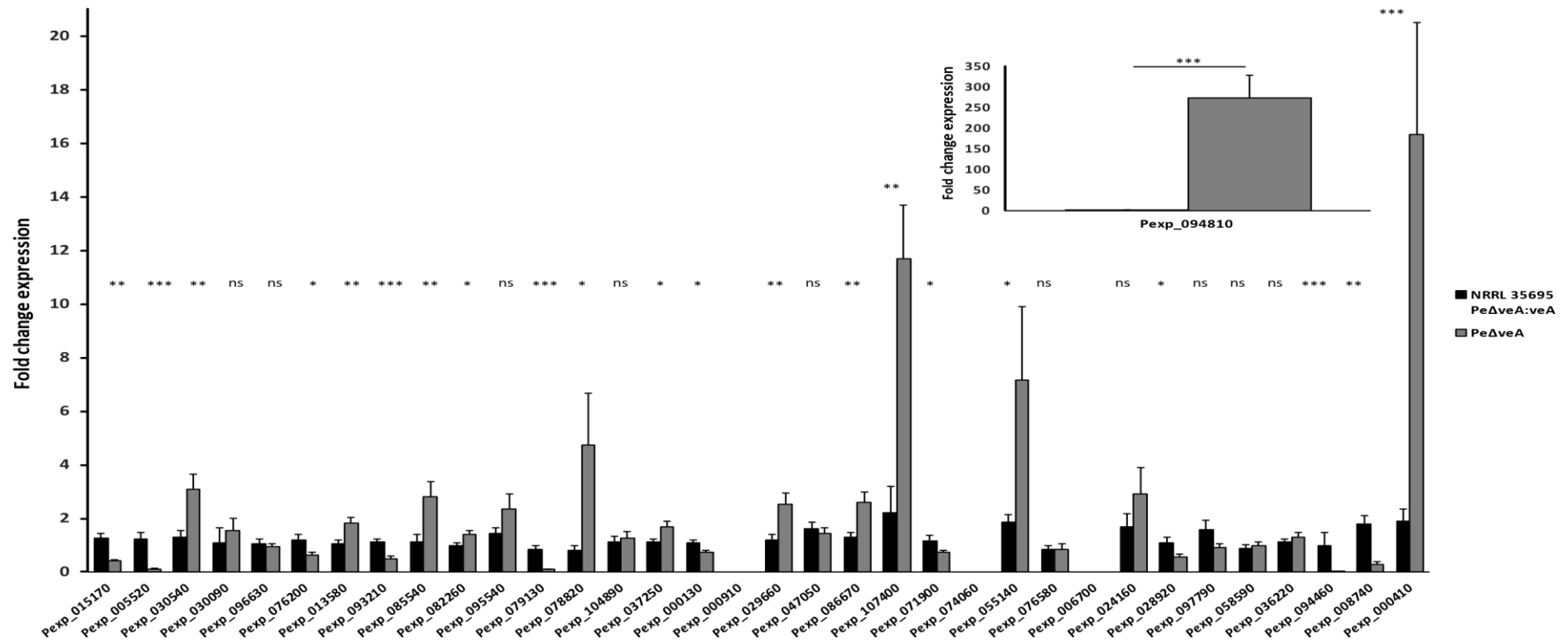
Fig. S9. Relative expression of 35 genes encoding backbone enzymes involved in secondary metabolite biosynthesis. Relative expression of polyketide synthases (PKSs), non-ribosomal peptide synthetases (NRPSs) and dimethylallyl tryptophan synthases (DMATs) identified on the sequenced genome of Penicillium expansum T01 and d1 strains grown on Potato Dextrose Agar (PDA). Gene expression was evaluated in the wildtype NRRL 35695 (WT), null mutant PeΔveA and complemented PeΔveA:veA strains. Primers were designed using PrimerExpress 2.0 software and tests were carried out using a ViiA7 Real-Time PCR System. Black bars represent combined expression level of genes in the WT and complemented strains after culture at 25°C in the dark for 5 days. Grey bars represent gene expression levels in the null mutant strain grown under the same conditions. Graphs show the mean ± standard error of the mean (SEM) of 8 replicates. Asterisks denote significant differences between the WT and the null mutant PeΔveA strains. Inset, fold change expression of Pexp_094810. nd = no difference detected, ns = no significant changes. * p -value < 0.05; ** p -value < 0.01; *** p -value < 0.001.
