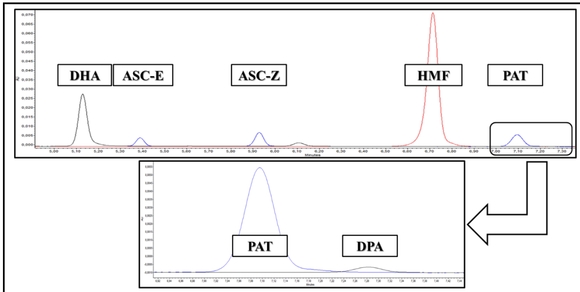
Figure 2 UHPLC chromatogram of mixture of PAT, its breakdown products (ASC-E/Z; DPA) and reaction products (DHA; HMF). PAT, patulin; DHA, dehydroascorbic acid; HMF, 5-hydroxymethylfurfural; DPA, desoxypatulinic acid; ASC-E, E-ascladiol; ASC-Z, Z-ascladiol.
