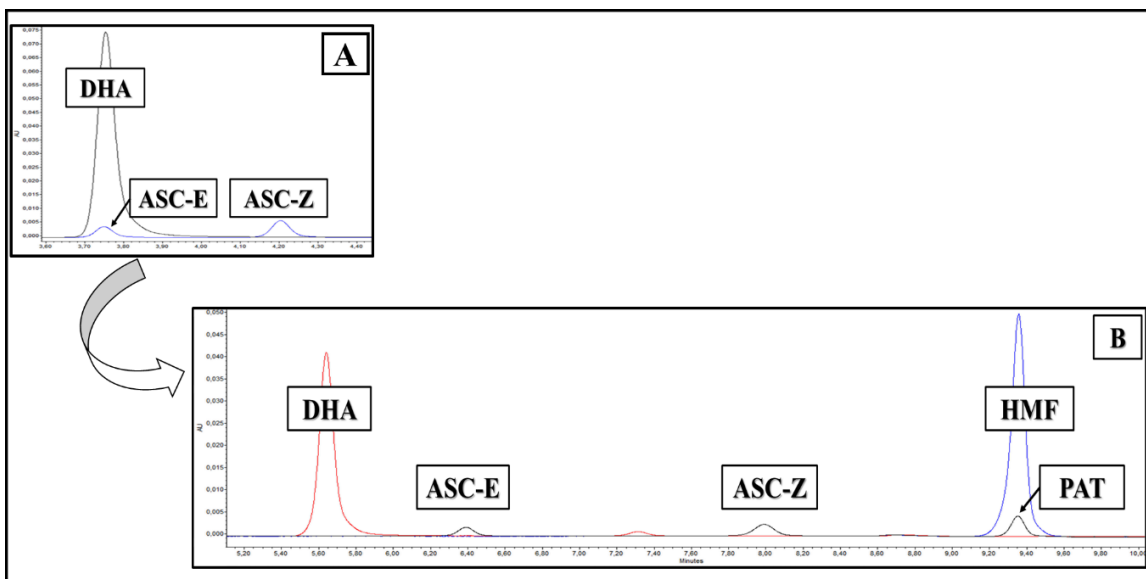
Figure 1 UHPLC chromatograms showing the interference of the UHPLC-UV signal of the secondary metabolites, degradation and reaction products following (A) a gradient method (2% B => 5% B), and (B) an isocratic method (0% B). PAT, patulin; DHA, dehydroascorbic acid; HMF, 5-hydroxymethylfurfural; ASC-E, E-ascladiol; ASC-Z, Z-ascladiol.
