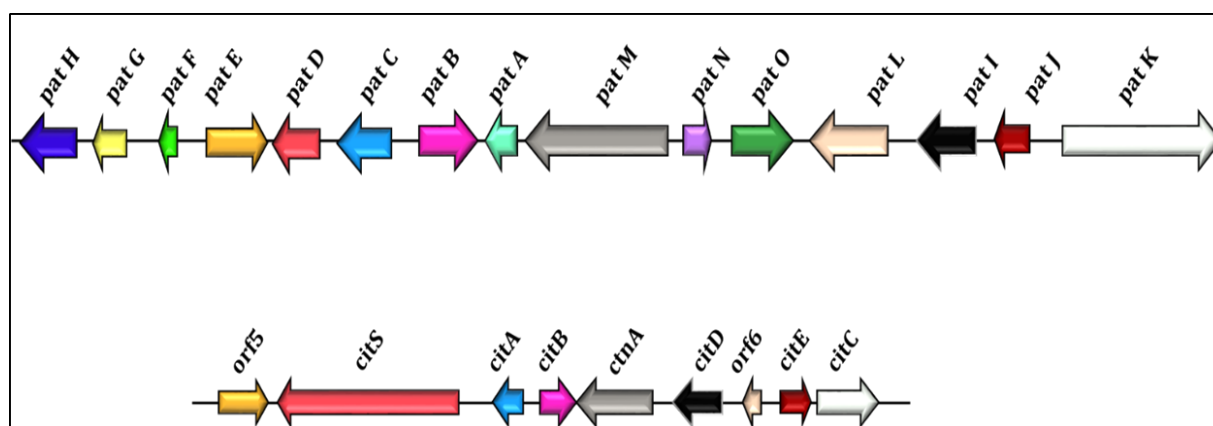
Figure 6 Gene clusters of the patulin biosynthesis pathway (the first at the top) (15 genes, 40 kb (Tannous et al. 2014)) and the citrinin biosynthesis pathway (the second at the bottom) (9 genes, 22 kb (Ballester et al. 2015; He and Cox. 2016)) in P. expansum .
