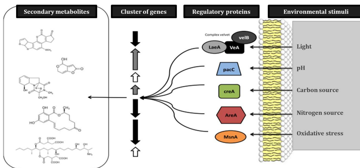
Figure 7 Global regulatory proteins involved in the regulation of gene clusters involved in the production of various fungal secondary metabolites, adapted scheme from Brakhage (2013).
