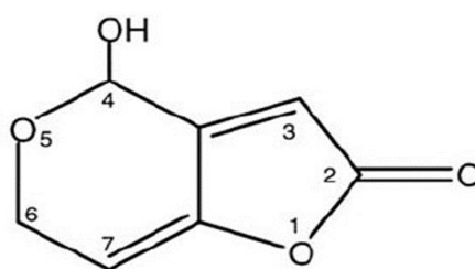
Figure 12 Chemical structure of patulin
