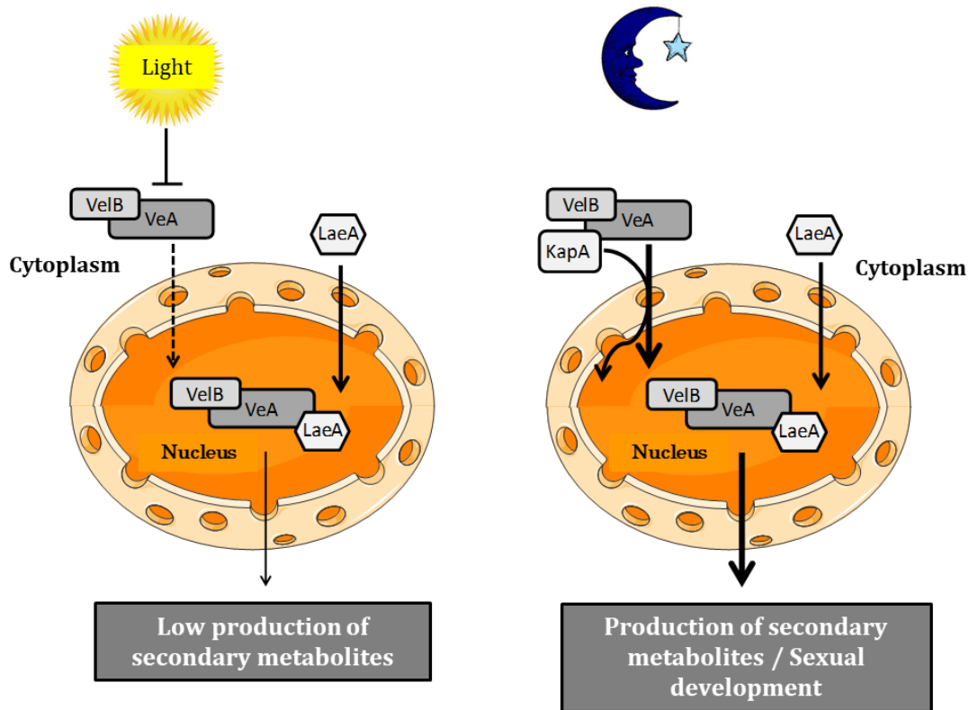
Figure 8 Operating model of the velvet complex in Aspergillus nidulans adapted from Bayram et al. (2008a). In the presence of light, VeA is retained in the cytoplasm and LaeA has low activity. In the dark, VeA coupled to VelB is transported into the nucleus by the importin \alpha KapA and the velvet complex is formed with LaeA to activate the production of secondary metabolites and sexual development
