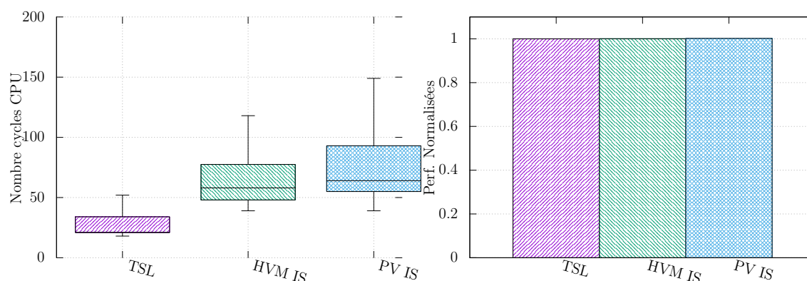
FIGURE 3.14 – Estimation de l'overhead de I-Spinlock.
