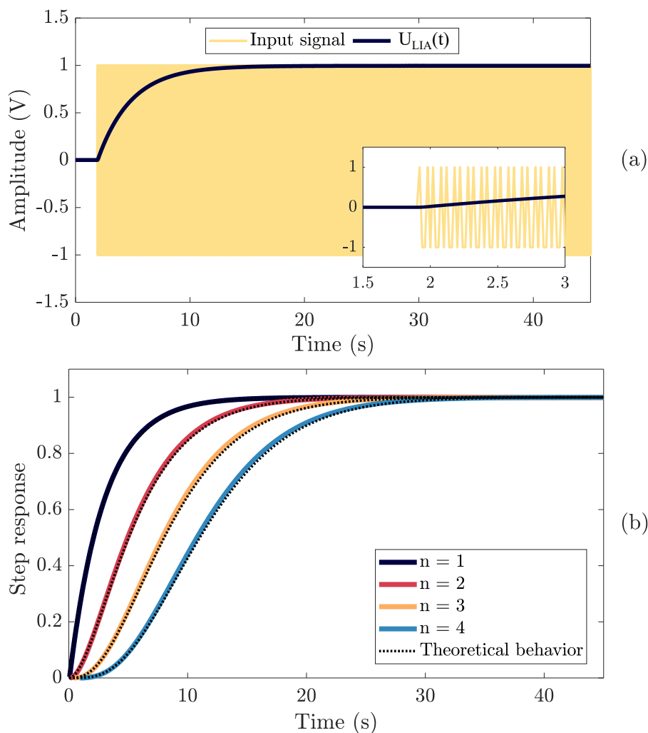
FIGURE 2.7 – (a) Step response of the LIA (black curve) for a 1-order low-pass filter with \tau_c = 3\text{s} . The frequency of the input signal (yellow) is f = 20\text{ Hz} . The insert is a zoom at the beginning of the acquisition. (b) Measured step response of the lock-in amplifier depending on the selected filter, and comparison with the theoretical behavior (dotted lines). The time constant is set at 3\text{s}
