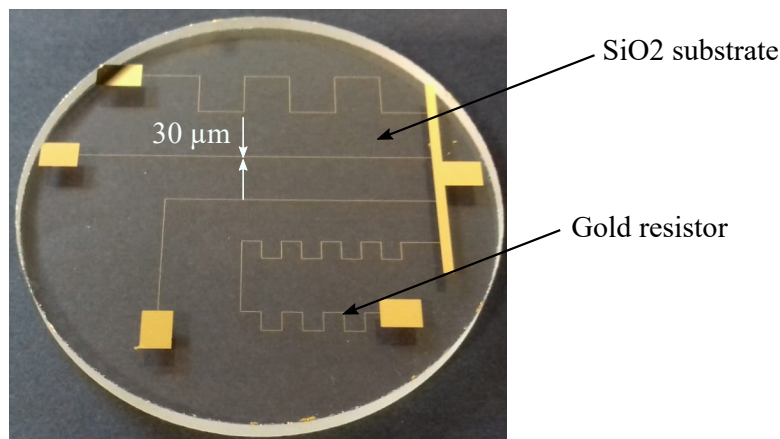
FIGURE 4.1 – Picture of a SiO 2 sample with gold resistors at its surface.
