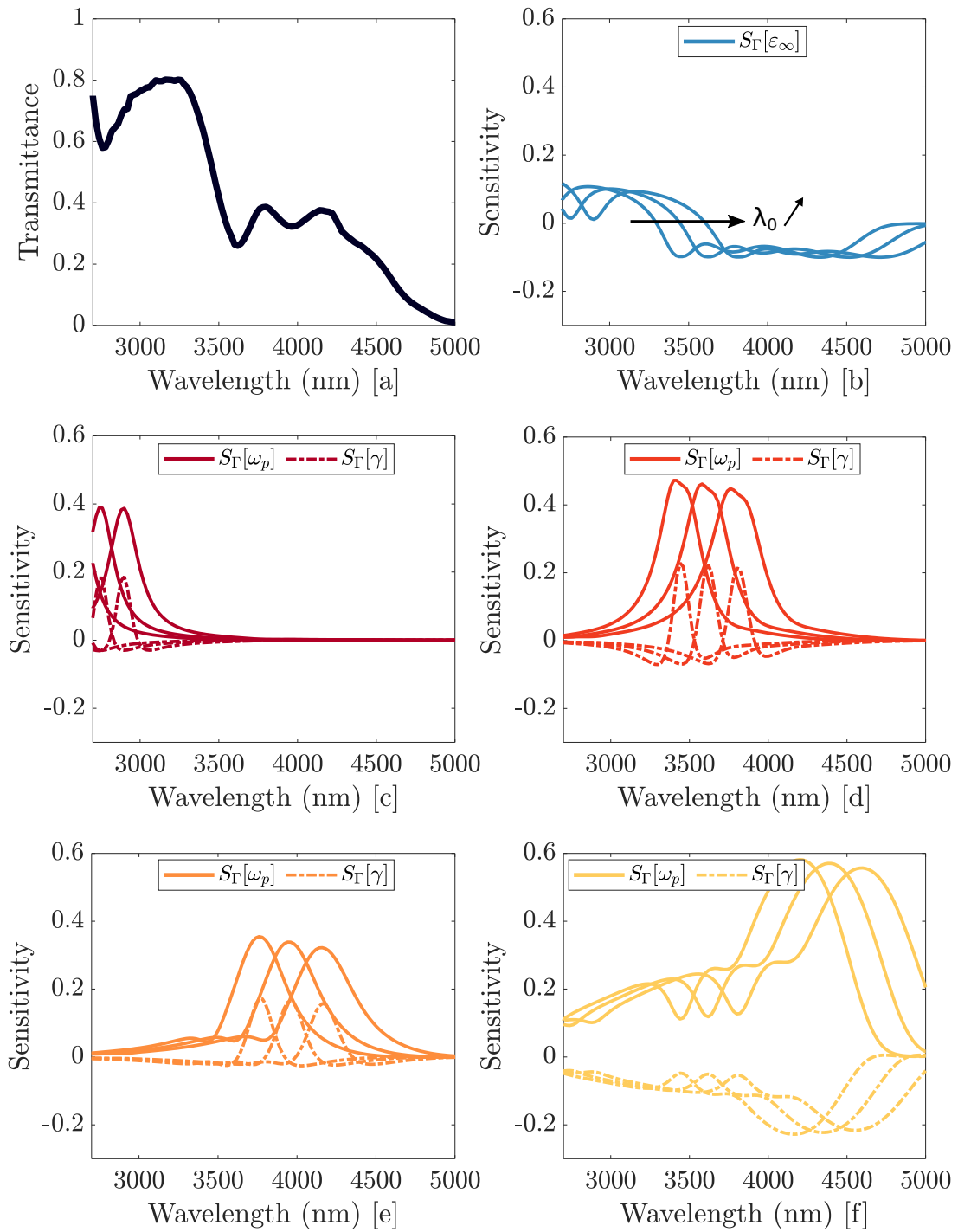
FIGURE 3.24 – [a] Reminder of the Borofloat spectral transmittance. [b] Transmittance sensitivity to \epsilon_{\infty} , for a variation of \lambda_0 of \pm 5\% . [c to f] Transmittance sensitivity to \omega_p (plain lines) and \gamma (dotted lines) with a variation of 10%, at each resonant wavelength. [c] \lambda_0 = 2750 nm \pm 5\% , [d] \lambda_0 = 3620 nm \pm 5\% , [e] \lambda_0 = 3960 nm \pm 5\% , and [f] \lambda_0 = 5500 nm \pm 5\% .
