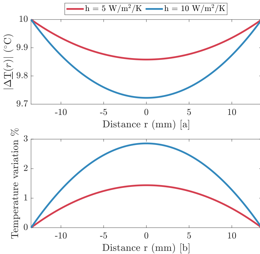
FIGURE 2.10 – (a) Amplitude |\Delta T(r, \omega_T)| depending on the distance r (mm). (b) Temperature variation in the sample compared to \Delta T(r_0) . The frequency is f_T = 10 \text{ mHz} .
