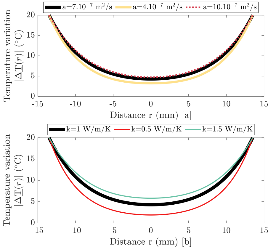
FIGURE 3.11 – Amplitude |\Delta\underline{T}(r, \omega_t)| as a function of the distance r (mm) (a) varying the thermal diffusivity with fixed thermal conductivity k = 1 \text{ W/m/K} , and (b) varying the thermal conductivity with fixed thermal diffusivity a = 7 \cdot 10^{-7} \text{ m}^2/\text{s} . The frequency is f_T = 5 \text{ mHz} and the convection coefficient is h = 10 \text{ W/m}^2/\text{K} . The black lines correspond to the set of data used in the model.
