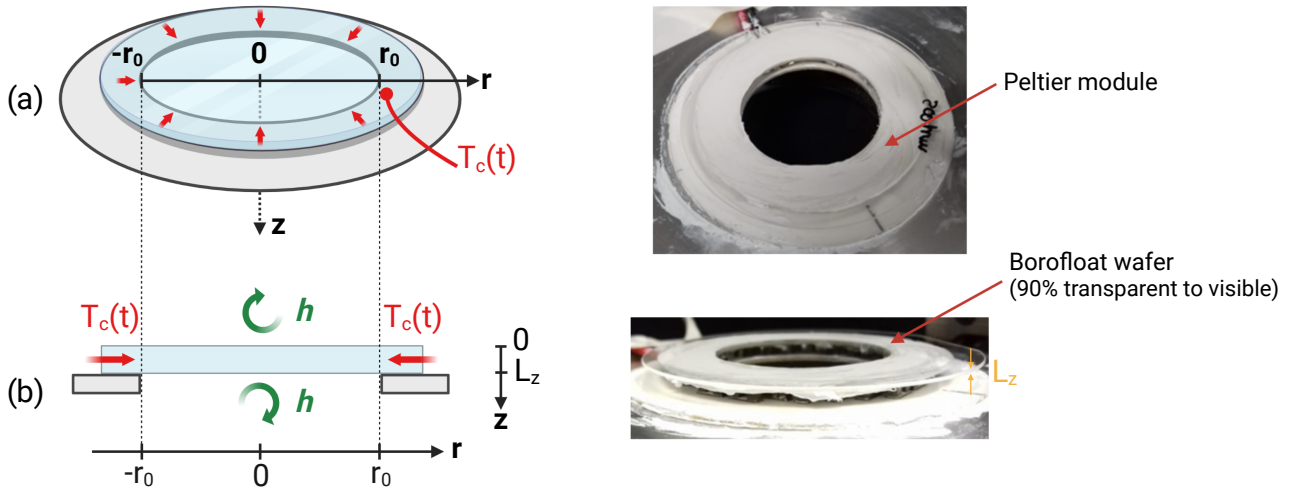
FIGURE 3.8 – Reminder of the Peltier module geometry, with heat transfer boundary conditions and corresponding images.
