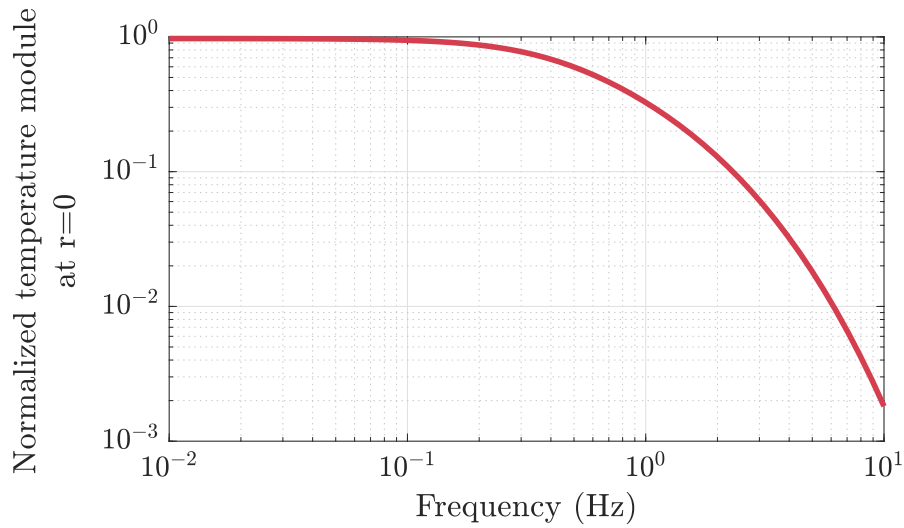
FIGURE 2.9 – Normalized temperature module |\Delta T(0)|/\Delta T(r_0) at the center depending on the frequency f_T . The convection coefficient is h = 10 \text{ W/m}^2/\text{K} .
