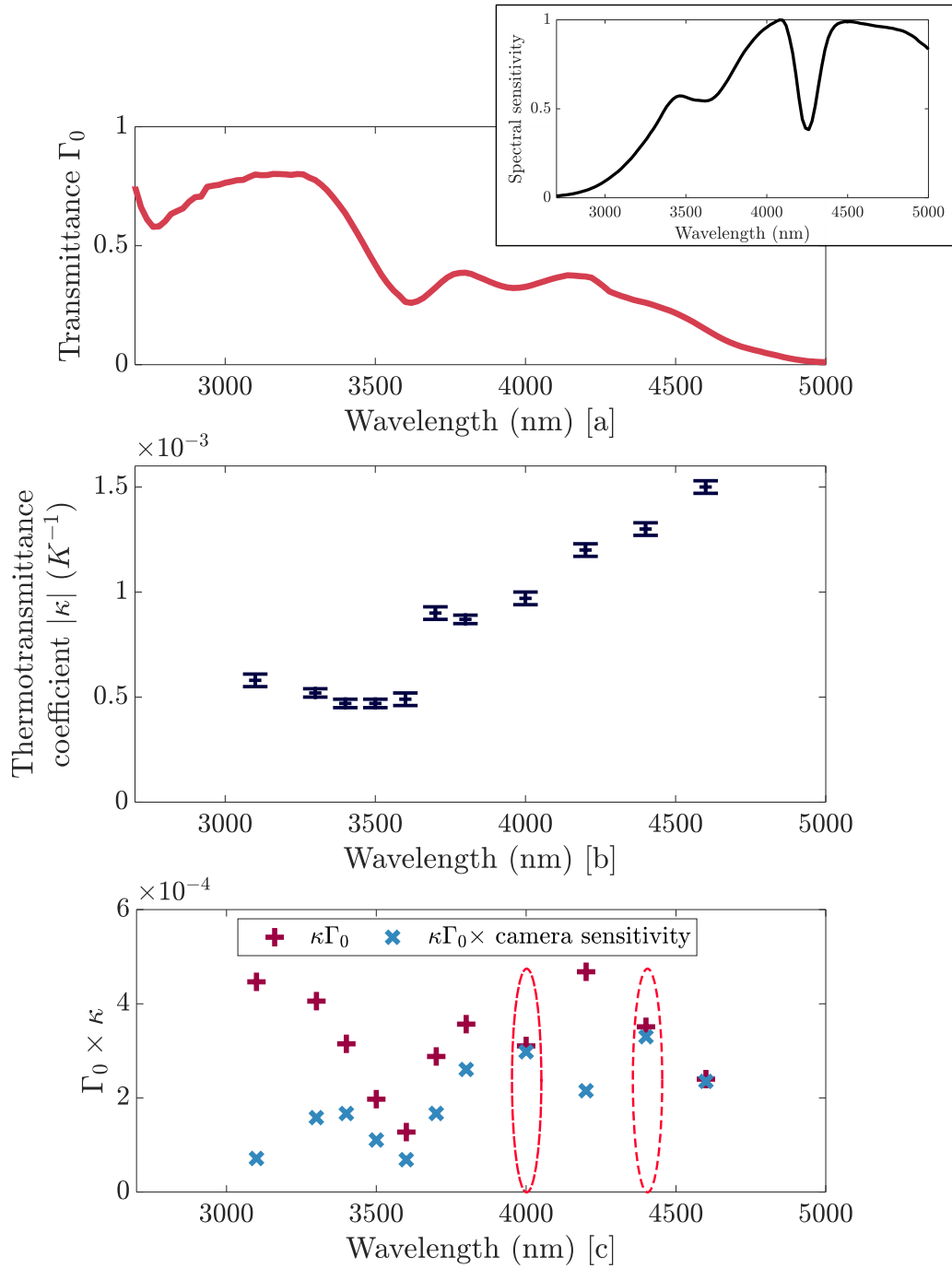
FIGURE 3.20 – [a] Reminder of transmittance spectrum \Gamma_0 , and spectral sensitivity of the acquisition chain in the insert. [b] Spectral thermotransmittance coefficient |\kappa(\lambda)| (absolute value). [c] Absolute variations \Delta\Gamma for a temperature rise of \Delta T = 1 K (red crosses). Blue crosses correspond to signal weighted by the sensitivity of the acquisition chain (see insert in (a)). The dotted red boxes show the best wavelengths to measure thermotransmittance of the Borofloat with the current setup.
