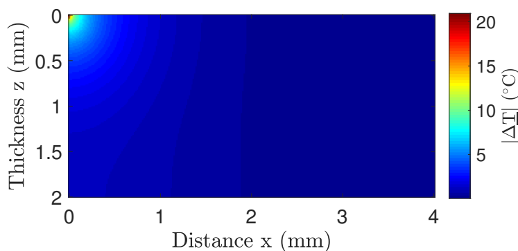
FIGURE 4.15 – Estimated temperature field |\Delta \underline{T}(x, z, \omega_T)| with the flux dissipated by Joule effect.
