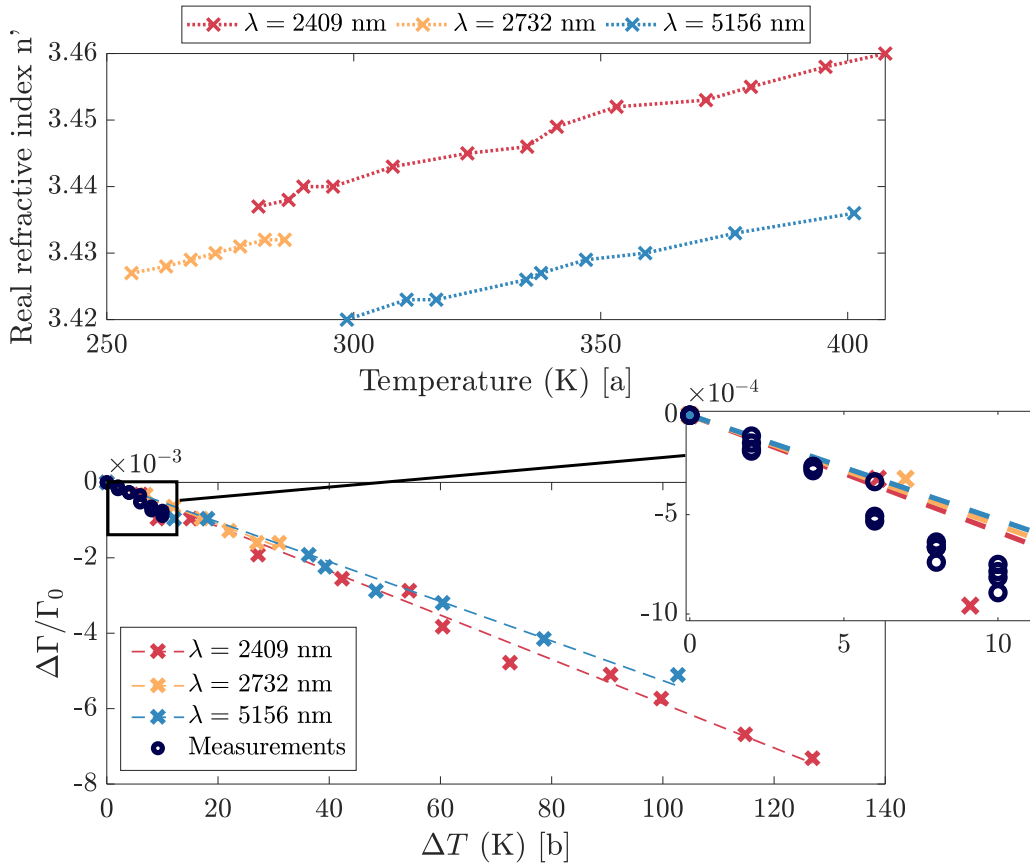
FIGURE 2.16 – [a] Real part of the Silicon refractive index depending on temperature, measured by H.H Li [85]. [b] Estimated thermotransmittance depending on temperature from the thermal dependency of the refractive index, for several wavelengths. The insert shows our measurements for \Delta T \in [0 - 10]^\circ\text{C} and \lambda = 4 \mu\text{m} .
