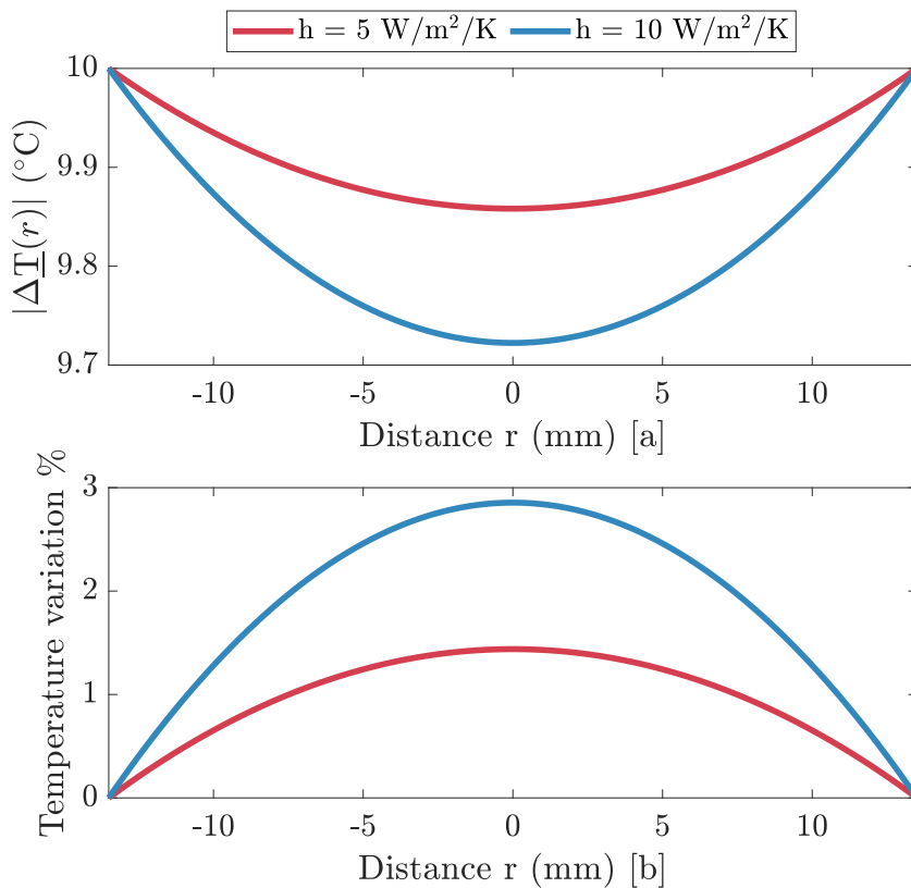
FIGURE 2.10 – (a) Amplitude |\Delta T(r, \omega_T)| depending on the distance r (mm). (b) Temperature variation in the sample compared to \Delta T(r_0) . The frequency is f_T = 10 \text{ mHz} .
