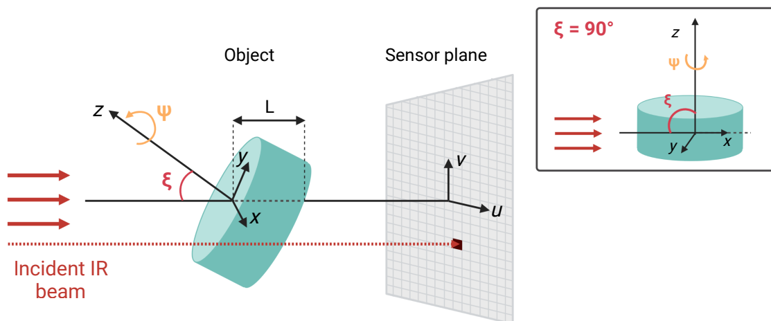
FIGURE 5.2 – Illustration of the rotary laminography and the coordinate systems used in this chapter. The insert illustrates the case \xi = 90^\circ corresponding to the CT configuration.
