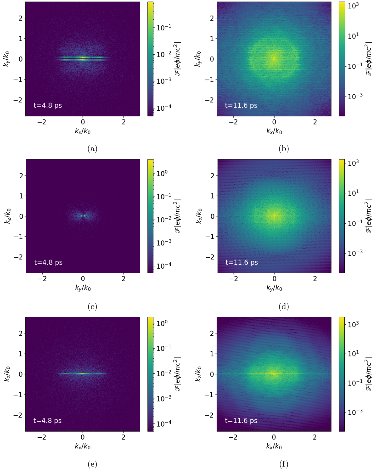
Figure 4.32: EPW potential in Fourier spectrum for the 3D TPD system, for a)-b) the x-y plane, c)-d) the y-z plane and e)-f) the x-z plane. The left and right image columns refer to the simulation time of t = 4.8 and 11.6 ps, respectively.
