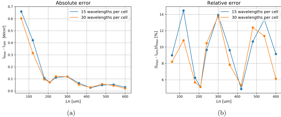
Figure 3.3: a) Absolute and b) relative error between the theoretical laser intensity threshold for SRS I_{theo} and the LPSE simulation one I_{sim} as a function of the density scale length L_n .
