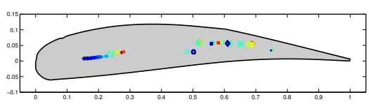
(b) Hinge locus ranked by C_{int} cost.
