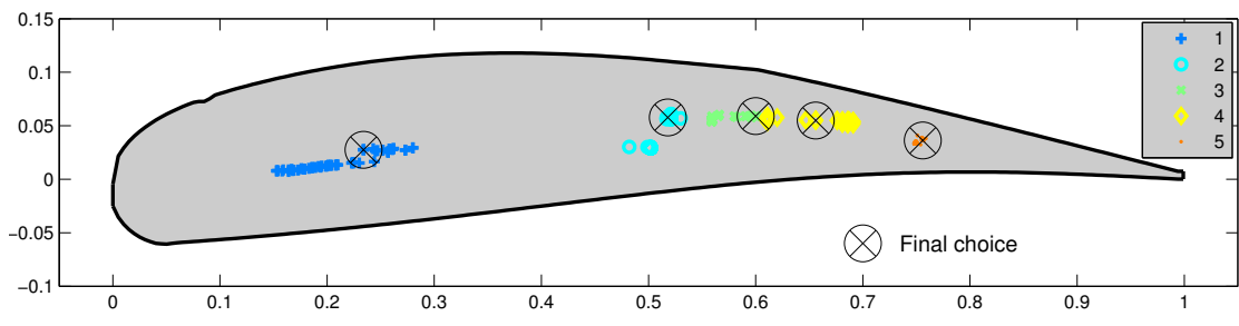
(a) Hinge locus ranked by hinge number.
