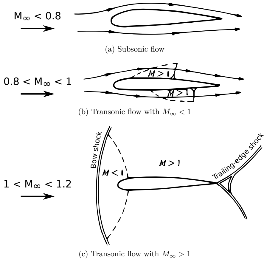
Figure 1.7: Compressibility effects on wings, from Anderson [And10].
