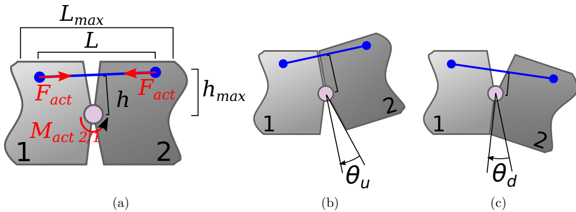
Figure 4.7: (a) Parametrized sketch of an actuated articulation. (b) Rotation when actuated, the maximum rotation angle is \theta_u . (c) Rotation when non-actuated, the mainimum rotation angle is \theta_d .
