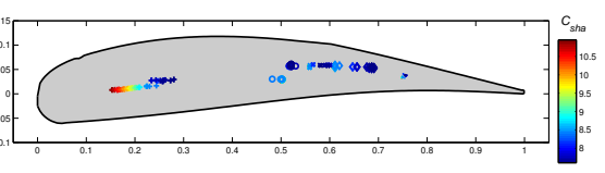
(c) Hinge locus ranked by C_{sha} cost.
