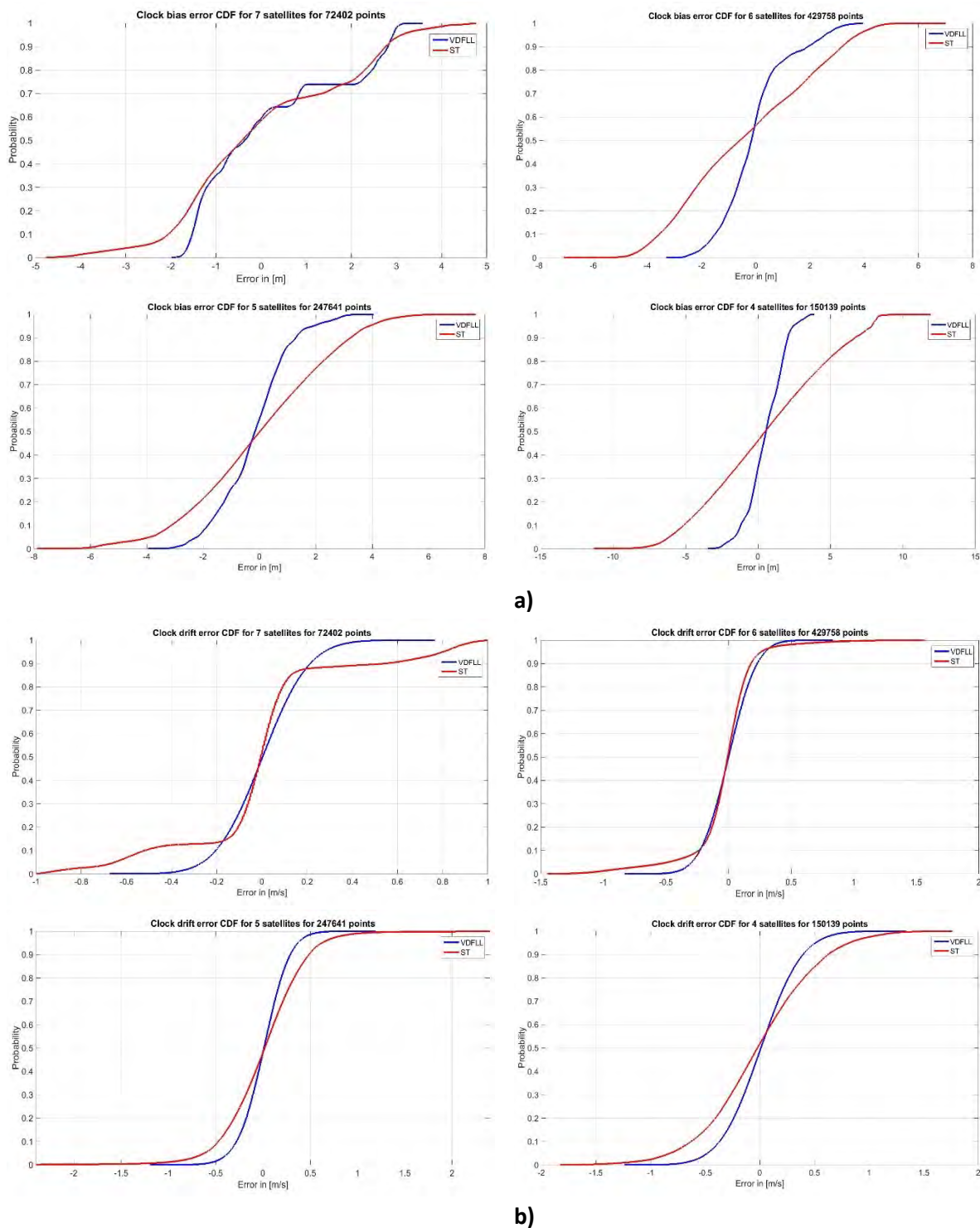
Figure D-3. a) Clock bias and b) Clock drift errors CDFs from Monte Carlo simulations.
