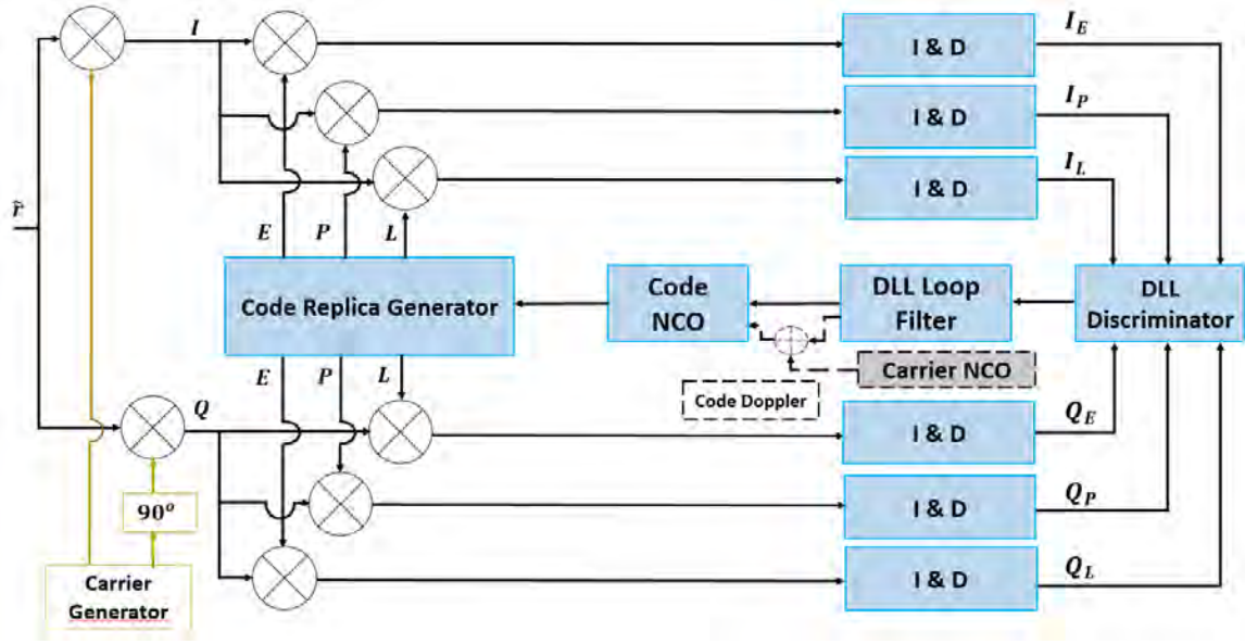
Figure 3-11. Generic code tracking (DLL) loop.
