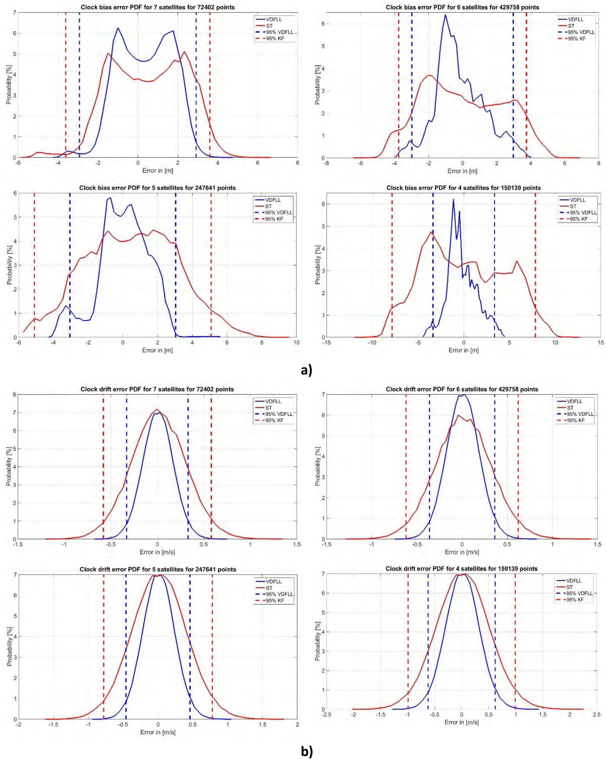
Figure 7-5. a) Clock bias and b) Clock drift errors PDFs from Monte Carlo simulations.
