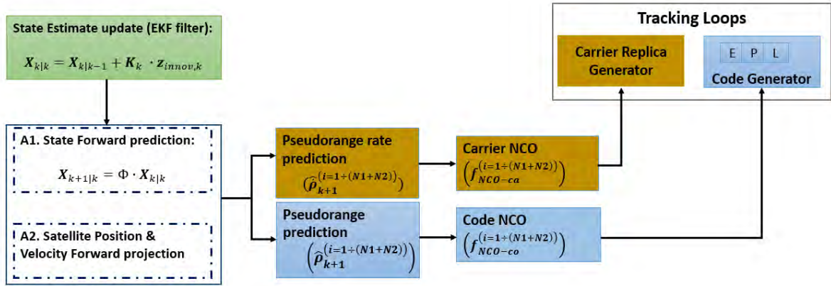
Figure 5-3. The L1/E1 VDFLL feedback loop workflow.
