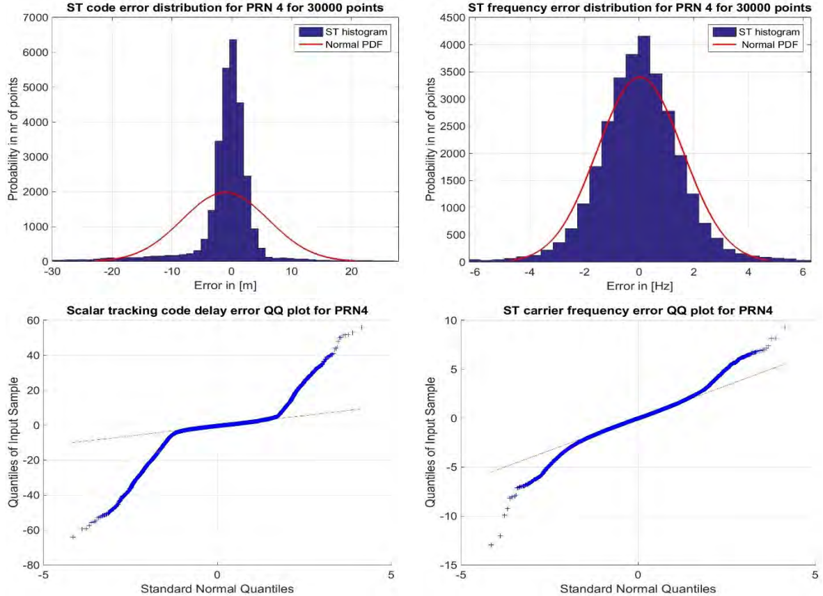
Figure 7-13. Performance comparison in the tracking channel level for one moderate LOS satellite in ionosphere and multipath reception condition.
