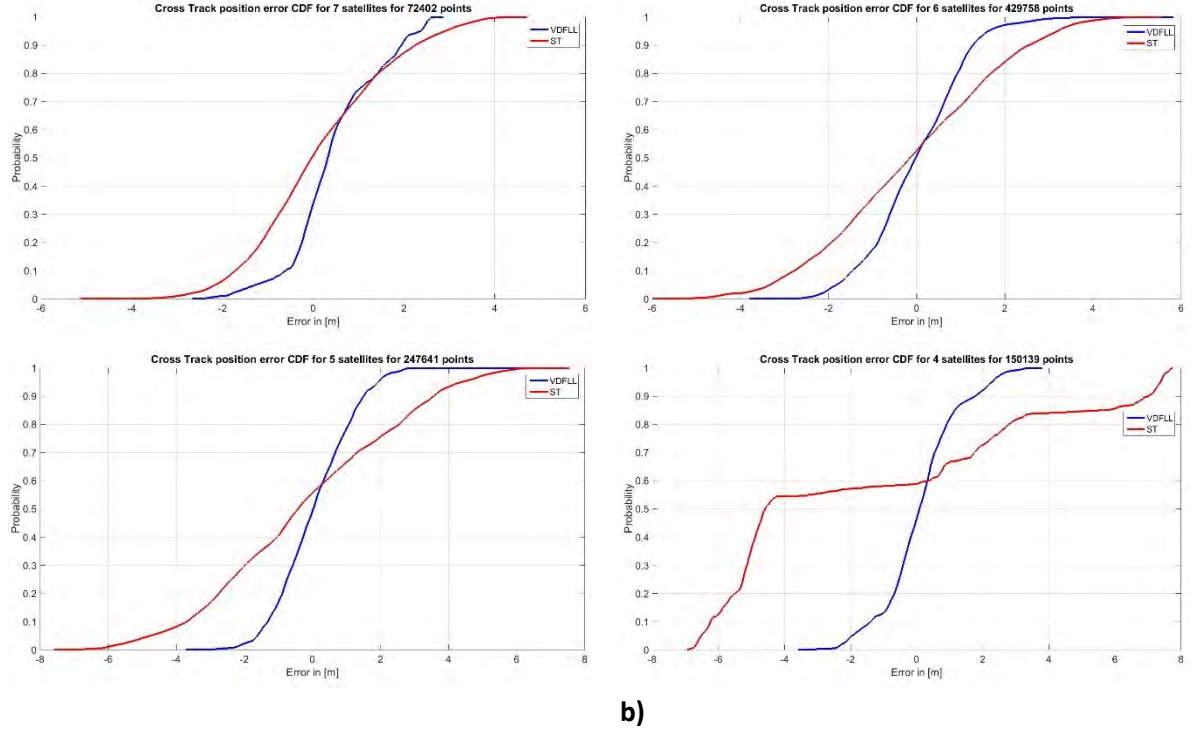
Figure D-1. a) Along- and b) Cross track position errors CDFs from Monte Carlo simulations.
