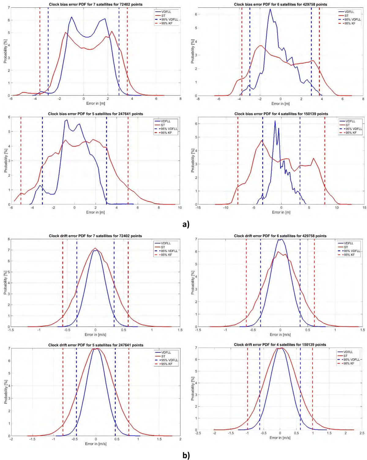
Figure 7-5. a) Clock bias and b) Clock drift errors PDFs from Monte Carlo simulations.
