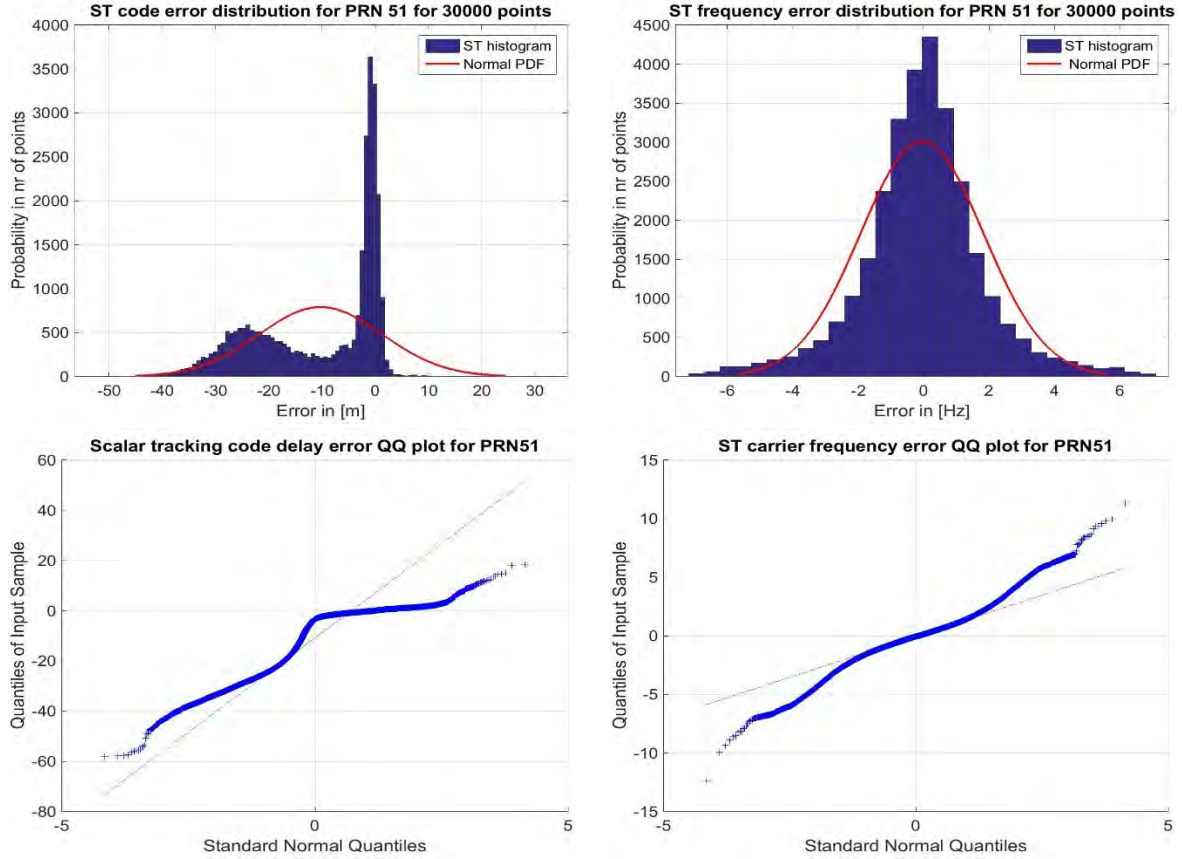
Figure 7-14. Performance comparison in the tracking channel level for a NLOS satellite in ionosphere and multipath reception condition.
