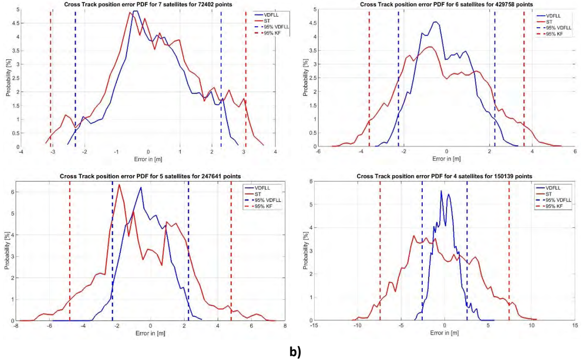
Figure 7-3. a) Along- and b) Cross track position errors PDFs from Monte Carlo simulations.
