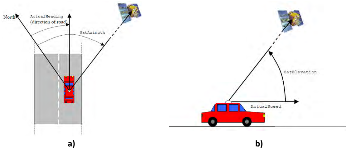
Figure 6-4. 2D-plane visualization of the: a) satellite azimuth and vehicle heading angles; b) satellite elevation angel and vehicle actual speed vector [DLR, 2007].
