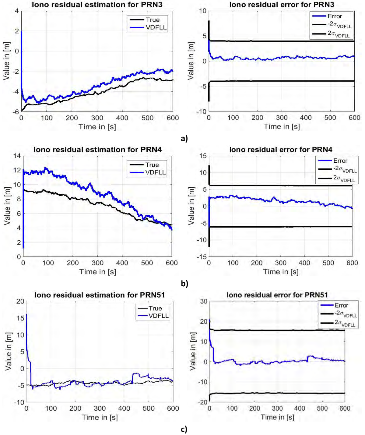
Figure 7-15. VDFLL ionosphere residual error estimation for a) a) LOS, b) Moderate LOS and c) NLOS satellite.
