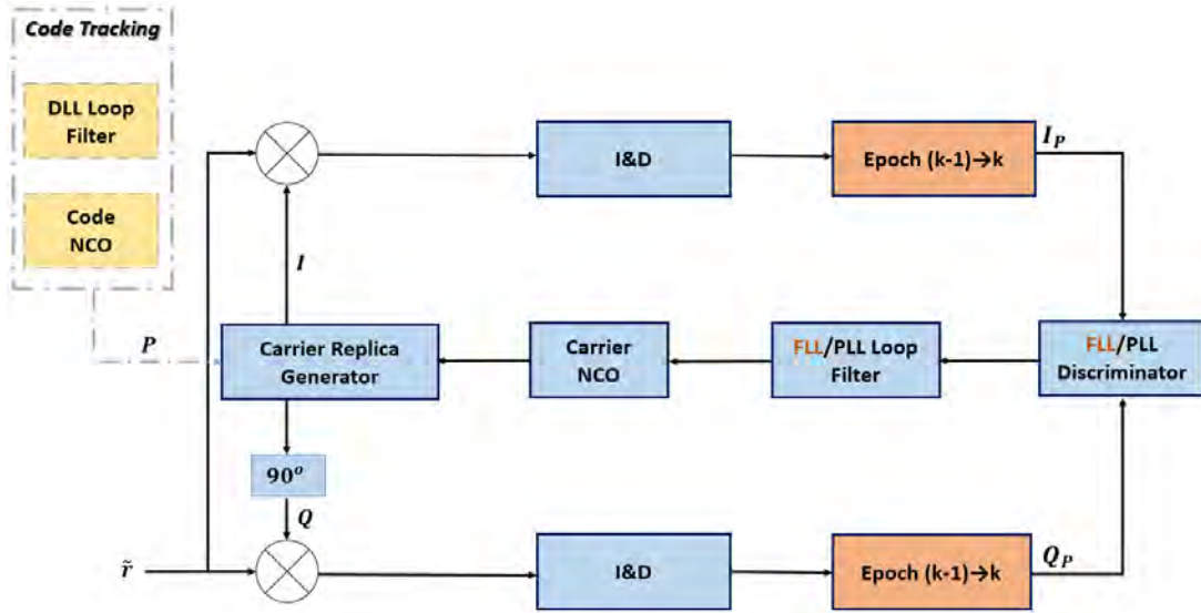
Figure 3-9. The generic tracking loop representation including both the FLL and PLL loops.
