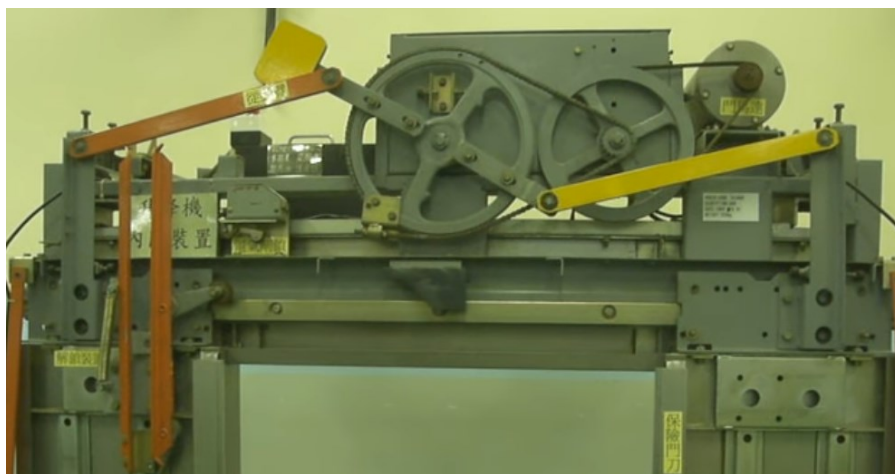
Figure 1.7 Typical driving mechanism of an elevator door opening on both sides
