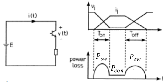
Figure 2.35 Transistor switching action waveform in one switching cycle
