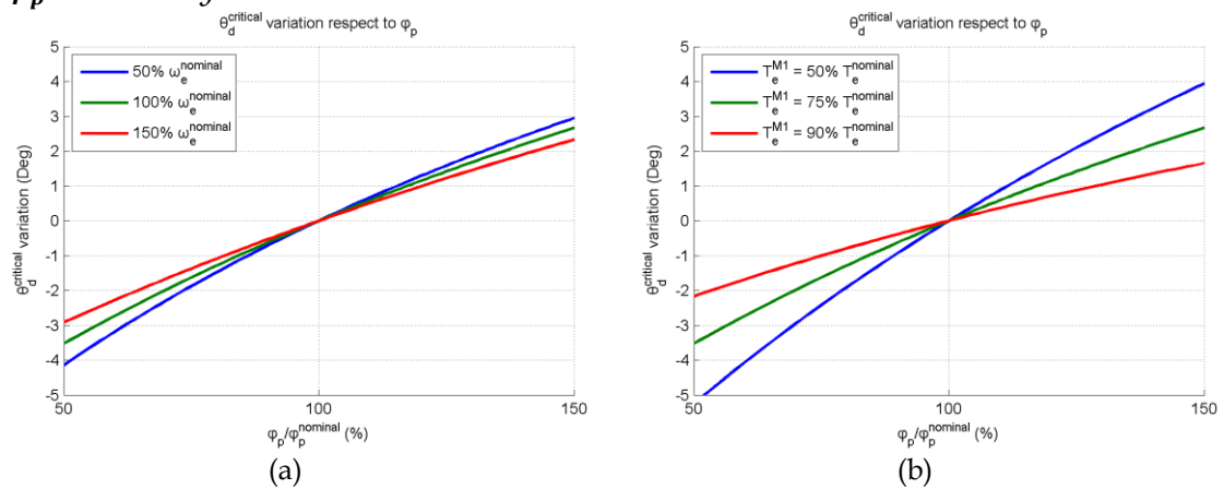
Figure 3.13 \theta_d^{critical} variation respect to \varphi_p under (a) different speed and (b) different torque load
