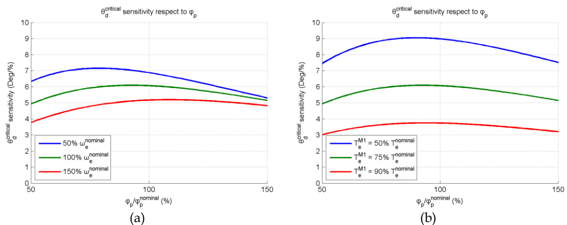
Figure 3.14 \theta_d^{critical} sensitivity respect to \varphi_p under (a) different speed and (b) different torque load
