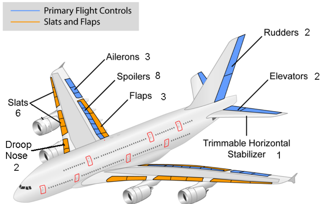
Figure 1.9 Control surface of A380.
