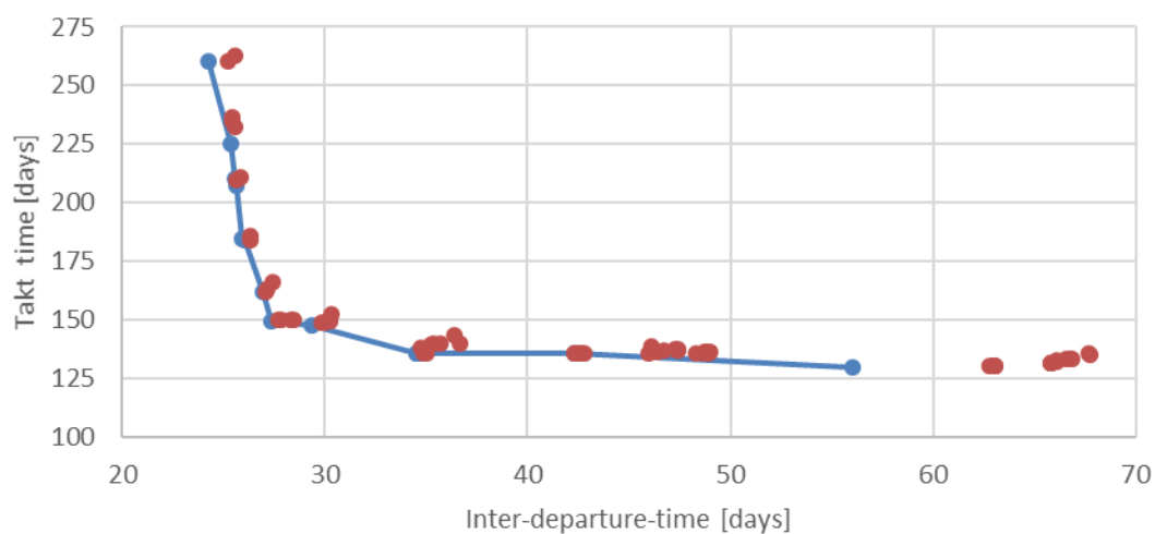
Figure 45: Optimization results for scheduling problem
