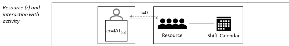
Figure 32: Resource class
