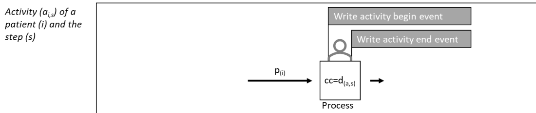
Figure 31: Process class
