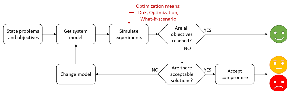
Figure 1: Problem-solving loop
