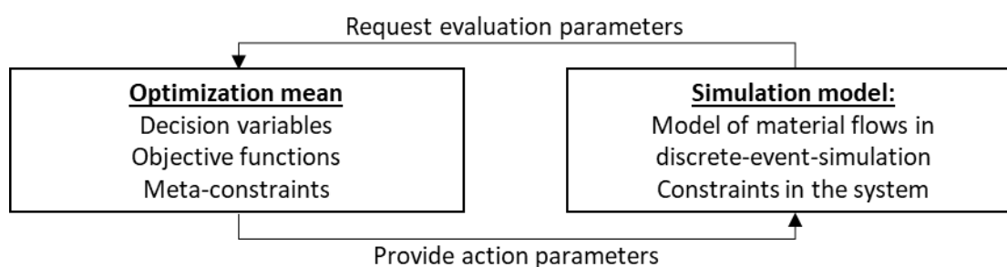
Illustration 4: Couplage simulation-optimisation
