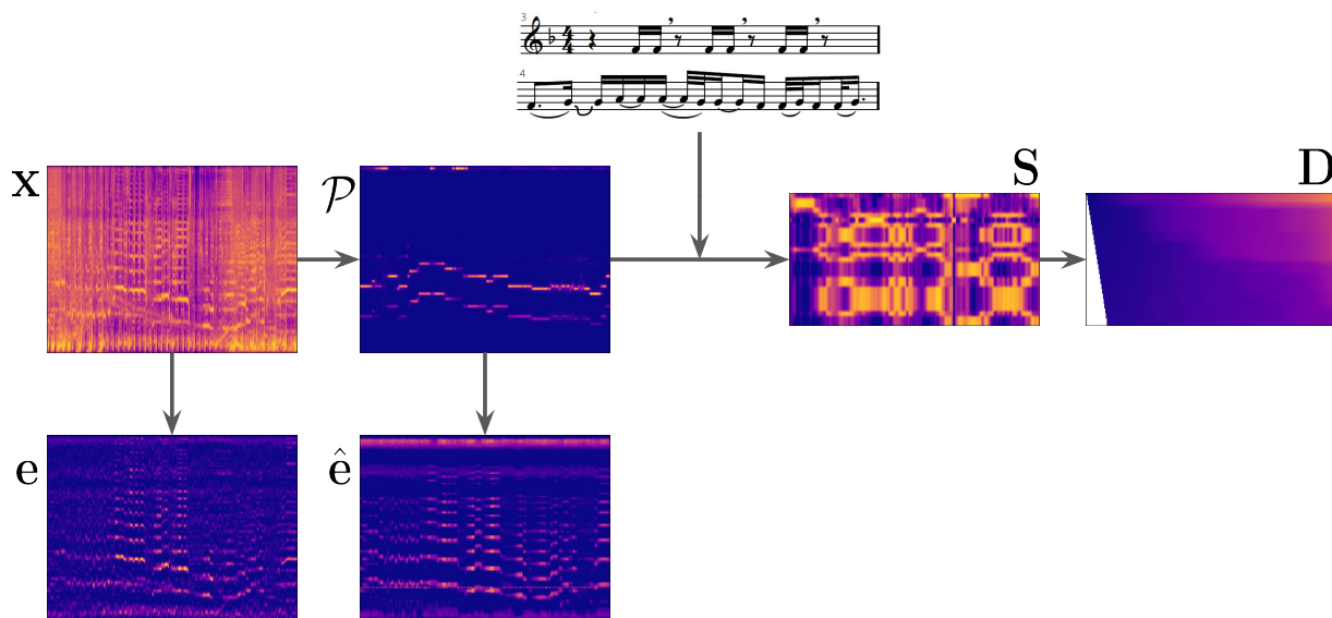
Figure 6.4: An example of inference for voice-to-note alignment with ADAGIO. Note that in this context e represents an excitation signal (all but spectral envelope). The posteriorgram, temporally constrained during training, predicts per-frame probability of note occurrences.
