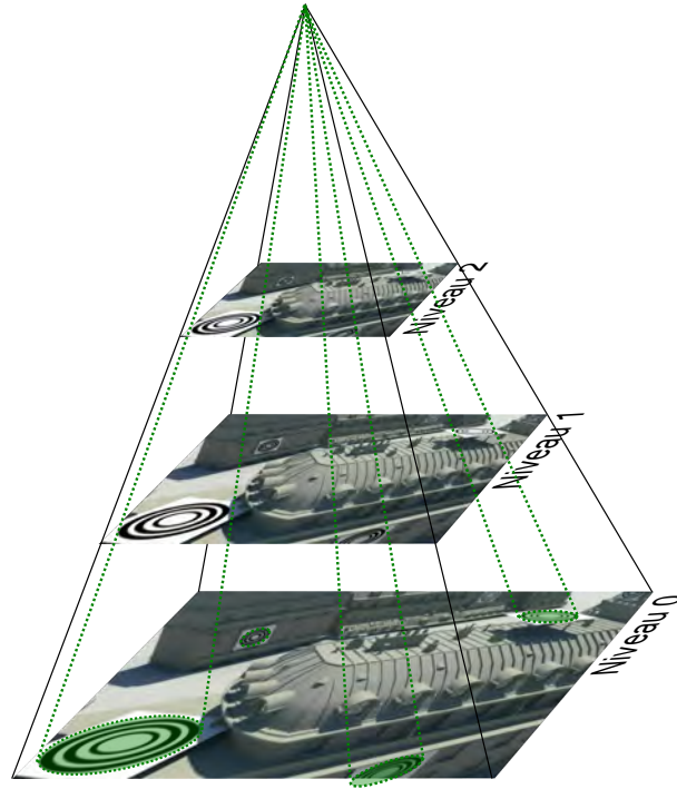
FIGURE 5.11: Pyramide d'images.
