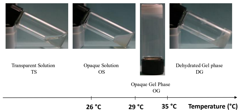
Figure III.17 Photographs of the observed phase transition for PNIPAM 4k - b -PBA 2k - b -PNIPAM 4k triblock structure at a concentration of 20 wt.% as a function of temperature: transparent solution (TS) → opaque solution (OS) → opaque gel phase (OG) → dehydrated gel phase (DG).
