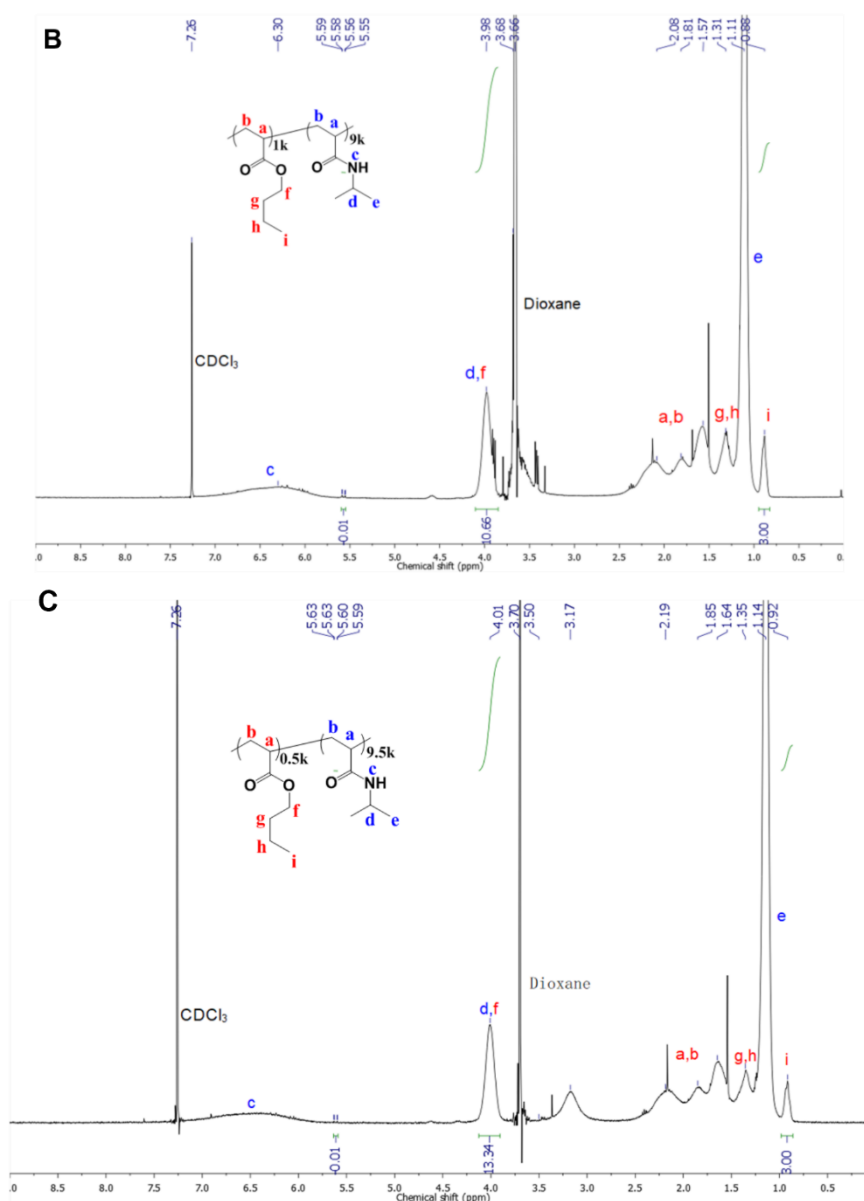
Figure III.3 ^1\text{H} NMR spectra of (A) \text{P}(\text{BA}_{2\text{k}}\text{-stat-NIPAM}_{8\text{k}}) , (B) \text{P}(\text{BA}_{1\text{k}}\text{-stat-NIPAM}_{9\text{k}}) and (C) \text{P}(\text{BA}_{0.5\text{k}}\text{-stat-NIPAM}_{9.5\text{k}}) in \text{CDCl}_3 .
