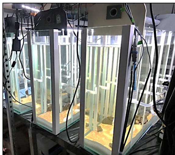
Figure 1: Aquatic mesocosms before NP contamination (T0).
