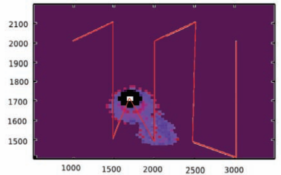
Figure 4.2 – (a) Illustration (on the environment with one target shown in figure 4.1) of the obtained map using G.I.D strategy for one underwater vehicle. (b) Illustrates the obtained map at the end of the mission execution.
