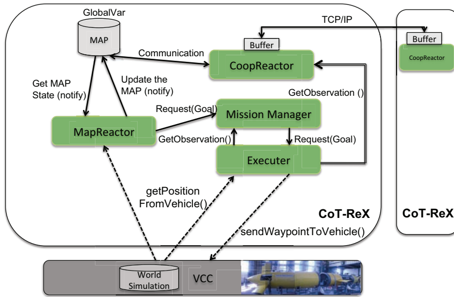
Figure 5.15 – Illustration of the proposed architecture on the real platform
