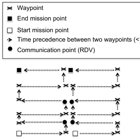
Figure 6.3 – All predefined waypoints and communication points for each underwater vehicle. Arrows represent the temporal execution precedence between two waypoints. This precedence determines the transects of each underwater vehicle.
