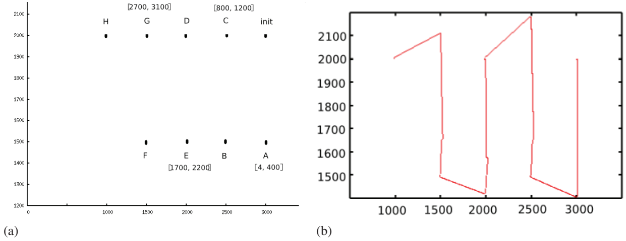
Figure 3.11 – (a). Illustration of predefined waypoints for one underwater vehicle. (b). Illustration of the obtained path. The time intervals to reach the waypoints (e.g. The vehicle can reach the point A between 4 until 400 ut) are large enough to allow the AUV explores a bit further, hence the resulting saw path.
