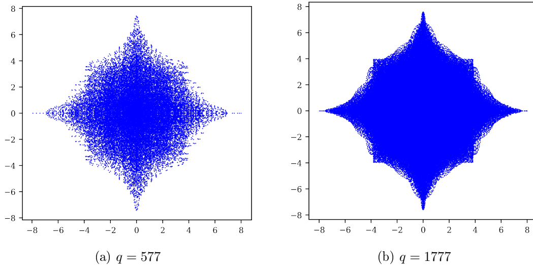
Figure 2.16: The sets \mathcal{G}_q(-, -, 8) for two 8-admissible values of q .
