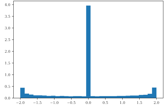
(b) Distribution of the values \frac{1}{31}K_{31^2}(a, 1) in [-2, 2] as a ranges in (\mathbf{Z}/31^2\mathbf{Z})^\times .
