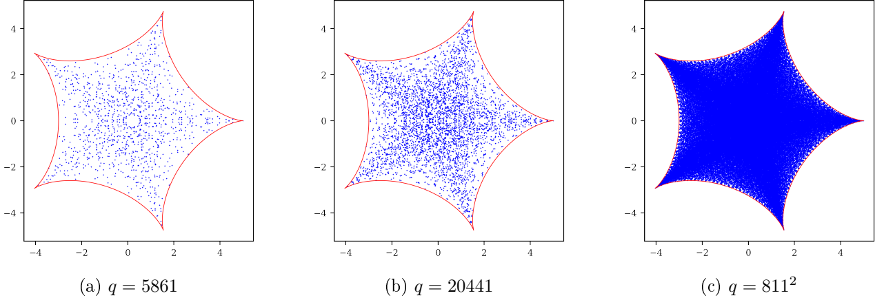
Figure 2.9: The sets \mathcal{G}_q(-, 5) and three 5-admissible values of q .
