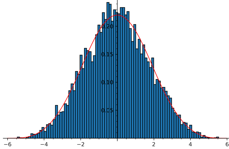
Figure 6.1: Distribution of the values of the sums \sum_{x \in \mathbb{Z}_g(\mathbb{F}_q)} \text{Kl}_2(ax, q) as a varies in \mathbb{F}_q , for g = X^3 - 9X - 1 and q = 8089 . The red curve is the probability density function of the random variable X_1 + X_2 + X_3 defined as the sum of three independent and identically distributed Sato–Tate random variables.
