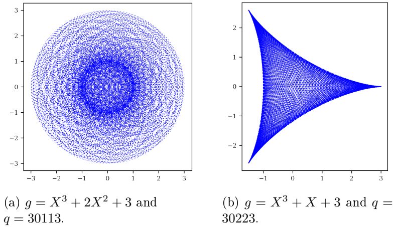
Figure 4.2: The sums \sum_{x \in \mathbf{Z}_g(\mathbf{F}_q)} e\left(\frac{ax}{q}\right) as a varies in \mathbf{F}_q , for two two different polynomials g of degree 3.
