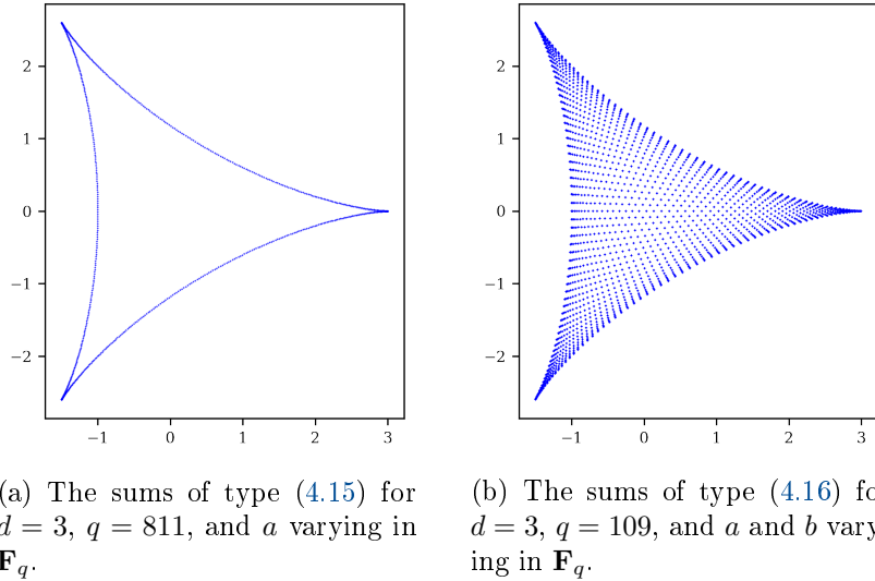
Figure 4.3: Comparison between the regions of equidistribution for sums of type (4.15) and sums of type (4.16).
