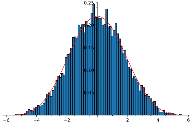
Figure 6.2: Distribution of the values of the sums \sum_{x \in \mathbb{Z}_g(\mathbb{F}_q)} \text{Kl}_2(a + x, q) as a varies in \mathbb{F}_q , for g = X^3 - 9X - 1 and q = 8089 . The red curve is the probability density function of the random variable X_1 + X_2 + X_3 defined as the sum of three independent and identically distributed Sato–Tate random variables.
