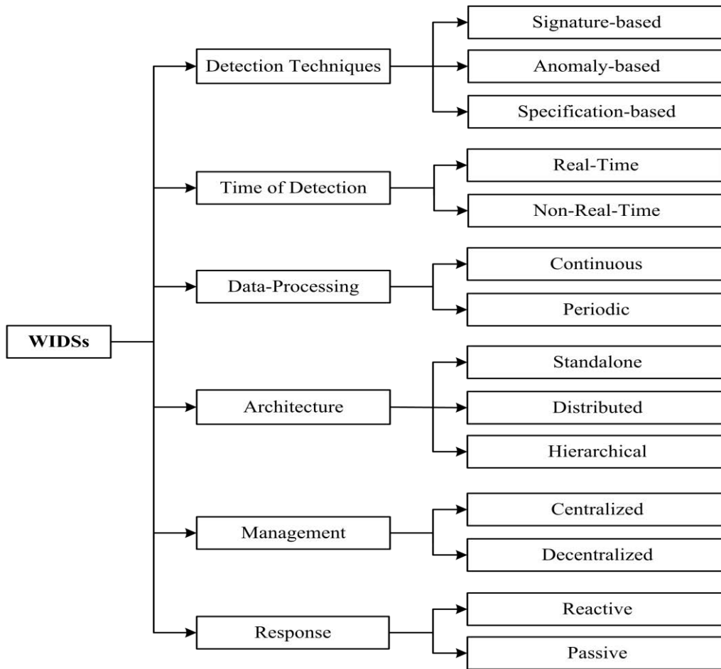
Figure III-2: WIDSs Classification.
