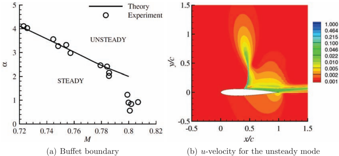
Figure 2.21: Global-stability theory results for the NACA 0012 airfoil (from Ref. [40]).
