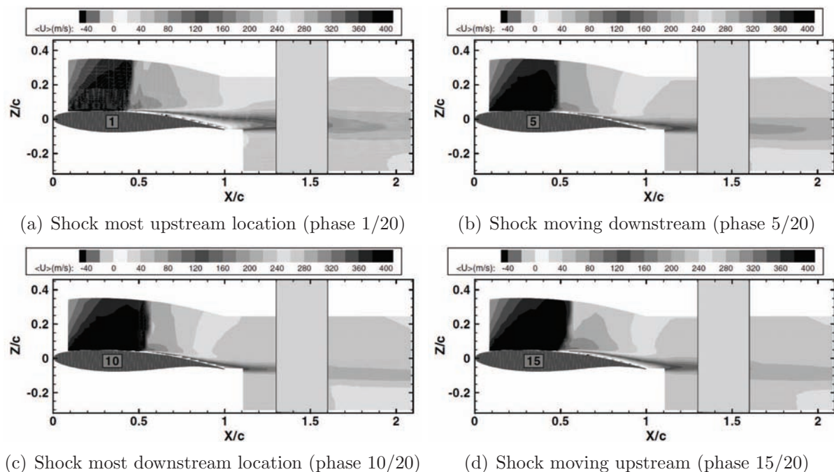
Figure 2.20: Phase-averaged velocity fields around the OAT15A (from Ref. [39]).
