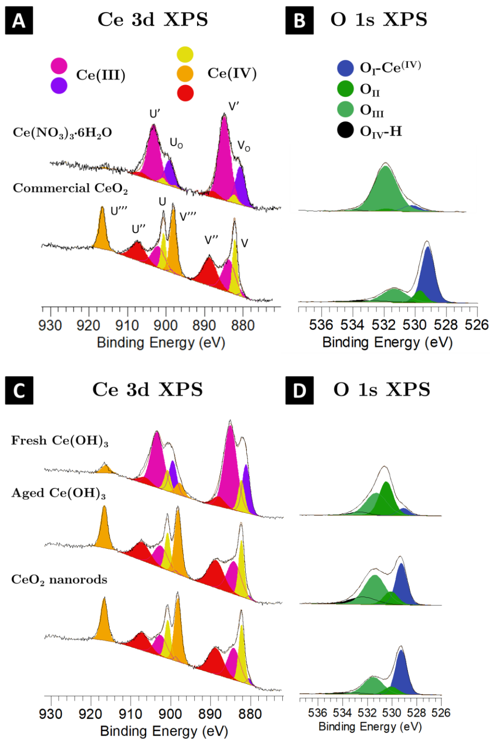
Figure 9. XPS spectra: (A) Ce 3d region and (B) O 1s region of Ce(NO 3 ) 3 · 6H 2 O and commercial cerium oxide with deconvolution of Ce (III) and Ce (IV) peaks and of different oxygen peaks. (C) Ce 3d region and (D) O 1s region of fresh Ce(OH) 3 , aged Ce(OH) 3 (Synthesis IV.2.) and CeO 2 nanorods (Synthesis IV.1.)
